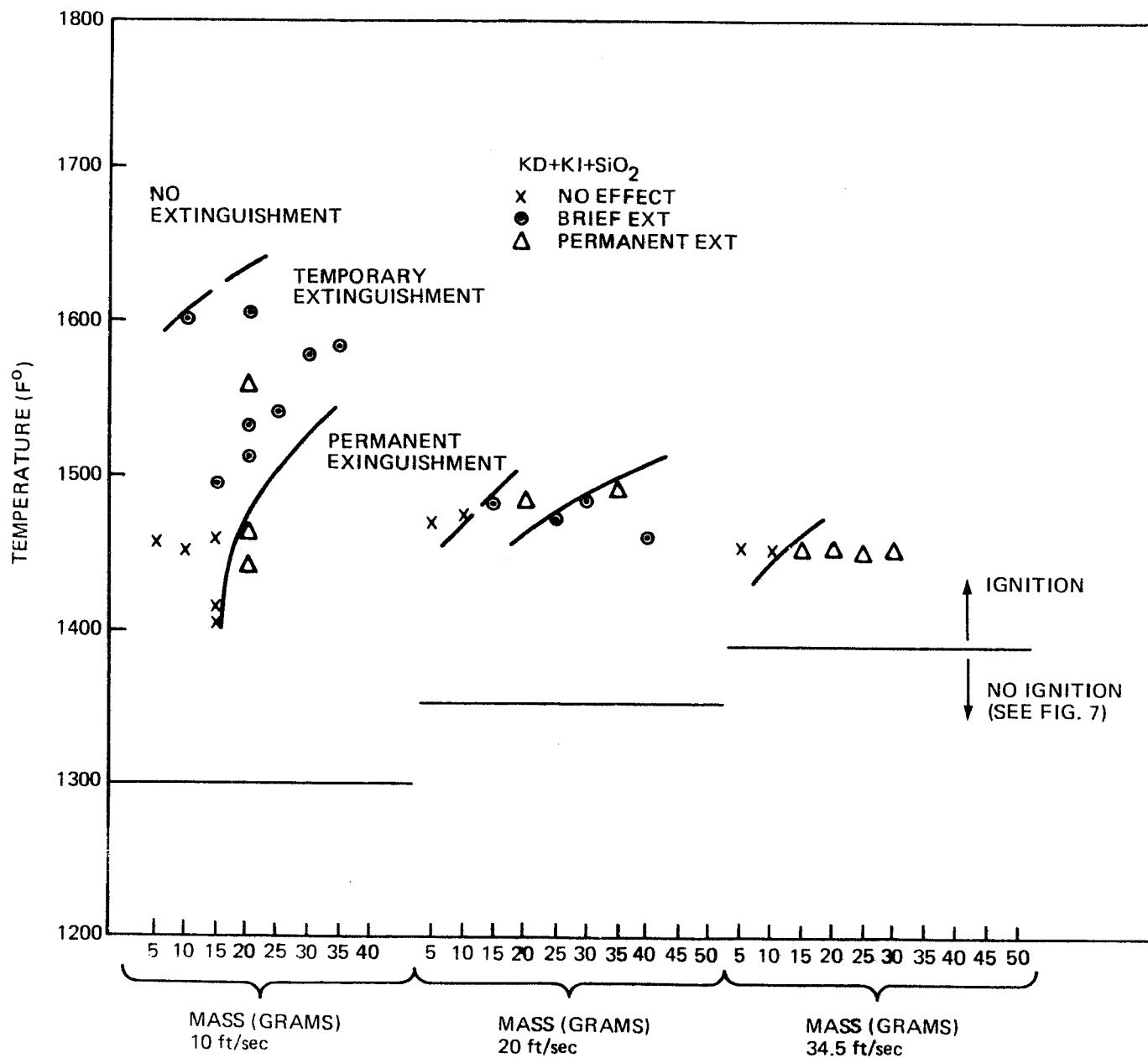
Figure 9. KD+KI+SiO 2 Test Data (Grams Versus Surface Temperature)
