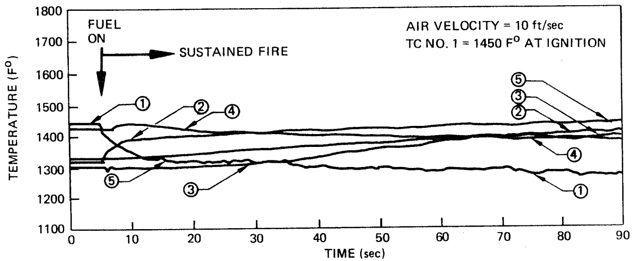
a. AFTER IGNITION
