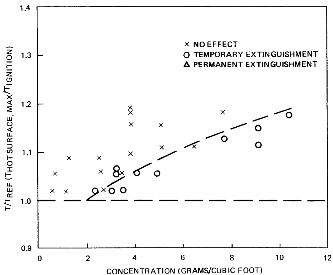
Figure 11. NaD+SiO_2 Test Data ( T/T_{ref} versus Concentration)
