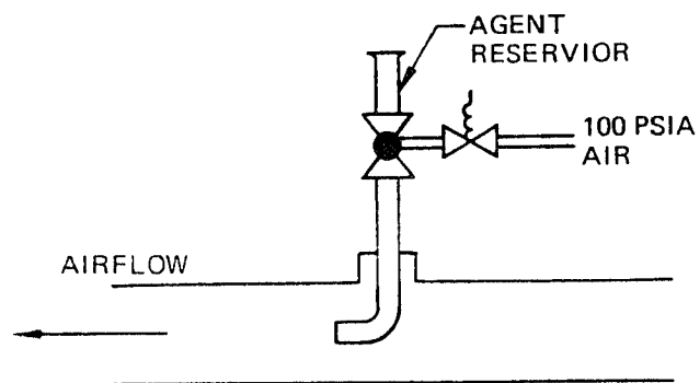
b. MODIFIED DESIGN
