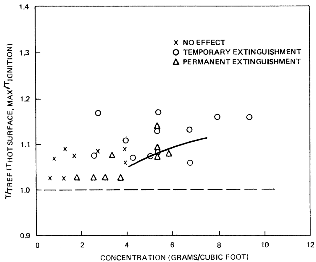
Figure 12. KD+KI+SiO_2 Test Data ( T/T_{ref} versus Concentration)
