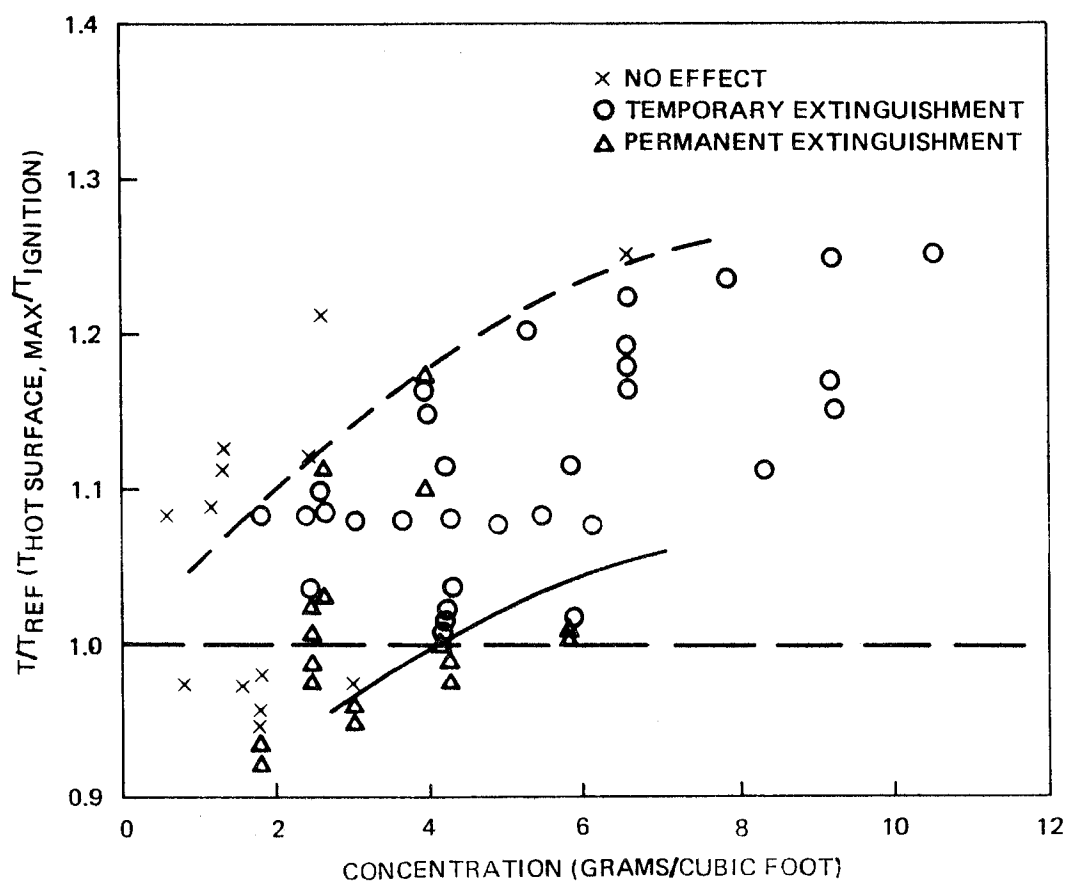
Figure 10. MONNEX Test Data (T/T ref versus Concentration)
