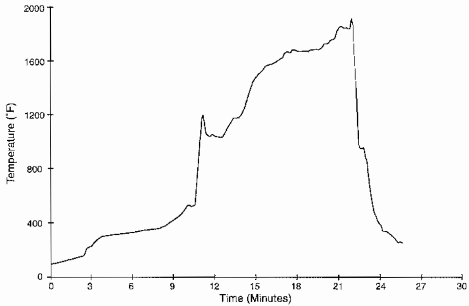
FIGURE 12. TEST RESULTS AFTER SIX GENERATORS WERE PACKED IN TUBES AND PACKED IN A BOX AND THE BOX PLACED ON ITS SIDE
