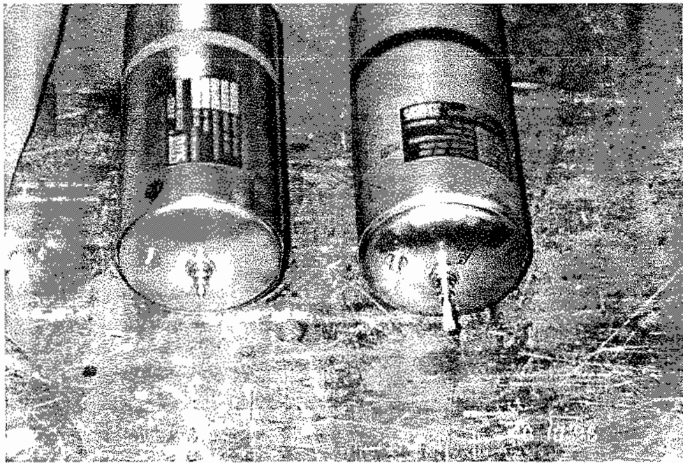
FIGURE 5. GENERATORS OVERPRESSURIZED AFTER PLUGGING THE OUTLETS AND ACTIVATED
