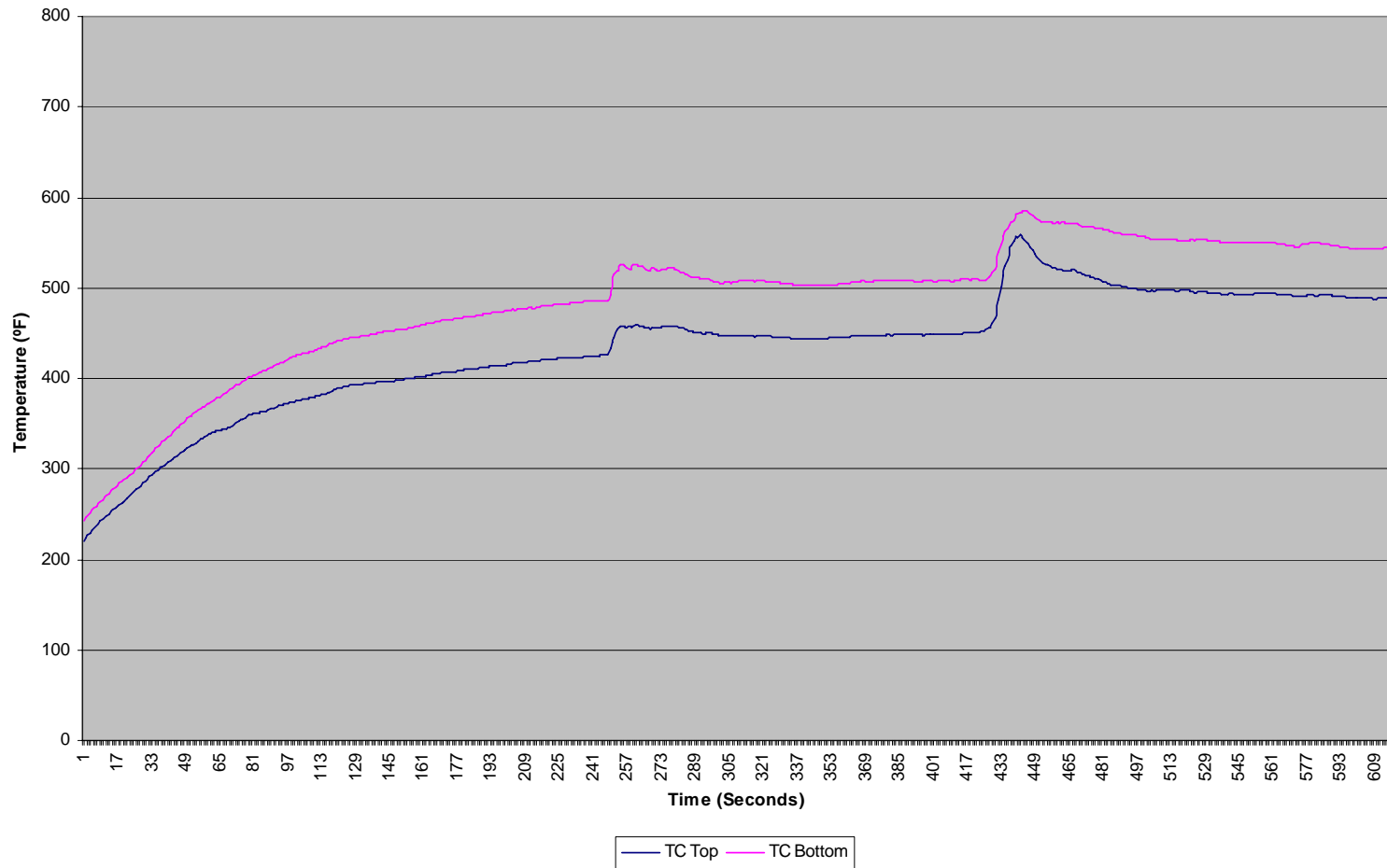
Test 86: Sanyo High Capacity, 50% Charge, Oven/Box Test
