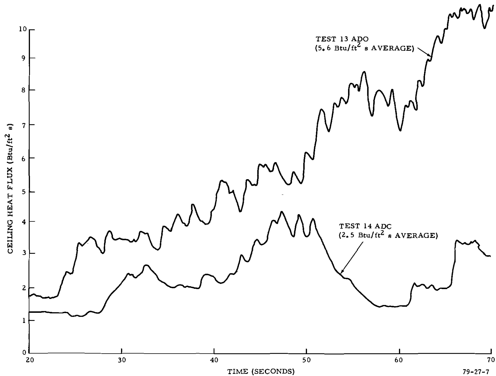
FIGURE 7. CEILING HEAT FLUX UNDER CALM WIND CONDITIONS--TESTS 13 AND 14
