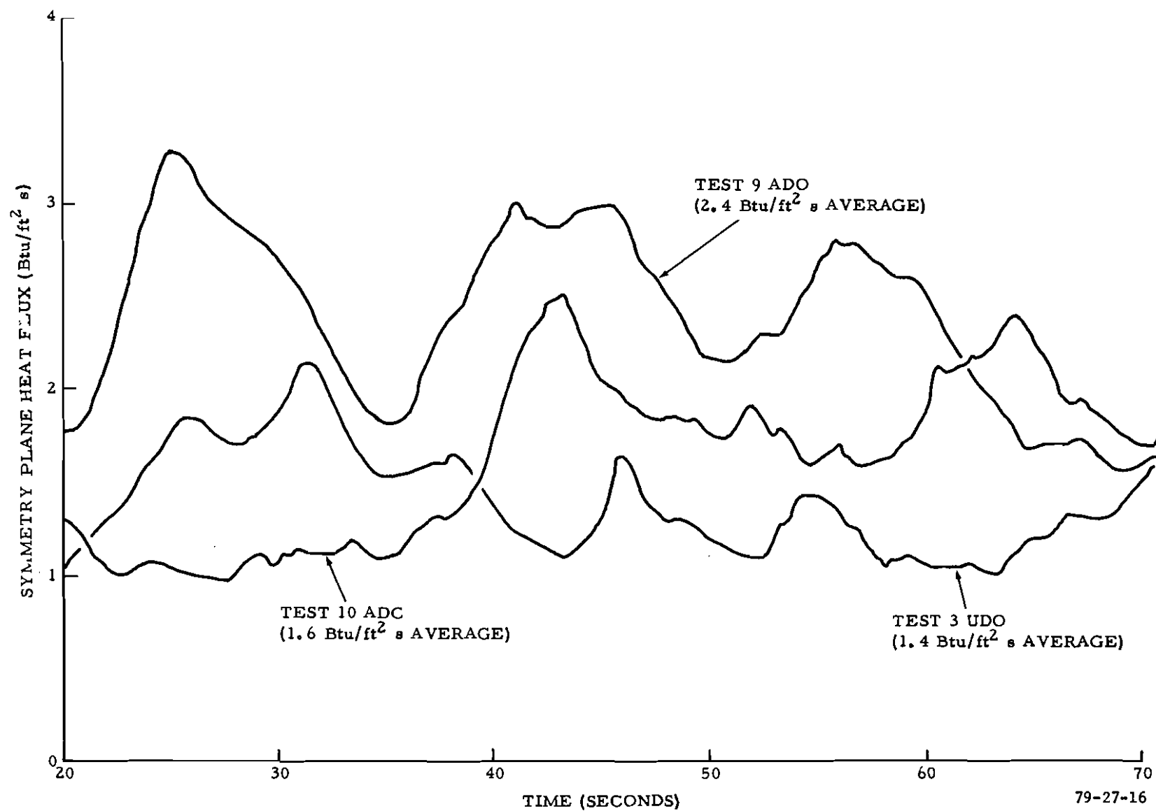
FIGURE 16. SYMMETRY PLANE HEAT FLUX WITH WIND PERPENDICULAR TO FUSELAGE--TESTS 3, 9, AND 10
