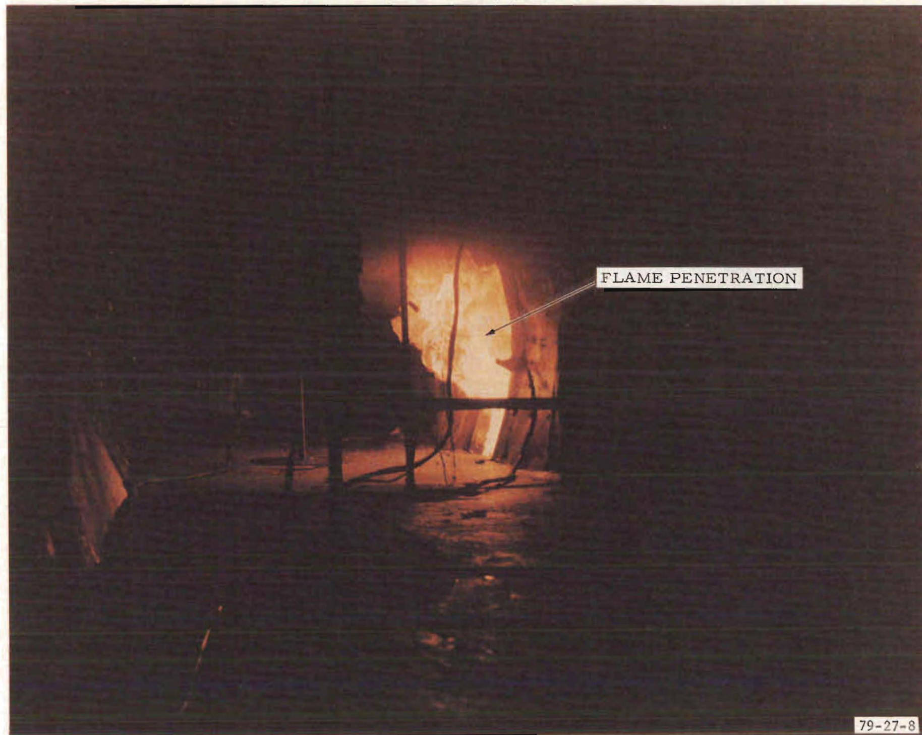
FIGURE 8. FLAME PENETRATION--TEST 13
