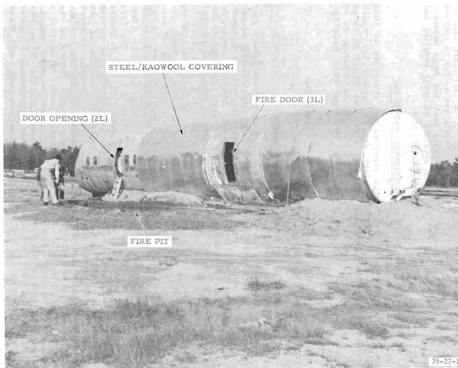
FIGURE 1. FIRE-HARDENED FUSELAGE
