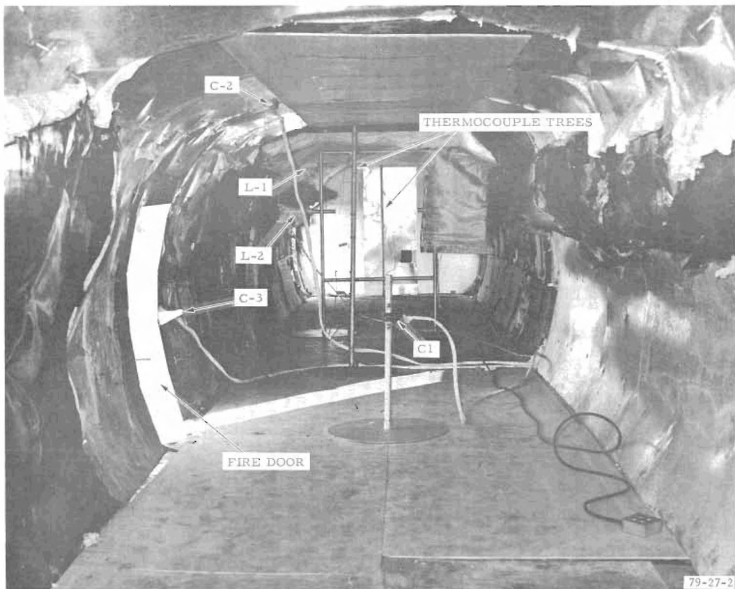
FIGURE 2. FORWARD VIEW OF DC7 INTERIOR
