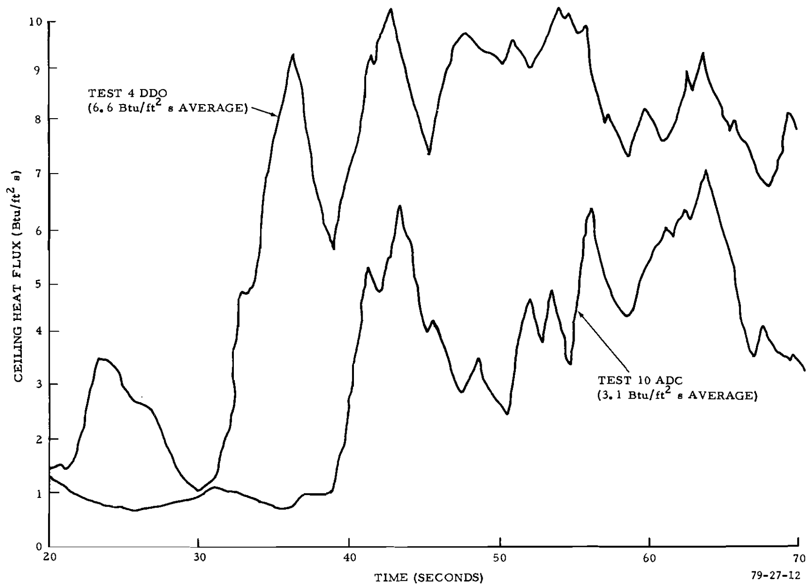
FIGURE 12. CEILING HEAT FLUX WITH WIND PERPENDICULAR TO FUSELAGE--TESTS 4 AND 10
