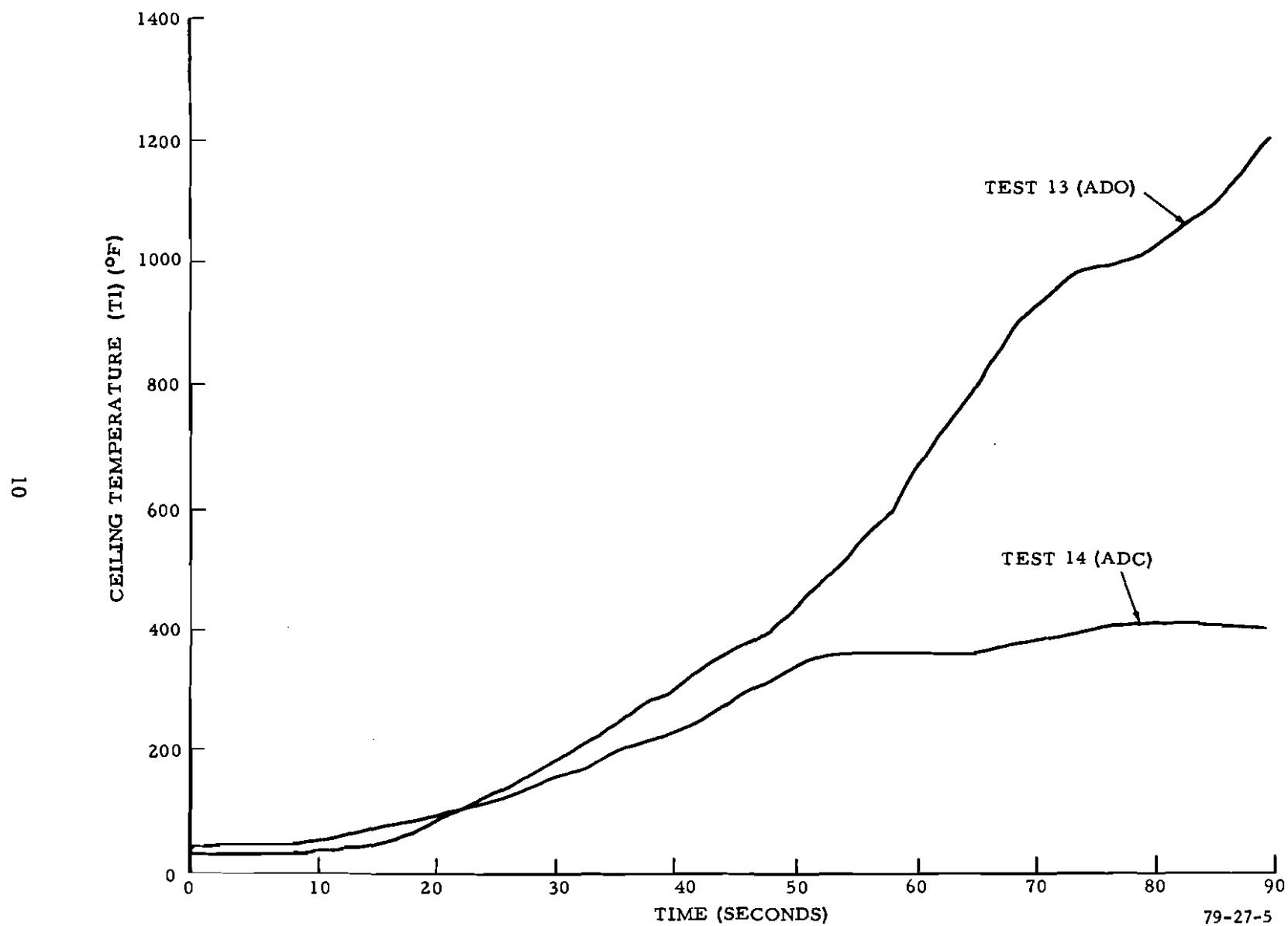
FIGURE 5. CEILING TEMPERATURE HISTORY UNDER CALM WIND CONDITIONS--TESTS 13 AND 14
