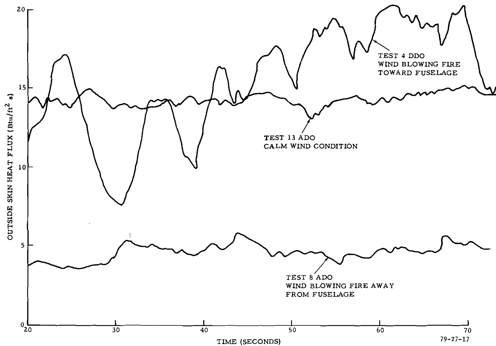
FIGURE 17. EXTERNAL SKIN HEAT FLUX--TESTS 4, 8, and 13
