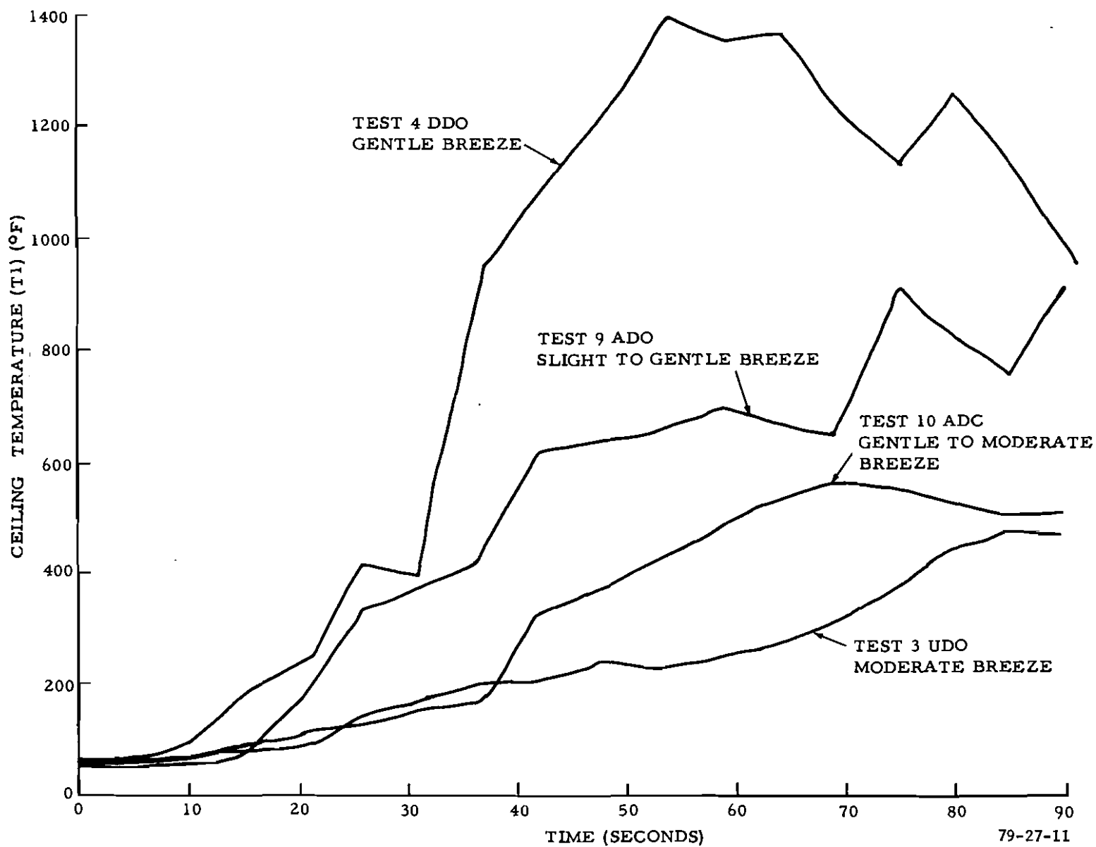
FIGURE 11. CEILING TEMPERATURE HISTORY WITH WIND PERPENDICULAR TO FUSELAGE--TESTS 3, 4, 9, AND 10
