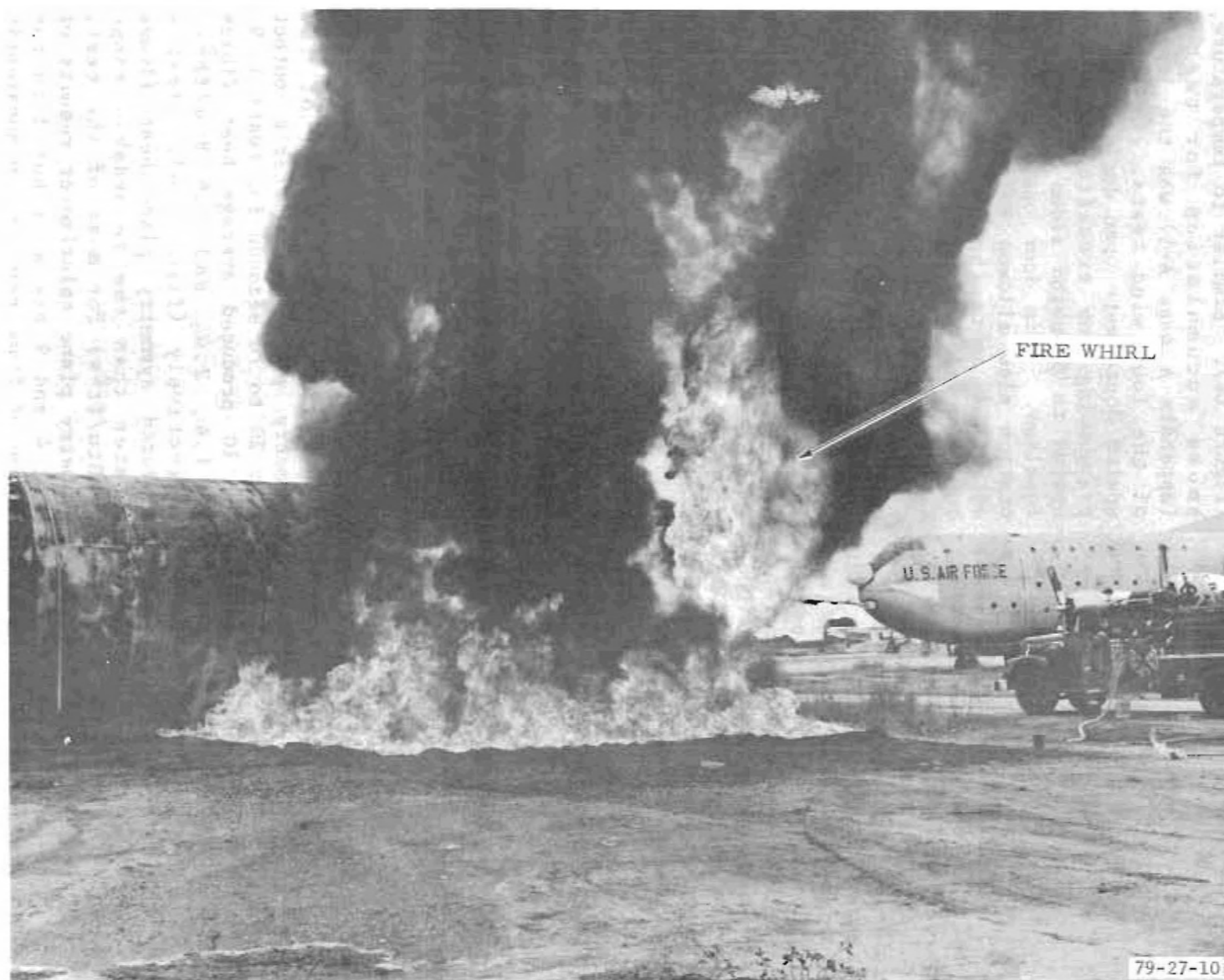
FIGURE 10. FIRE WHIRL--TEST 14
