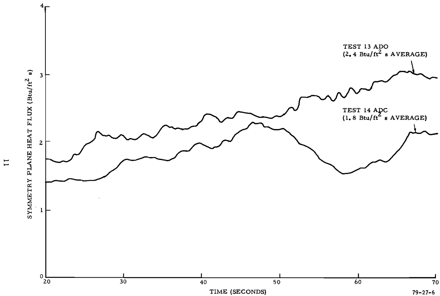
FIGURE 6. SYMMETRY PLANE HEAT FLUX UNDER CALM WIND CONDITIONS--TESTS 13 AND 14
