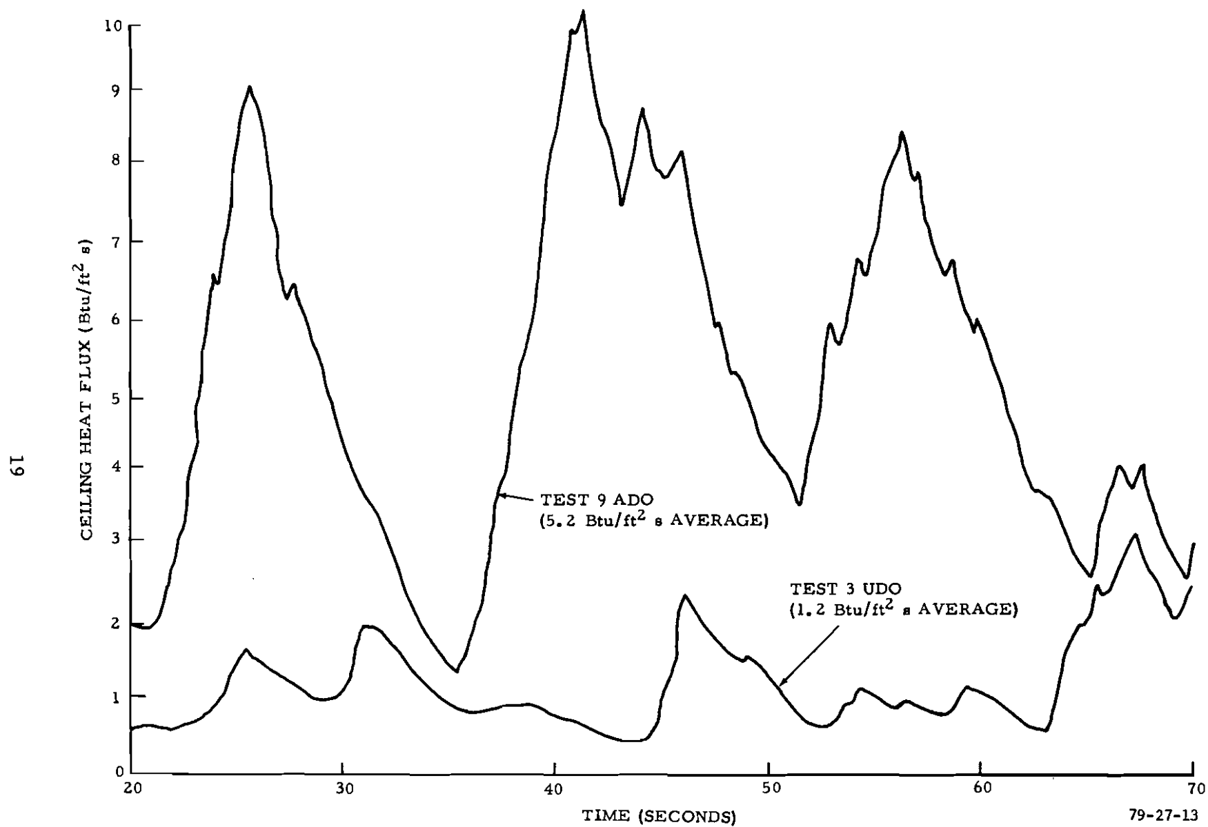
FIGURE 13. CEILING HEAT FLUX WITH WIND PERPENDICULAR TO FUSELAGE—TESTS 3 AND 9
