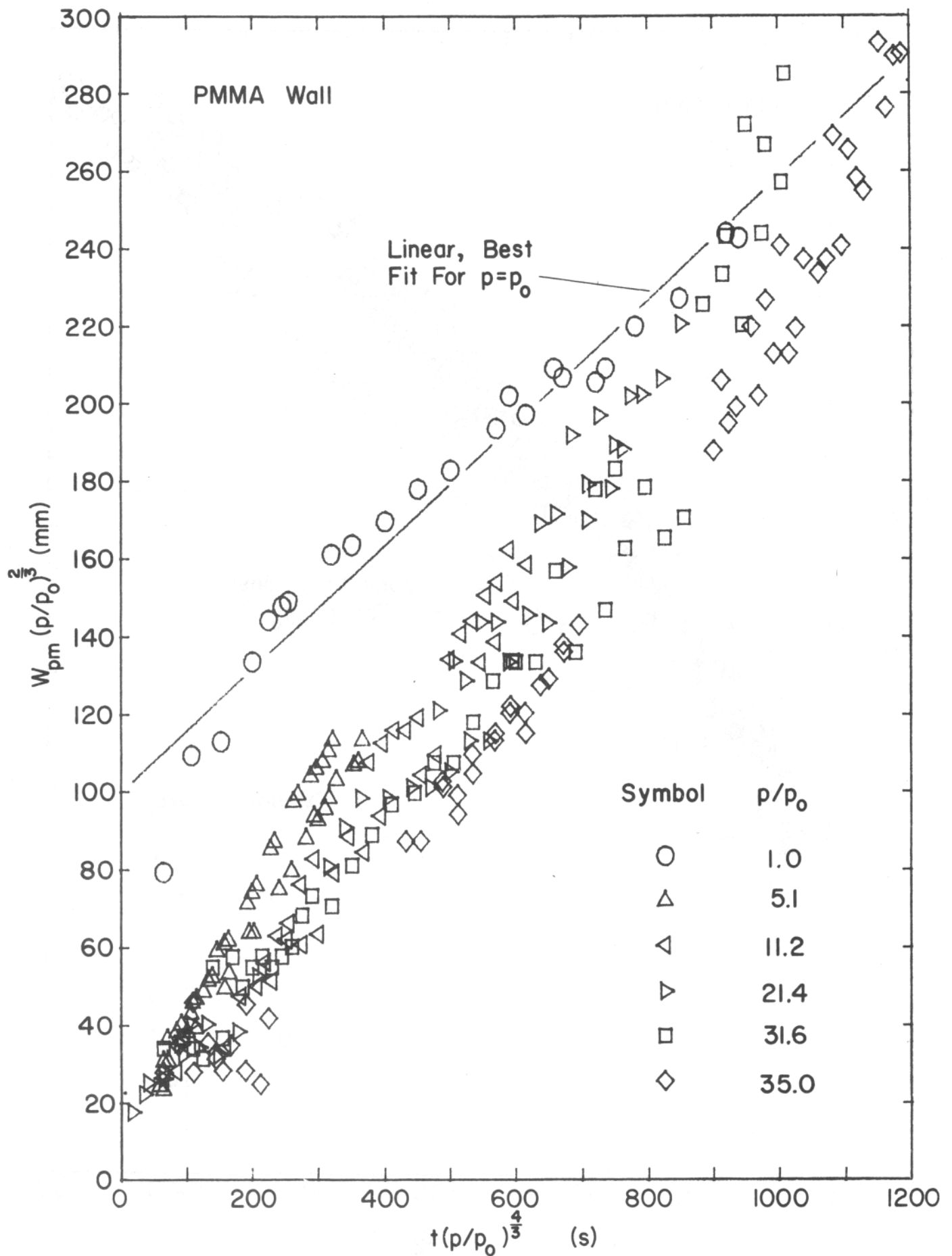
Figure 15: Correlation of Maximum Width of Pyrolysis Zone
