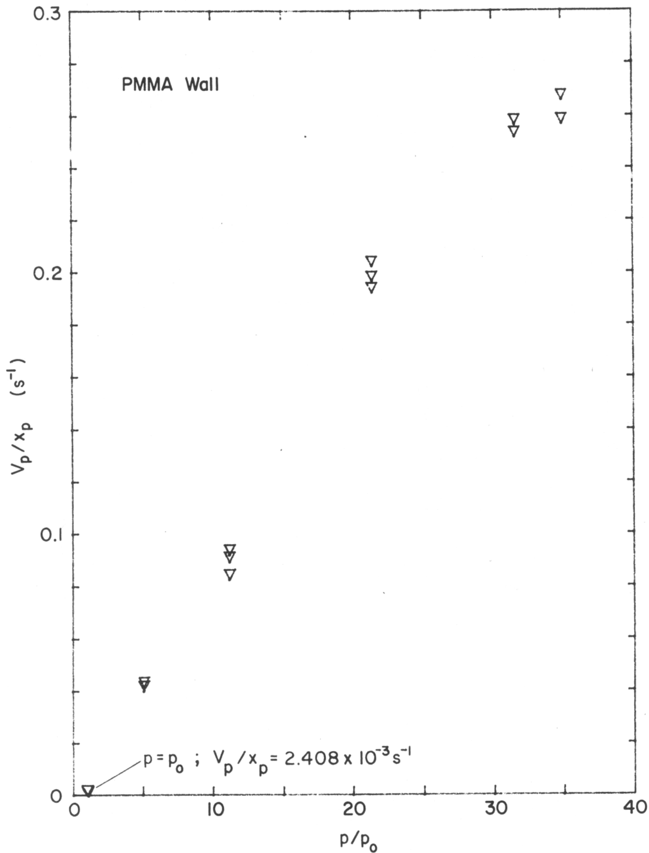
Figure 7: Exponential Growth Factor for Pyrolysis Zone Height
