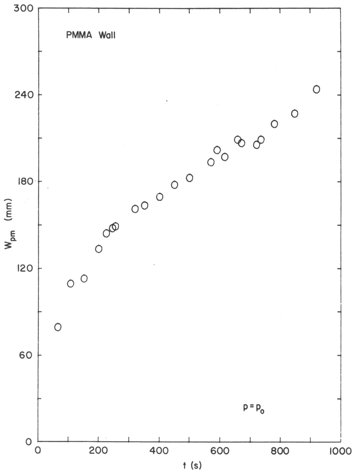
Figure 10: Maximum Width of Pyrolysis Zone for Prototype
