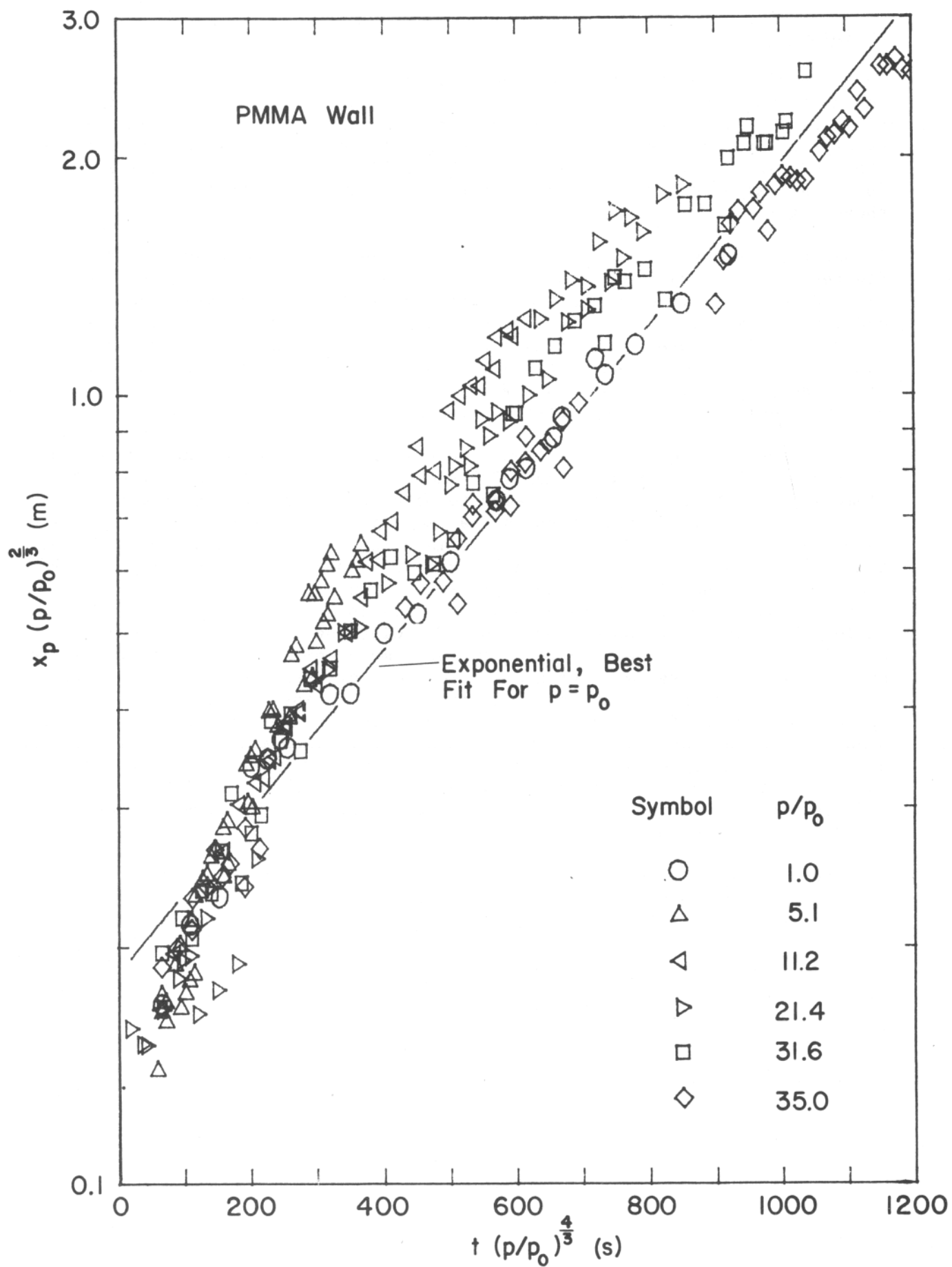
Figure 13: Correlation of Pyrolysis Zone Height
