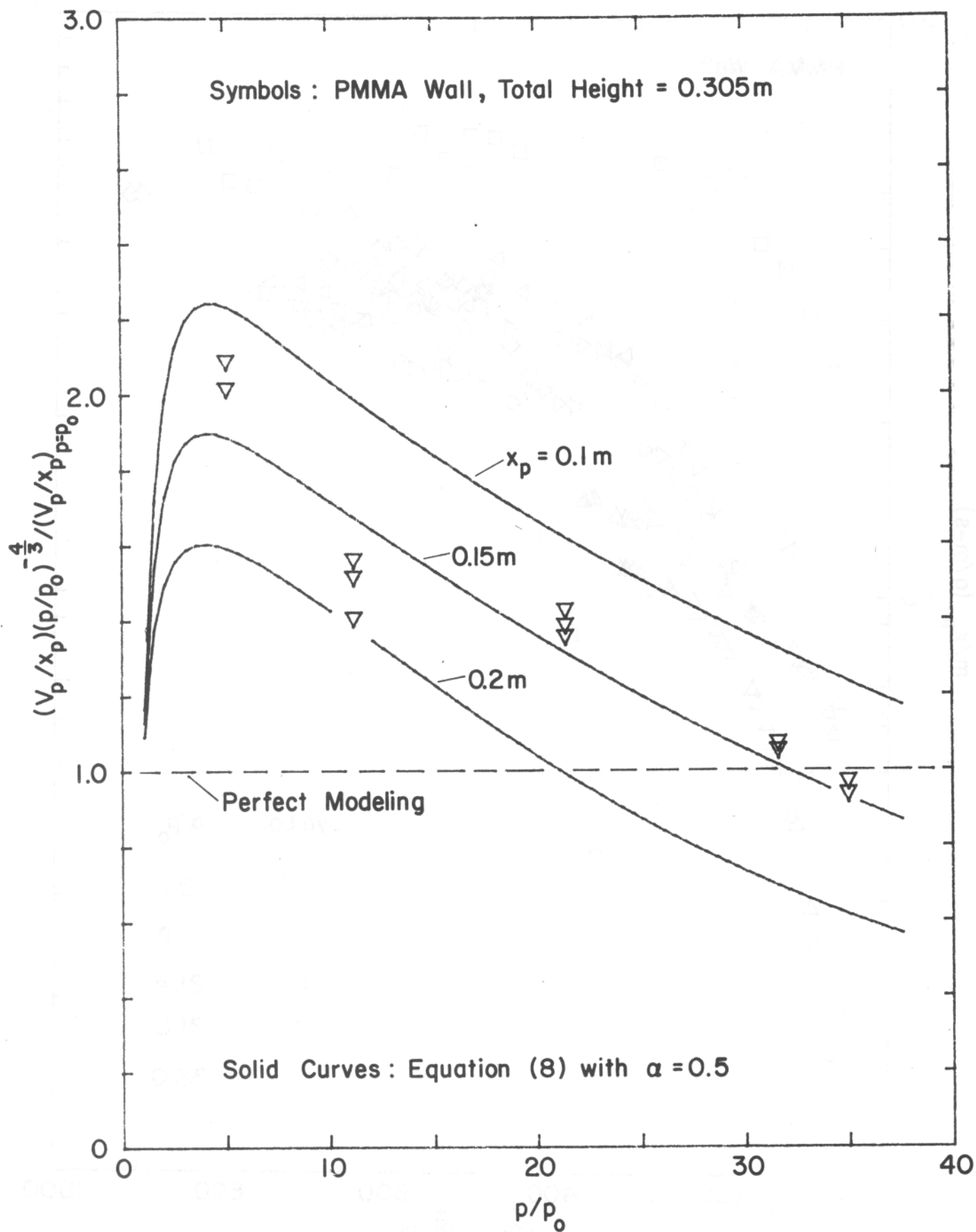
Figure 18: Exponential Growth Factor for Thermally Thick PMMA
