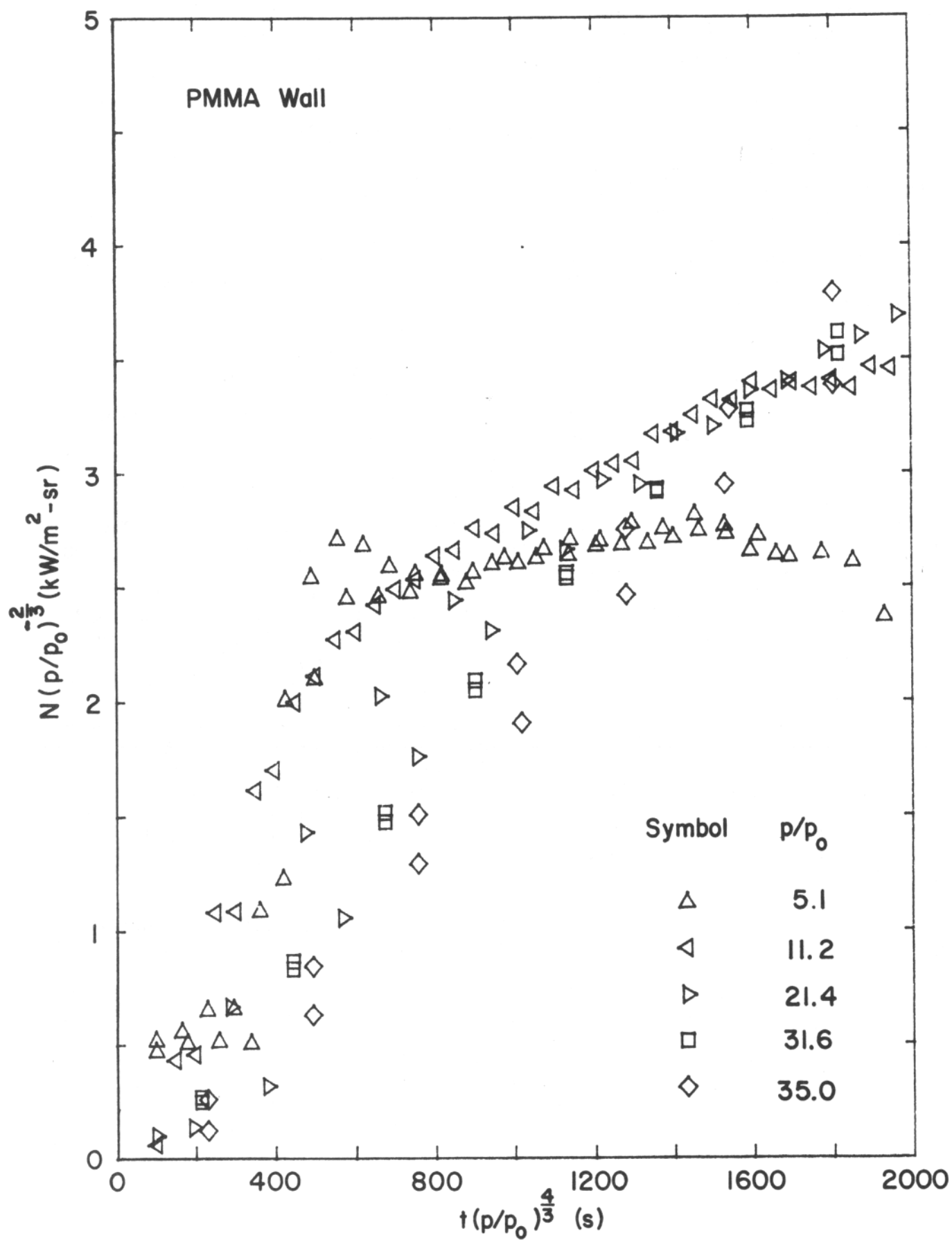
Figure 16: Correlation of Radiance Measurements for Model
