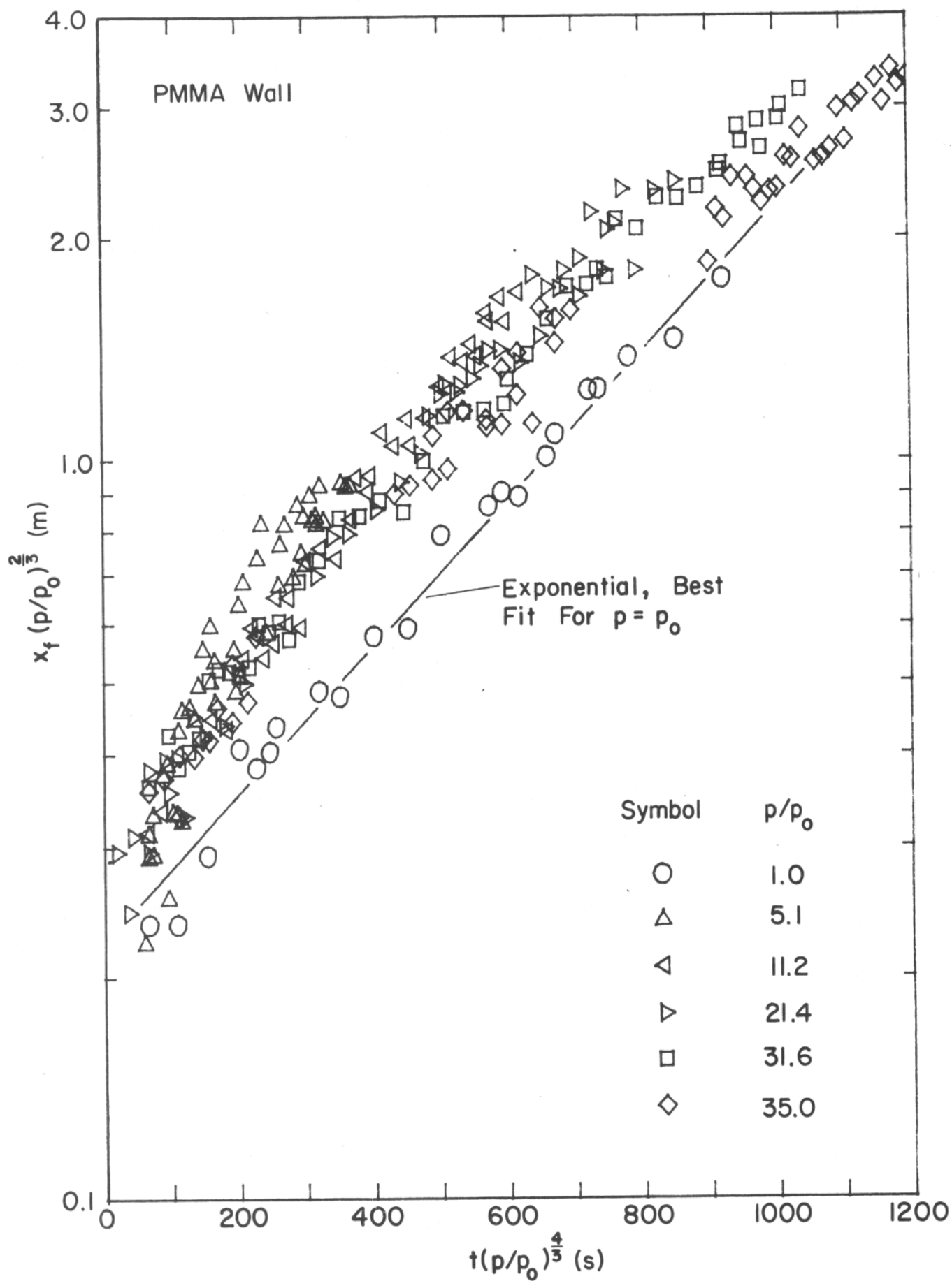
Figure 14: Correlation of Flame Height
