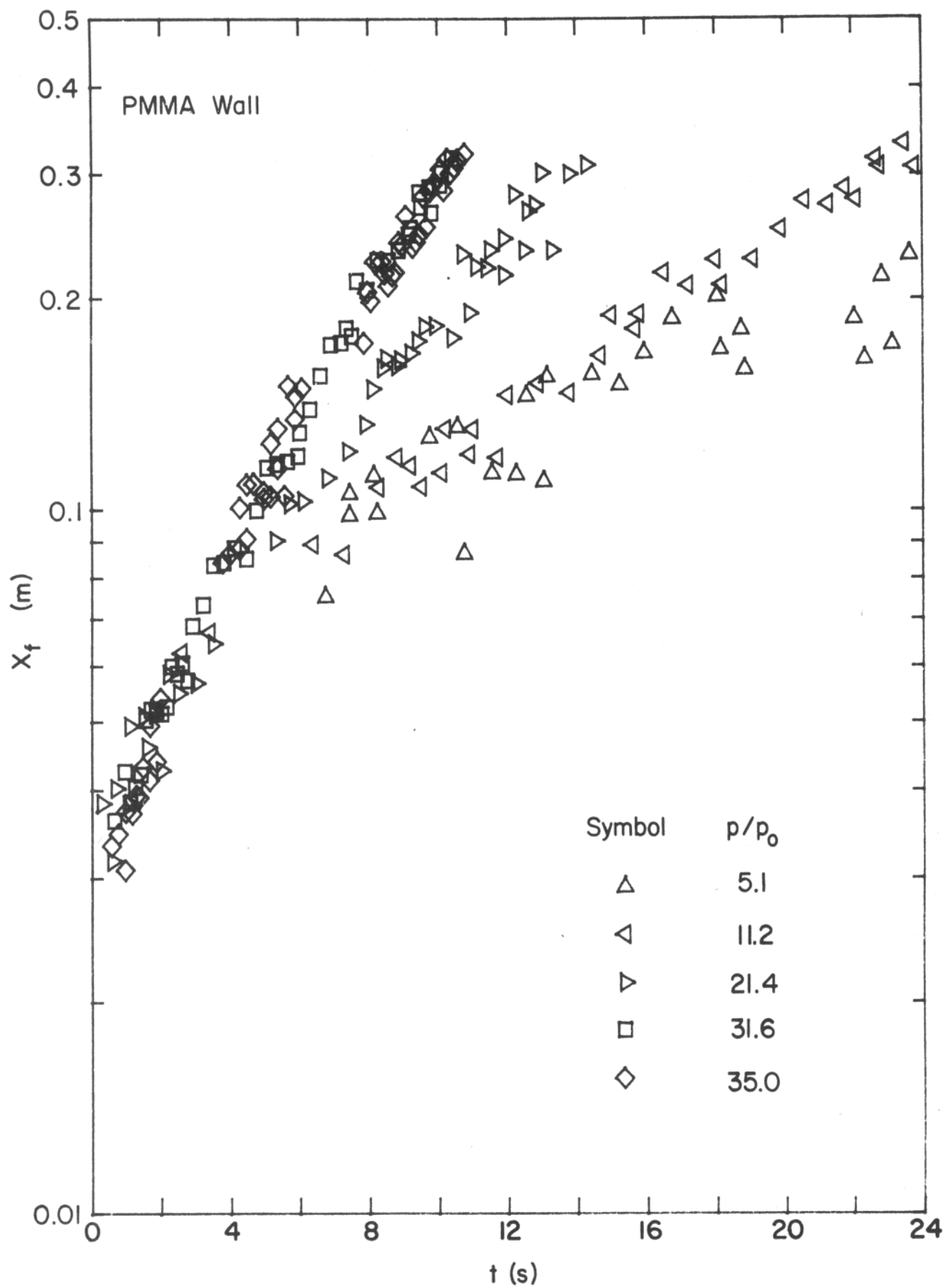
Figure 5: Flame Height for Model
