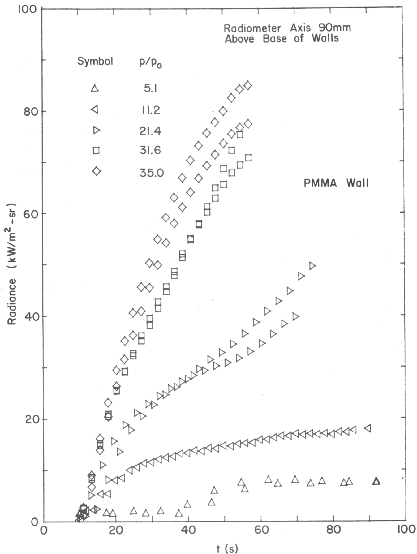
Figure 11: Flame and Fuel Radiance for Model
