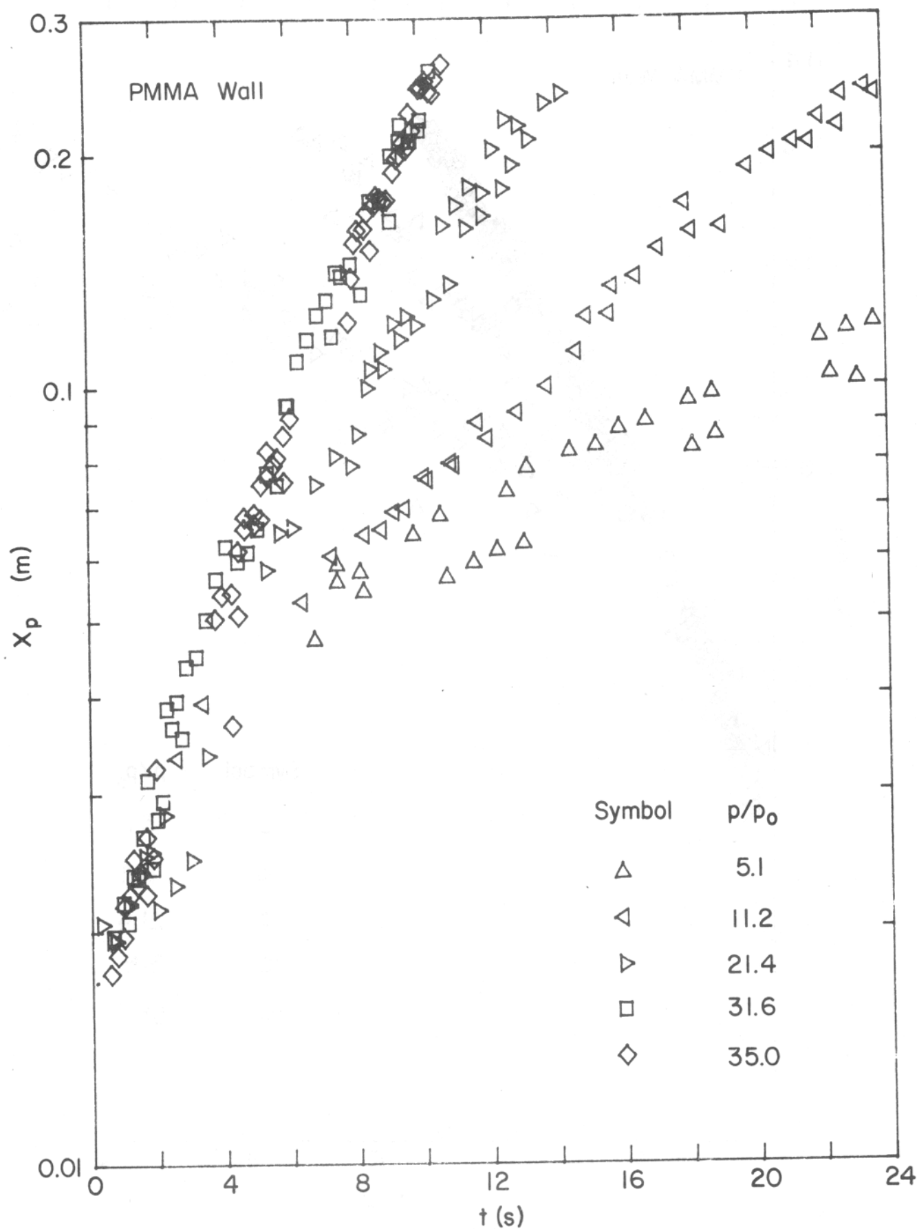
Figure 4: Pyrolysis Zone Height for Model
