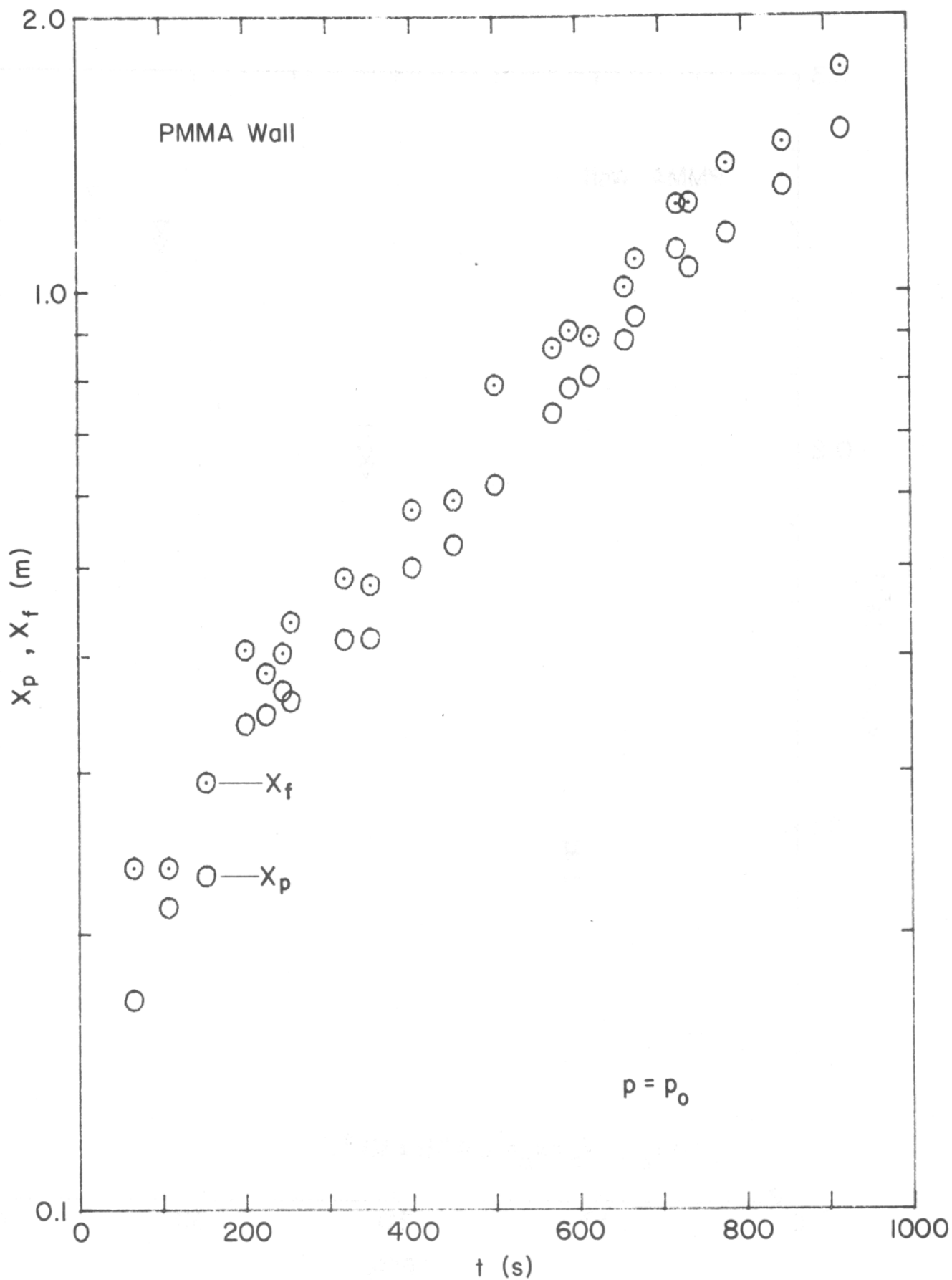
Figure 6: Flame and Pyrolysis Height for Prototype
