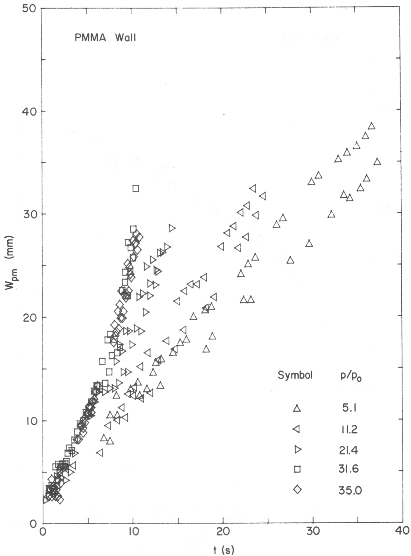
Figure 9: Maximum Width of Pyrolysis Zone for Models
