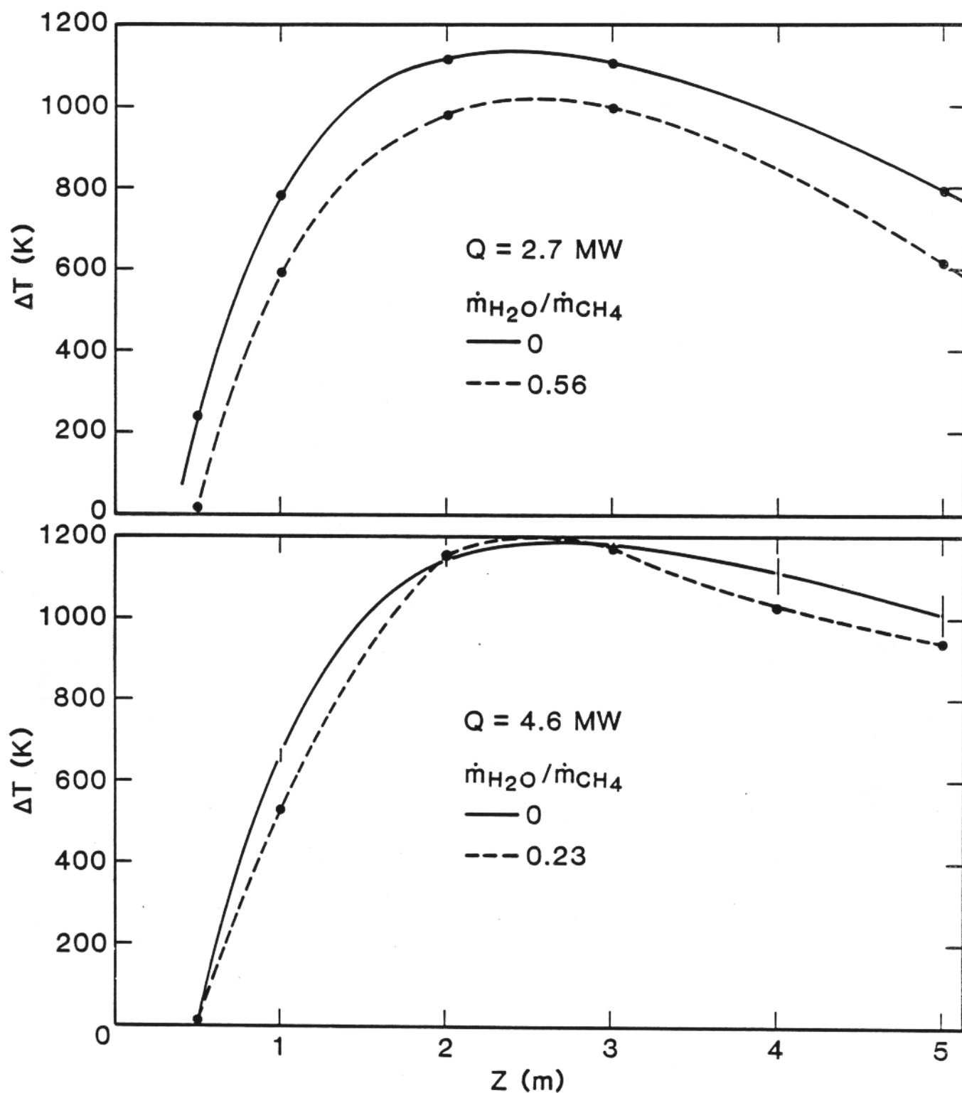
Figure 13. Centerline temperature rise vs height with and without water spray ( Q = 2.7 and 4.6 MW)
