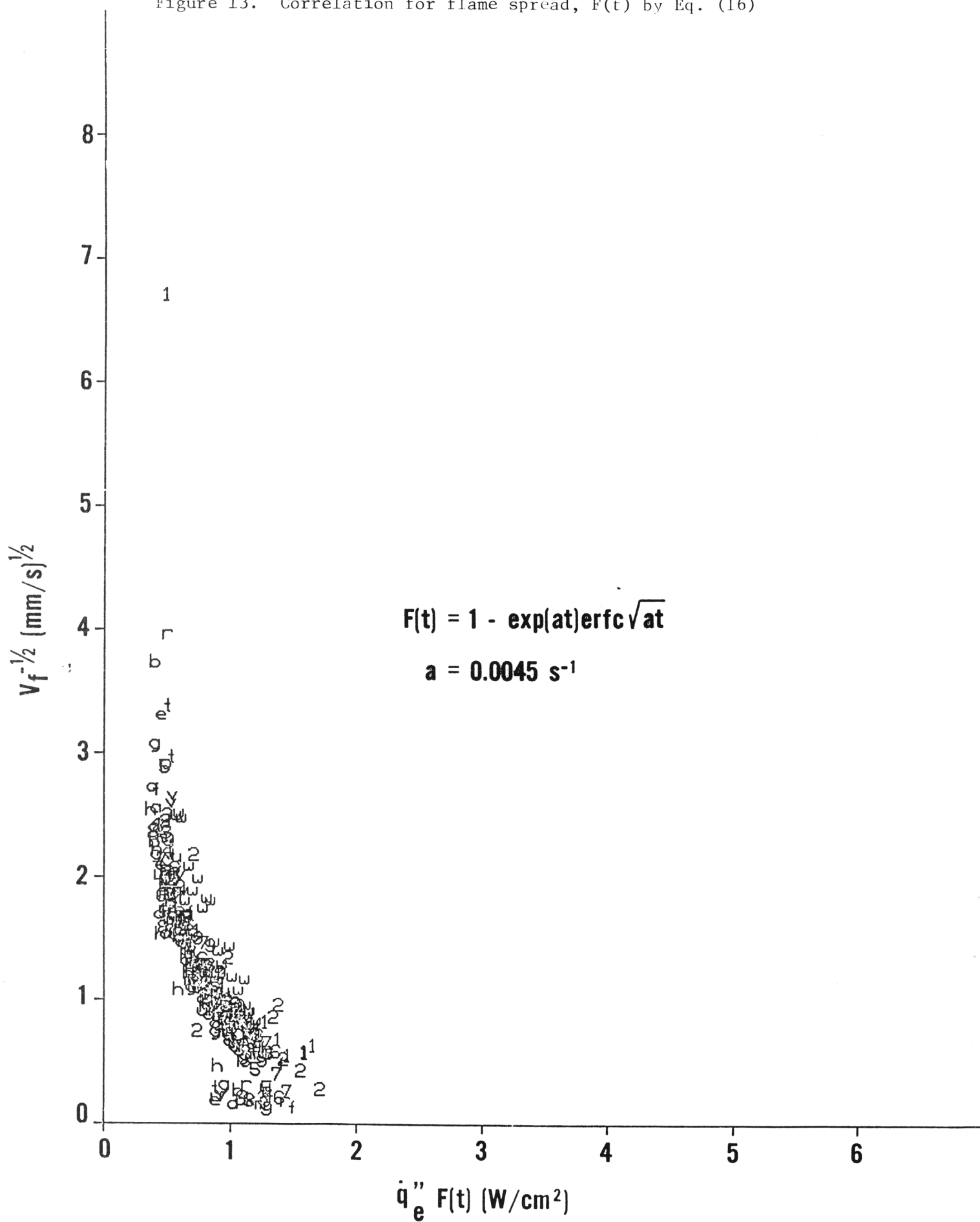
Figure 13. Correlation for flame spread, F(t) by Eq. (16)
