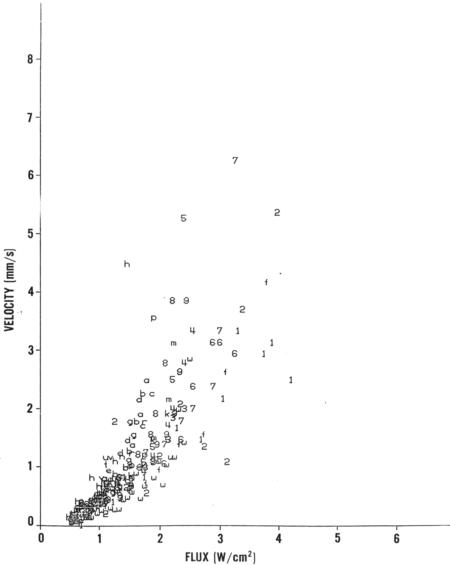
Figure 10. Flame spread velocity for particle board tests
