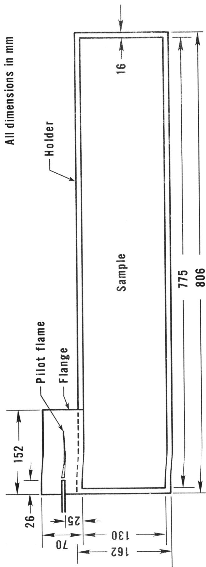
Figure 6. Pilot flame configuration
