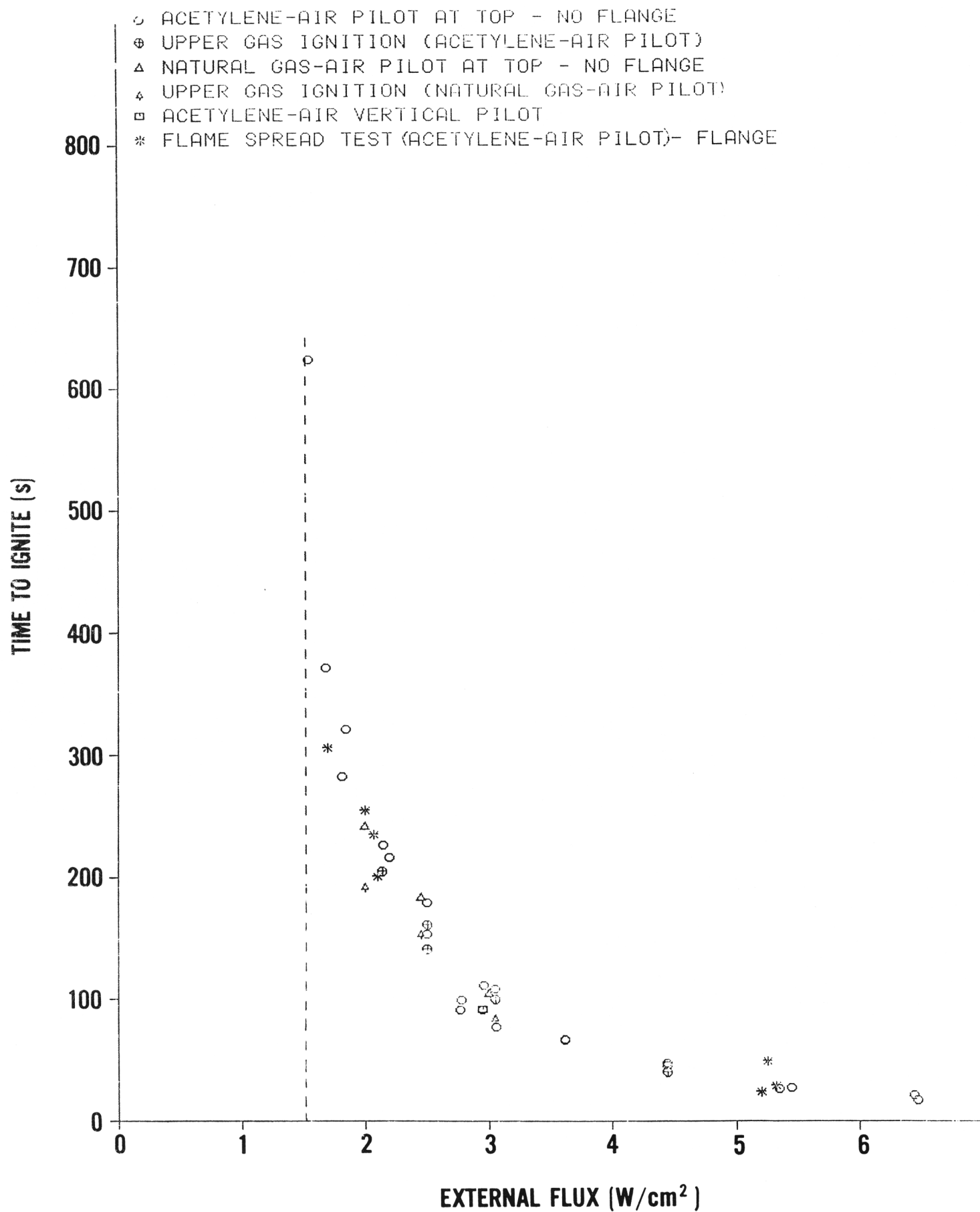
Figure 7. Time to ignite for particle board
