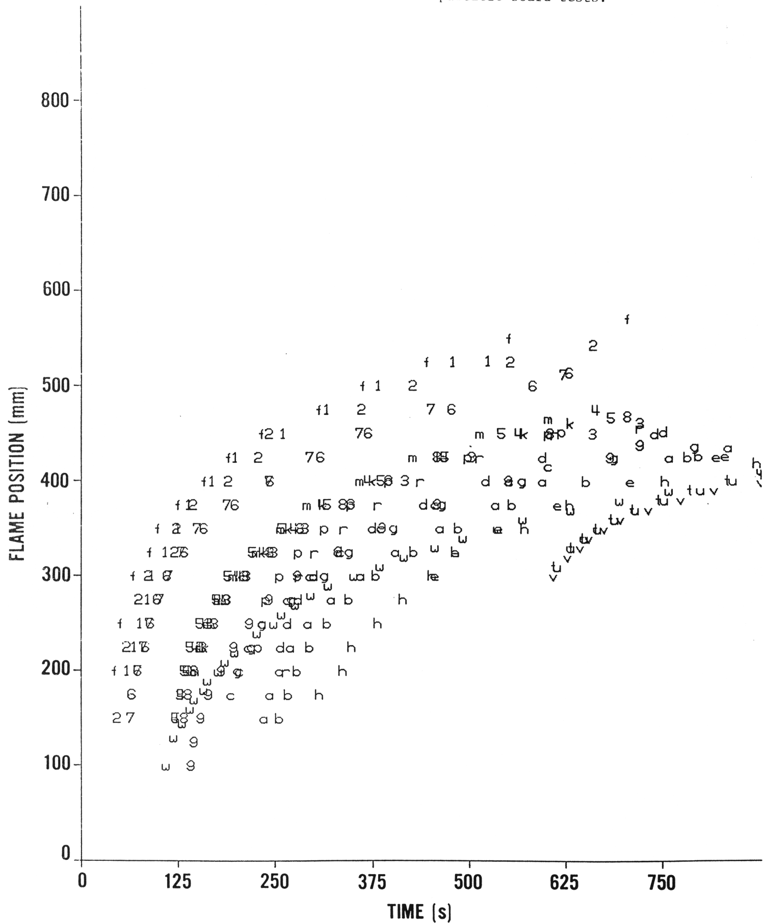
Figure 9. Flame front movement for particle board tests.
