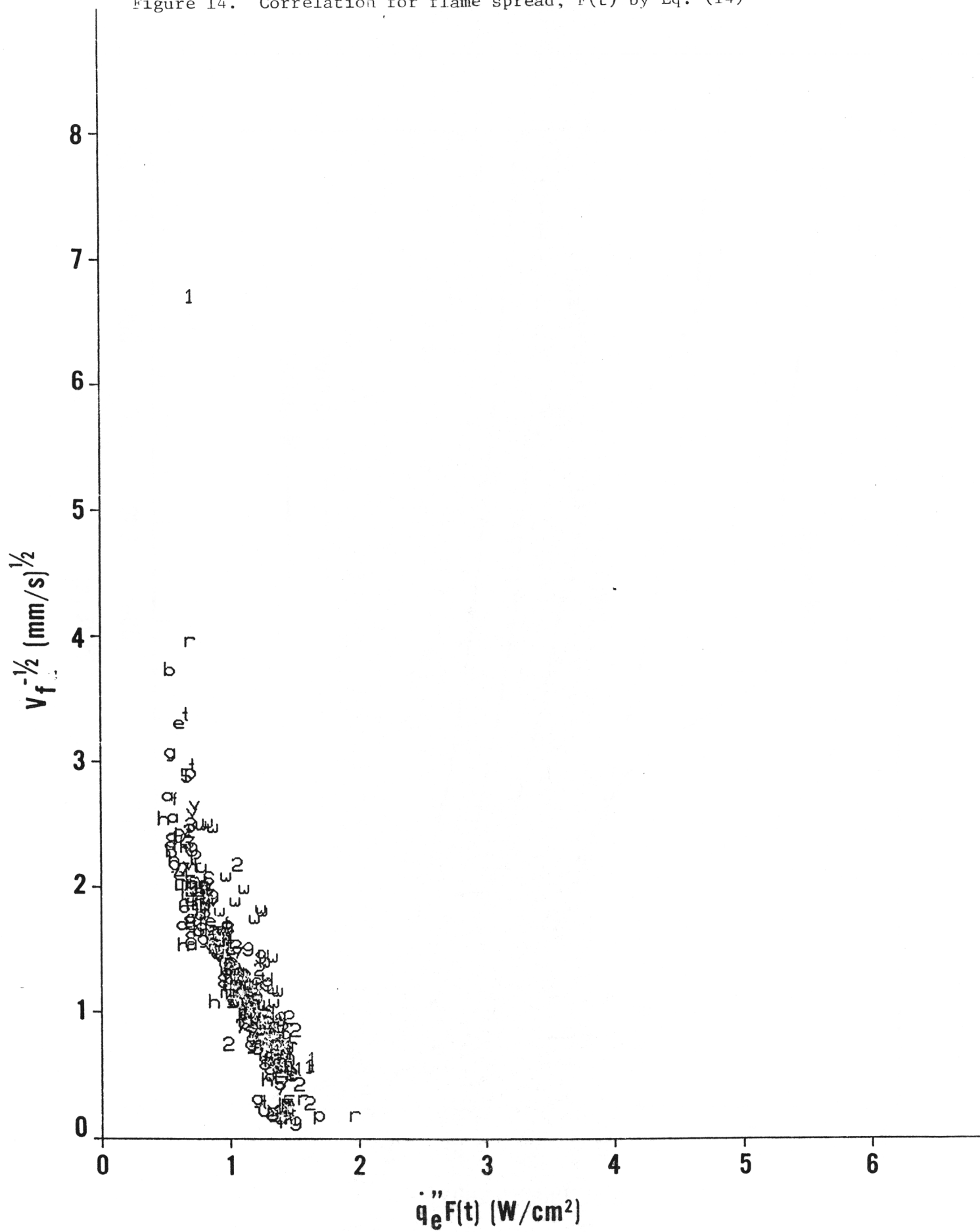
Figure 14. Correlation for flame spread, F(t) by Eq. (14)
