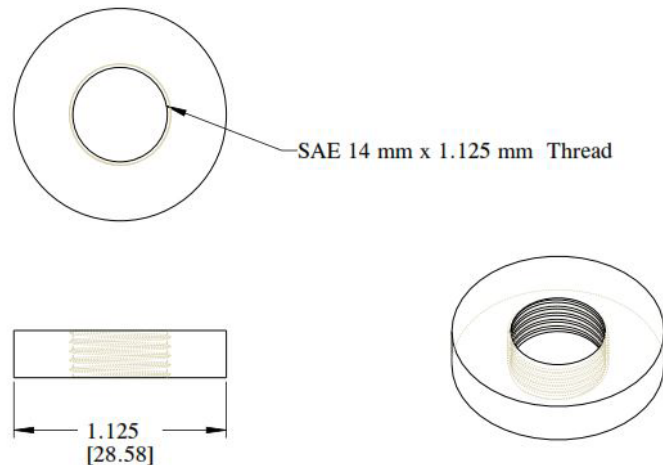
Figure 7-S-26. Threaded Boss
