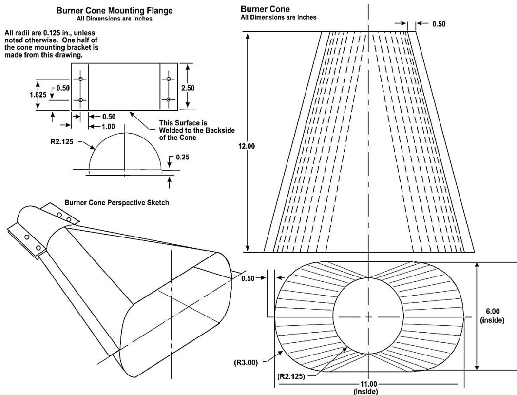
Figure 7-S-25a. Burner Cone Details
