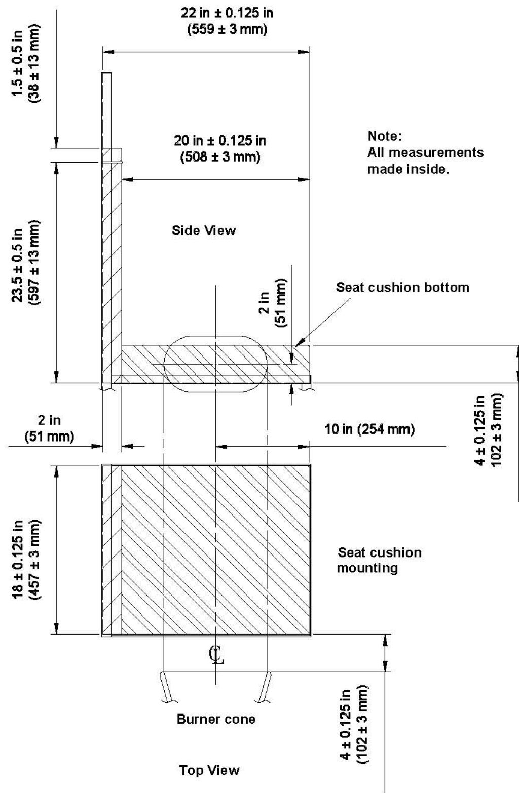
Figure 7-2. Top and Side View of Seat Test Sample in Test Sample Mounting Frame
