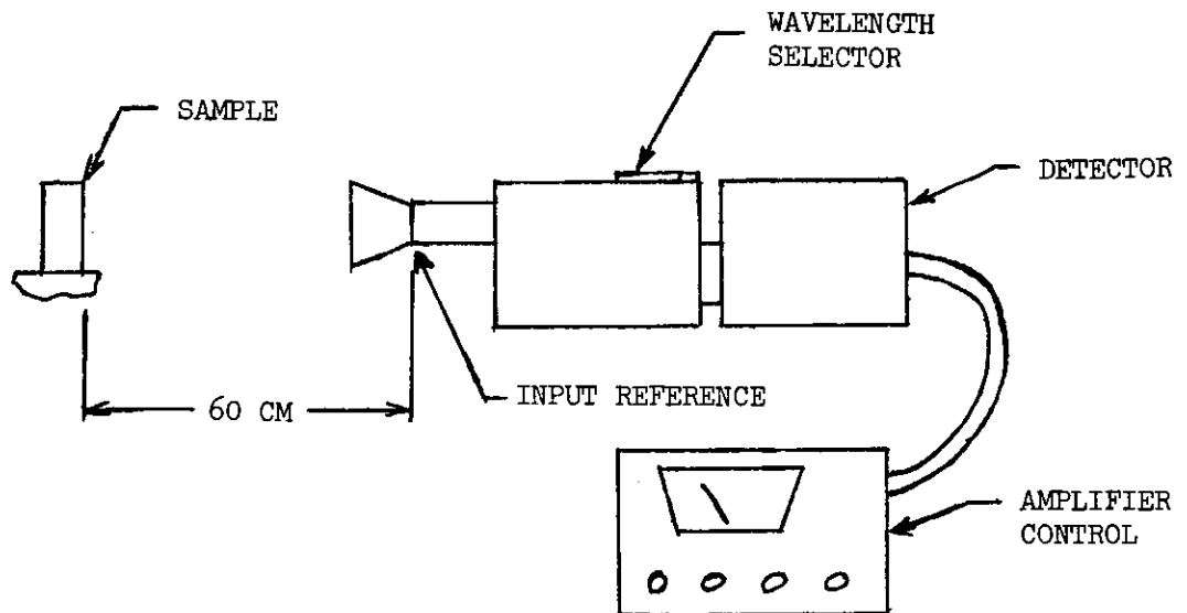
Figure 18. Ultraviolet Measurement Instrumentation
