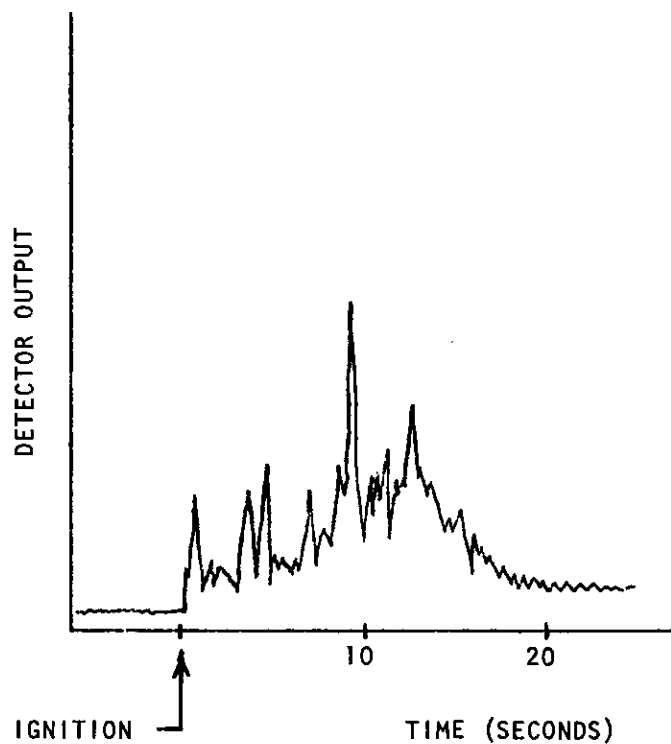
Figure 19. Typical Ultraviolet Emission Measurement
