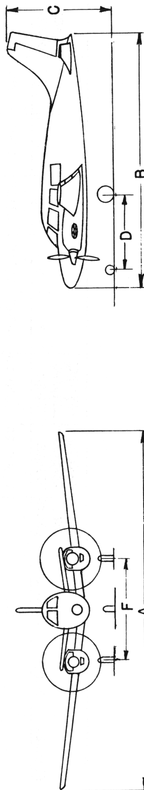
FIGURE 2-4. TWIN ENGINE, LOW OR MID WING, TRICYCLE GEAR AIRCRAFT 8,000 LB. (3,628 KG.) or less.
