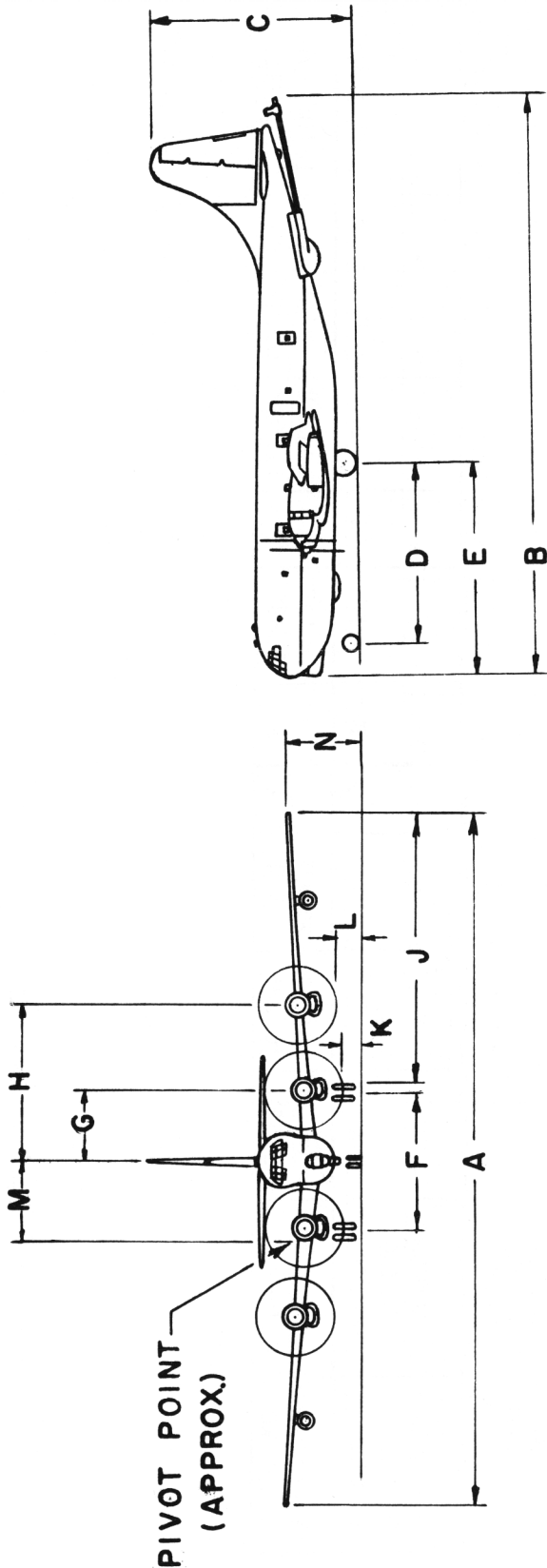
FIGURE 3-2. BOEING KC-97L
