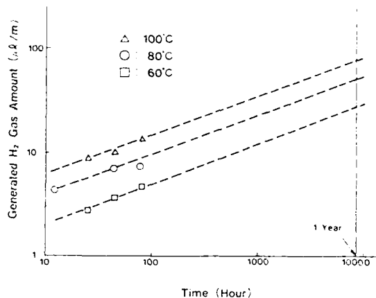
Fig.7 Temperature Dependency of H 2 gas from Optical Fiber Unit
