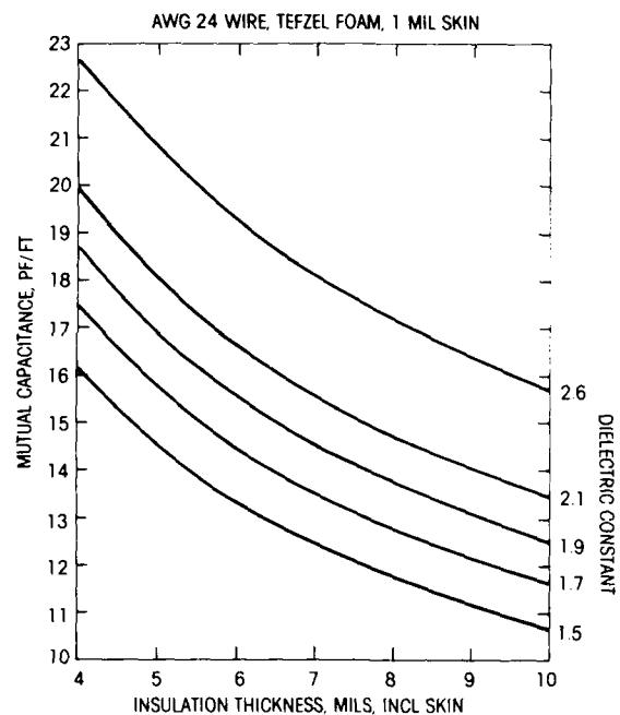
Figure 15 MUTUAL CAPACITANCE
