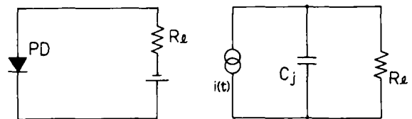
(a) Physical circuit
