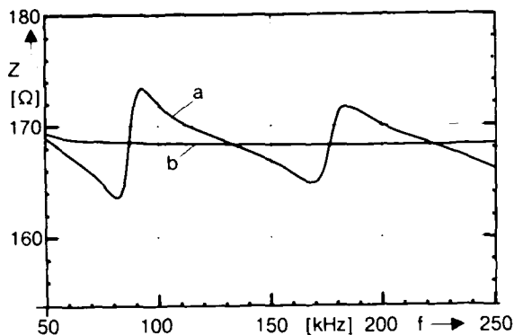
Fig. 5 Calculated characteristic impedance, with (a) and without (b) error current. (Same parameters as Fig. 4).
