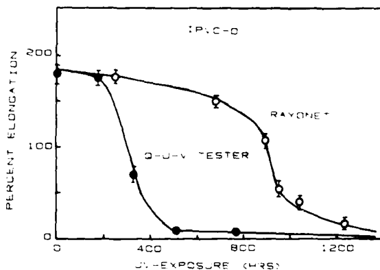
Fig.5 320-380nm DEGRADATION OF BRAND NEW XPVC.
