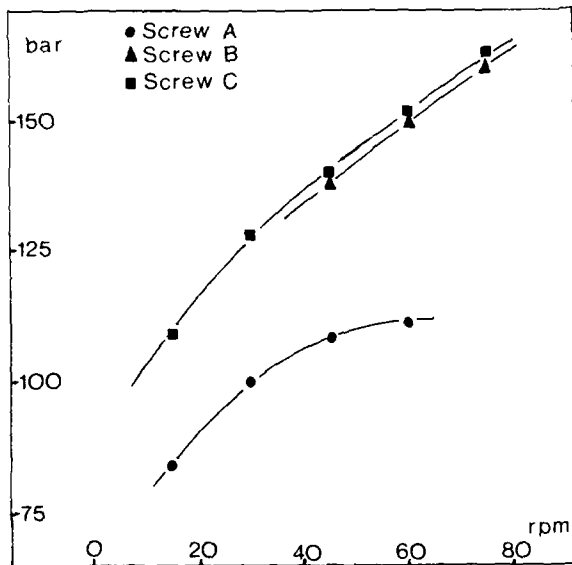
Figure 18. Head Pressure Versus Screw Speed
