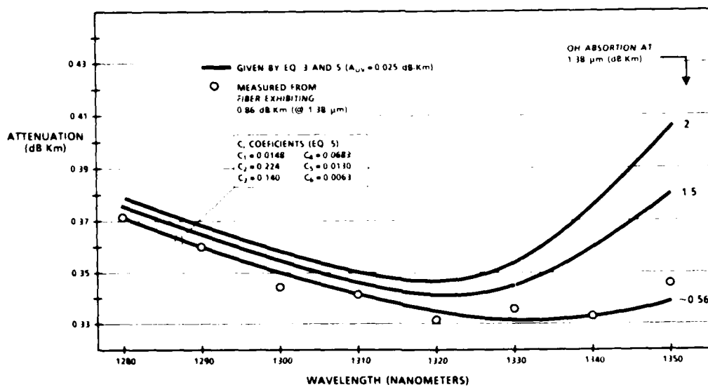
Figure 4 - Spectral attenuation: measured results and fitted curves (given by equations (3) and (5), being A_{OH} = 0.025 \text{ dB/Km} ).
