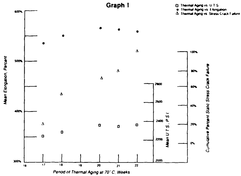
Foam Skin Insulation Static Stress Crack Failure Samples Pre-Conditioning 8 weeks @ 70°C
