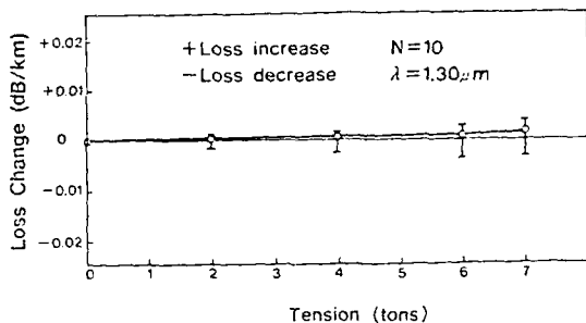
Fig. 5 Tension-Loss Characteristic
