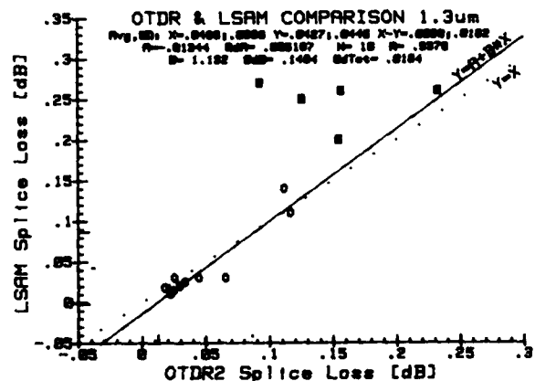
Figure 2. LSAM vs Bi-directional OTDR
