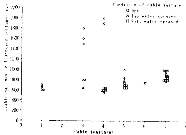
Fig. 8 Relationship between cable length and lightning impulse flashover voltage
