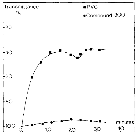
Figure 11. Results From 3 Metre Cube Smoke Test
