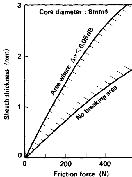
Fig.18 Calculated sheath design parameters in consideration of sheath shrinkage
