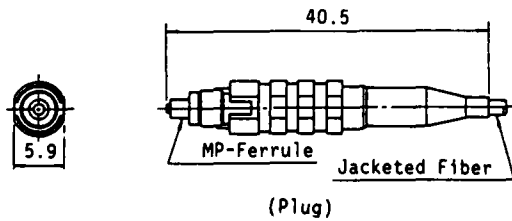
Figure 3 SJ Connector with MP-Ferrule
