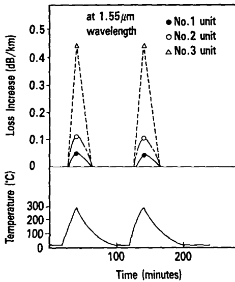
Figure 6 Transmission Loss Change of Six-Fiber Unit as a Result of Heat Shock ( L=500\text{m} )
