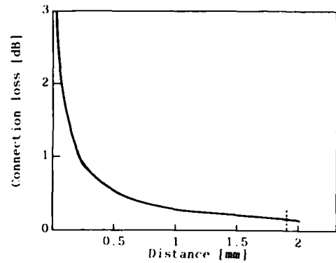
Fig. 6 Connection loss when a bonding wire located at the center of spot (NA 0.25)
