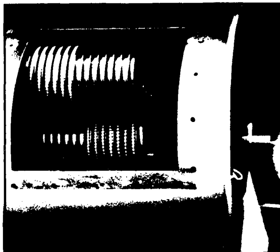
Fig. 5: Rotary Transfer Coupler for 6 optical fibres (by GKL, Elsdorf, FRG)
