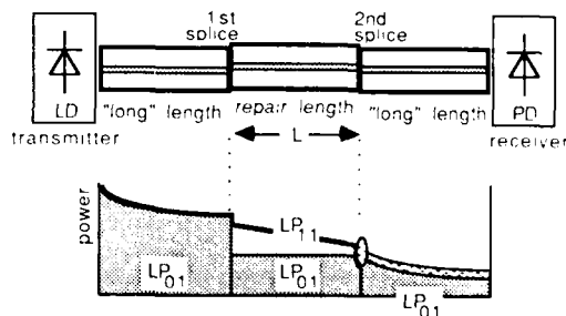
Fig. 6 Simulation of a Repair Section
