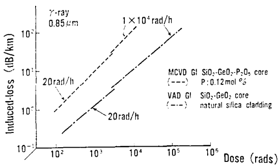
Fig.3 Increase of the \gamma -ray induced-loss of the graded-index fibers fabricated by (-----) MCVD and (-----) VAD process
