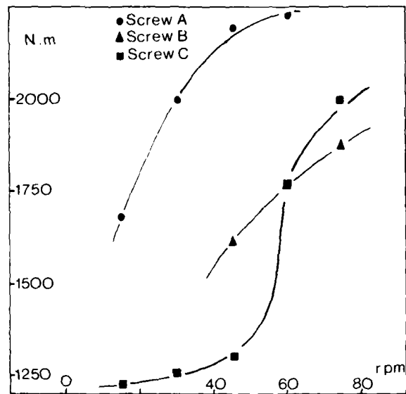
Figure 19. Screw Torque Versus Screw Speed
