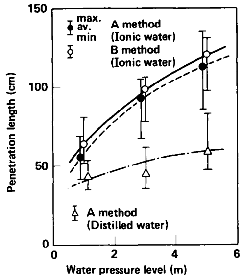
Fig.15 Penetration length as a function of water pressure level, using the waterproof test method as a parameter
