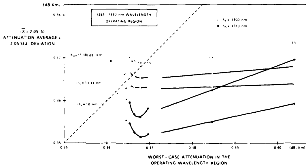
Figure 10 - Statistical vs. worst-case fibre attenuation in the 1285-1340 nm window, for GeO 2 -doped silica based single-mode fibres.
