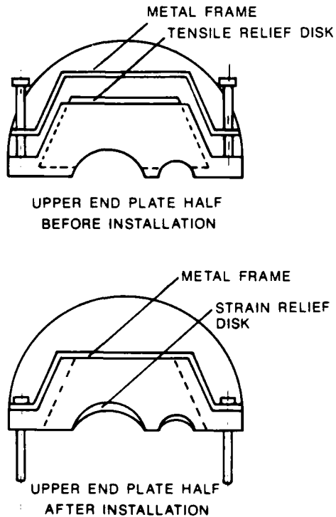
FIGURE 2 END CAP
