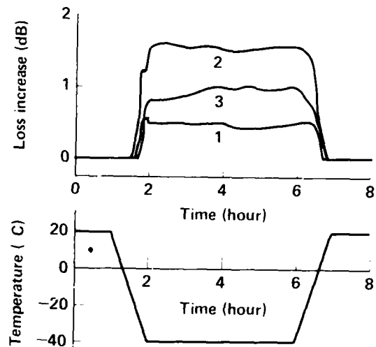
Fig.9 Loss increase of fiber in glass pipe model due to freezing
