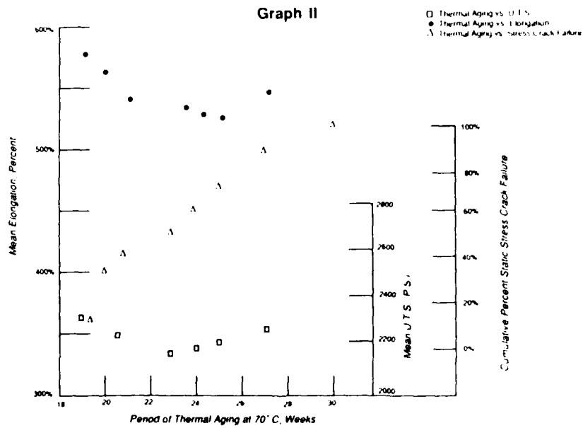
Foam Skin Insulation Static Stress Crack Failure Samples Pre-Conditioning 4 weeks @ 70°C
