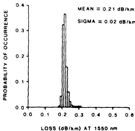
FIGURE 3. NEW NONMETALLIC CABLE -PRODUCTION RESULTS
