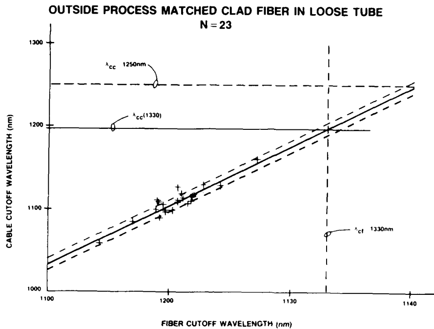
Figure 7. Typical Example of Measured \lambda_{cc} 's Plotted as a Function of \lambda_{ct} 's
