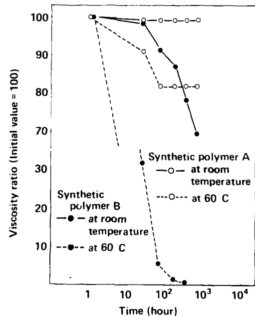
Fig.4 Viscosity changes in absorbent polymer gel due to thermal degradation as a function of time
