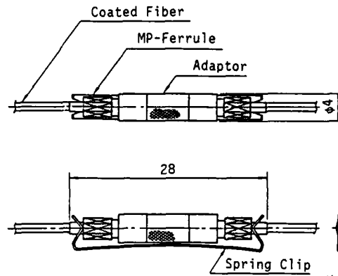
Figure 4 SP Connector with MP-Ferrule
