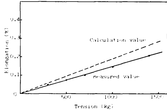
Fig.4 Tension-elongation characteristic
