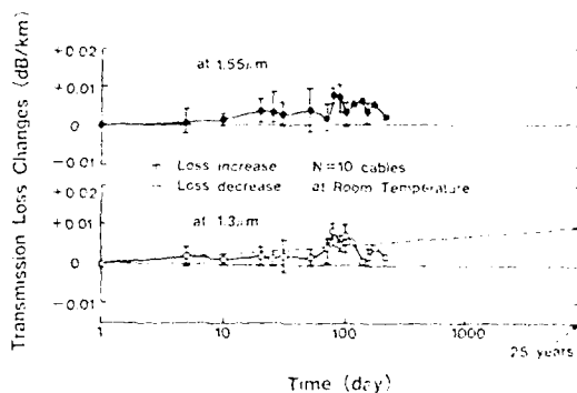
Fig.11 Transmission Loss Changes during Storage
