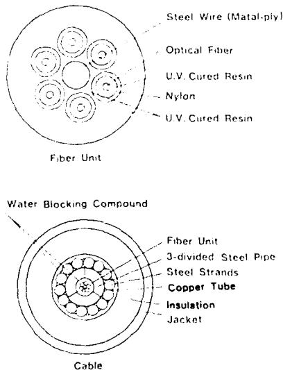
Fig.1 Optical Fiber Submarine Cable
