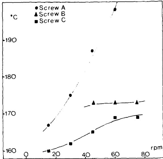
Figure 17. Melt Temperature Versus Screw Speed
