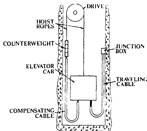
TYPICAL ELEVATOR
