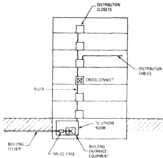
FIGURE 1. COMMERCIAL BUILDING DISTRIBUTION
