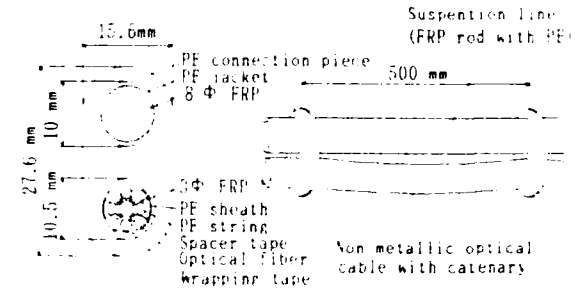
Fig. 2 Structure of non-metallic self-supporting optical cable
