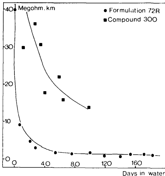
Figure 7. Insulation Resistance Constant vs Time
