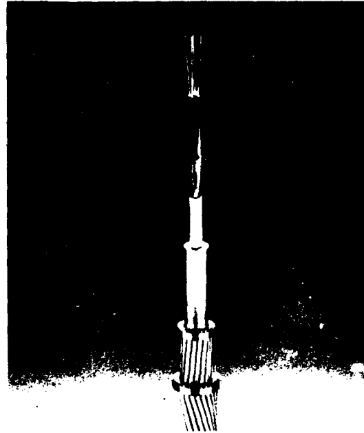
Fig. 1 Optical Overhead Ground Wire Single and Double Layer 4 to 12 Fiber
