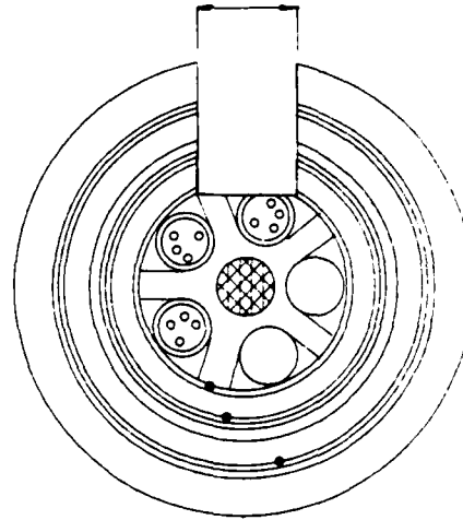
FIG. 6 6.4 mm HOLE DRILLED INTO CABLE
