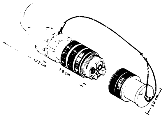
Figure 3. SIMFOCS Connector
