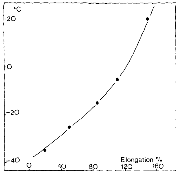
Figure 6. Elongation at Break vs Temperature
