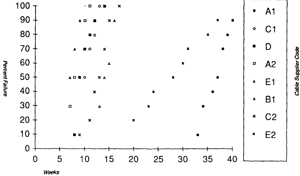
Cumulative Failure of Commercial Cable Preaged at 70°C and Aged at 70°C (% Failure vs. Weeks)
