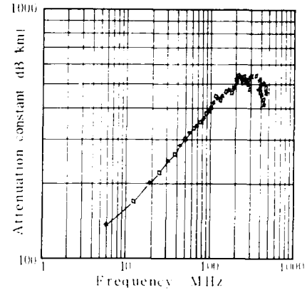
Fig. 7 The frequency dependence of attenuation
