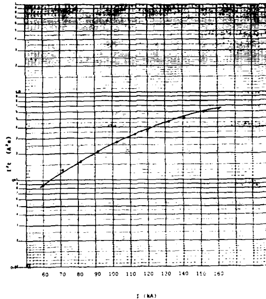
FIG. 2 REPRESENTATIVE VALUES OF I'c vs I FOR SIMULATED LIGHTNING TESTS
