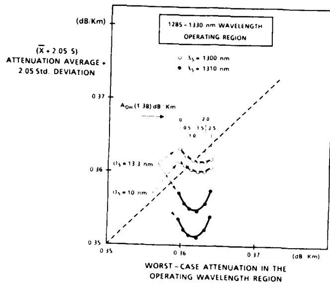
Figure 9 - Statistical vs. worst-case fibre attenuation in the 1285-1330 nm window, for GeO 2 -doped silica based single-mode fibres.
