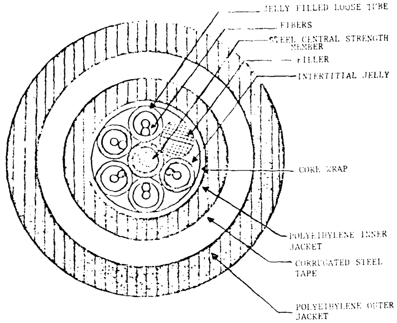
U.S. 1 ARMORED OPTICAL CABLE
