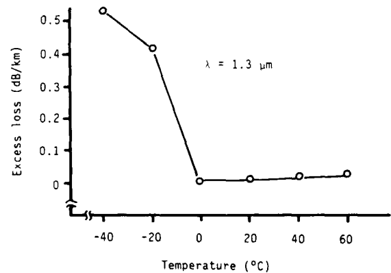
Figure 7 Thermal properties of water-penetrated cable
