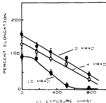
Fig.8 DEGRADATION OF PVC PHTHALATE BLEND UNDER 320-380nm LIGHT. Samples were pre-irradiated with \gamma -rays for 0( \bullet ), 4( \circ ) & 10( \blacksquare ) Mrad.
