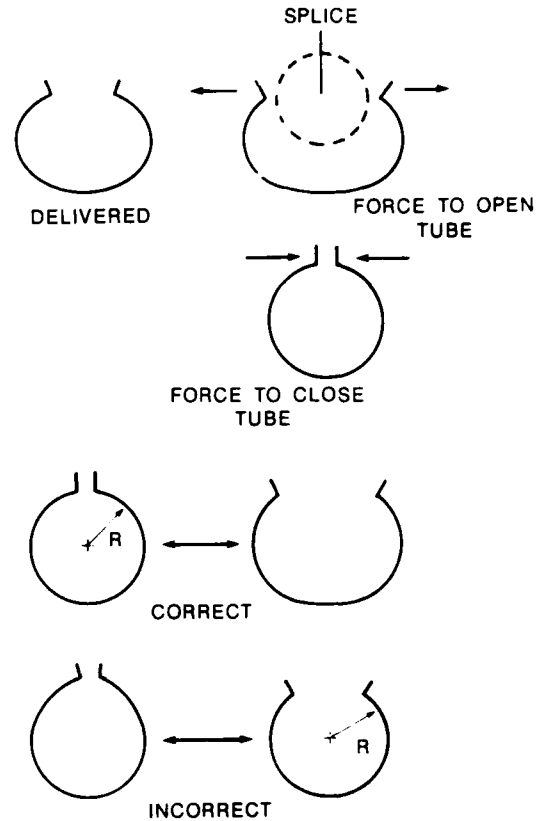
FIGURE 3 CLOSURE TUBE
