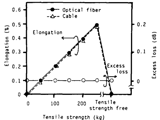
Figure 9 Relationship between tensile strength and elongation of optical fiber and cable (involving excess loss)
