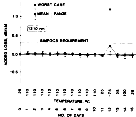
Figure 8. SIMFOCS Cable Accelerated Aging Test Results
