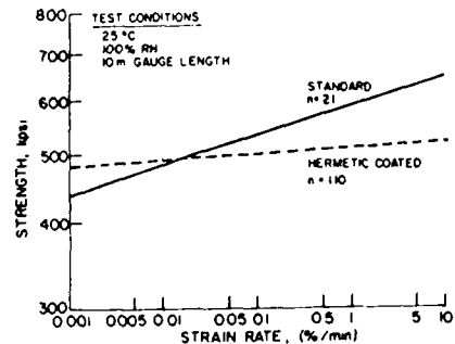
FIGURE 2 Dynamic Fatigue Of Hermetically Coated And Standard Fibers In 10 Meter Gauge Lengths
