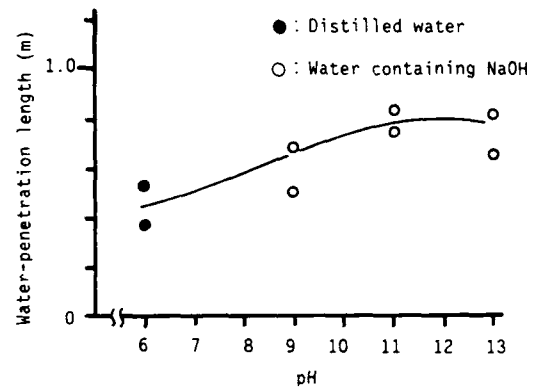
Figure 6 pH dependence of water-penetration length
