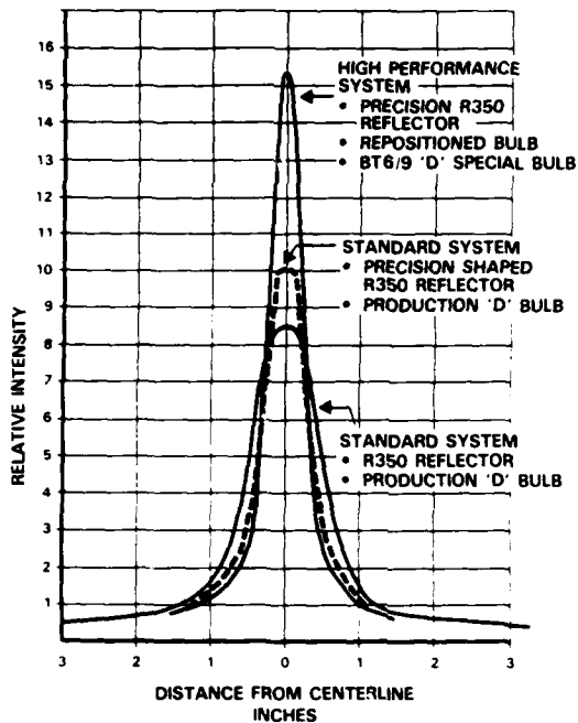
FIGURE 3 CENTERPEAK INTENSITY
