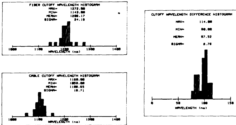
Figure 6. Examples of \lambda_{c,f} , \lambda_{c,c} , and \lambda_{c,f} - \lambda_{c,c} Histograms
