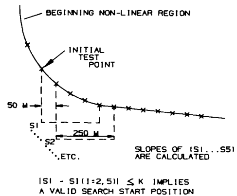
FIGURE 5. SEARCH START POSITION DETERMINATION
