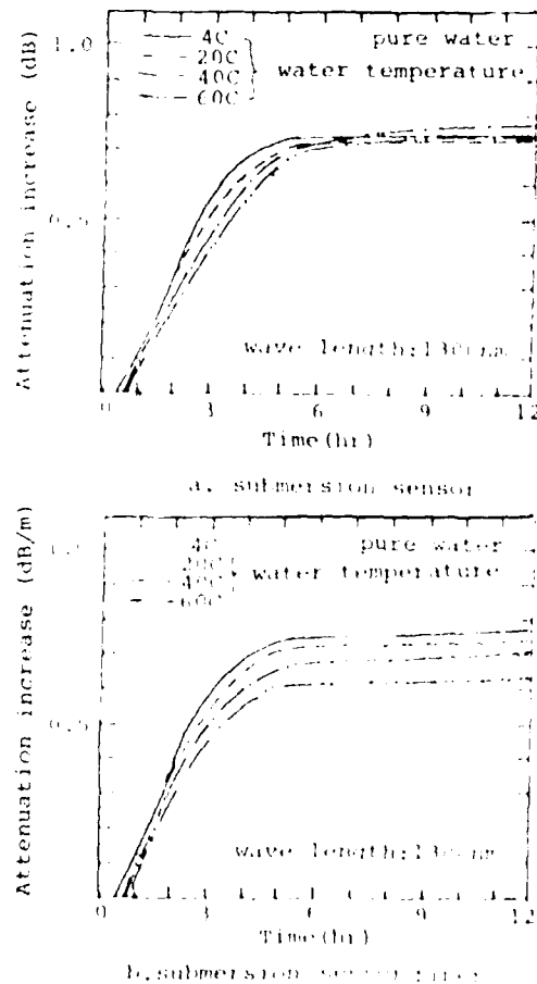
Fig.11 Temperature dependence of attenuation increase
