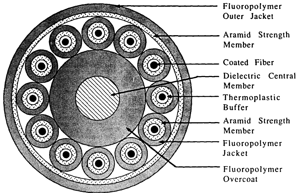
Figure 2: Siccor Fan-Out Intrabuilding Cable
