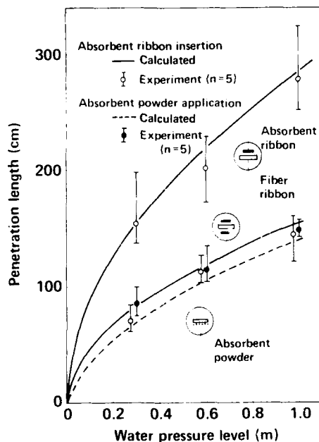
Fig.12 Initial penetration length in watercourse model
