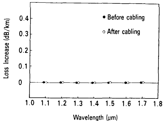
Figure 3 Transmission Loss Change during Cabling
