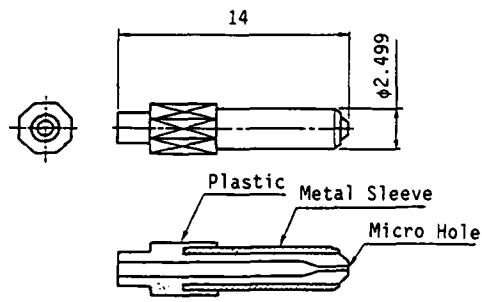
Figure 1 MP-Ferrule
