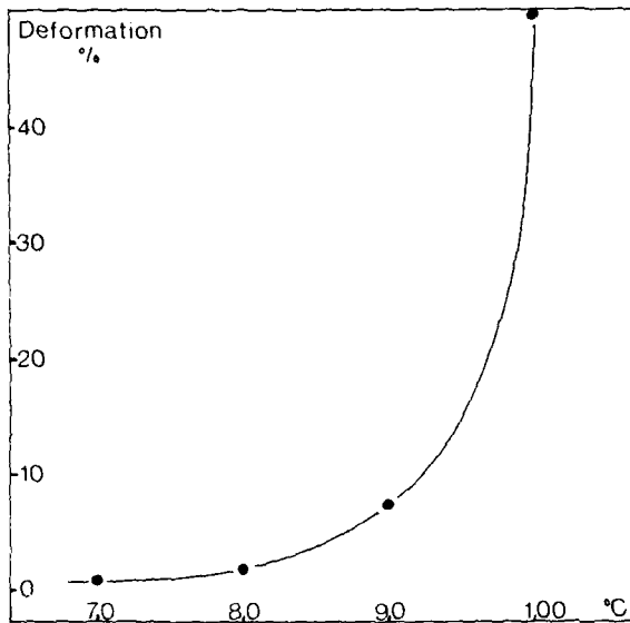
Figure 4. Hot Deformation Test BS 6469:1984
