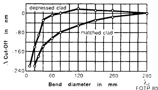
Fig. 5 Shift of Effective Cutoff Wavelength for a Single Loop in 2m of Fiber ( \Delta n = 0.35\% )
