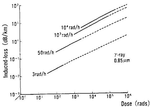
Fig.4 Increase of the \gamma -ray induced-loss of the graded index fibers with germanium-doped silica core fabricated by VAD process and synthetic silica cladding. The dashed curves represent the increases extrapolated.
