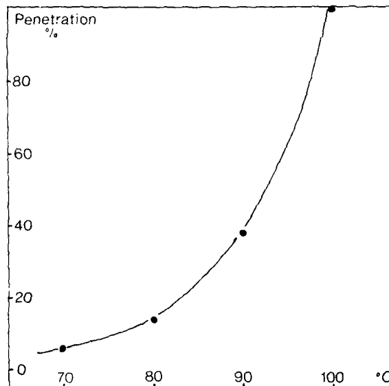
Figure 5. Hot Pressure Test BS 6469:1984
