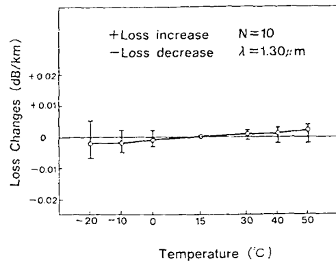
Fig.4 Temperature-Loss Characteristic
