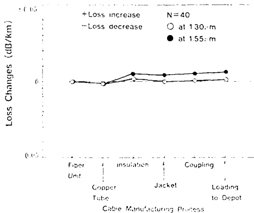
Fig.3 Average Loss Characteristics during Cable Manufacturing
