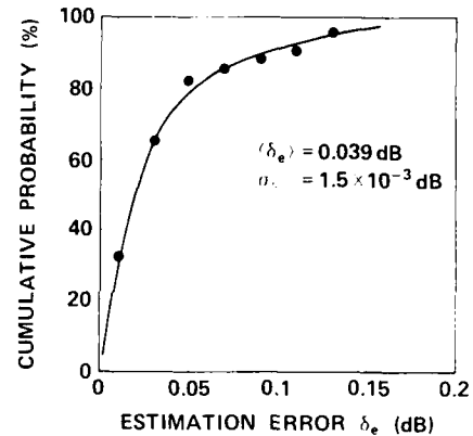
Fig.13 Cumulative probability of estimation error.
