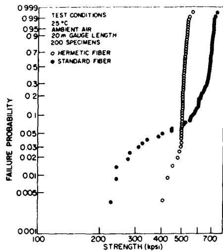
FIGURE 1 Weibull Strength Distribution Plots For Hermetically Coated And Standard Fibers
