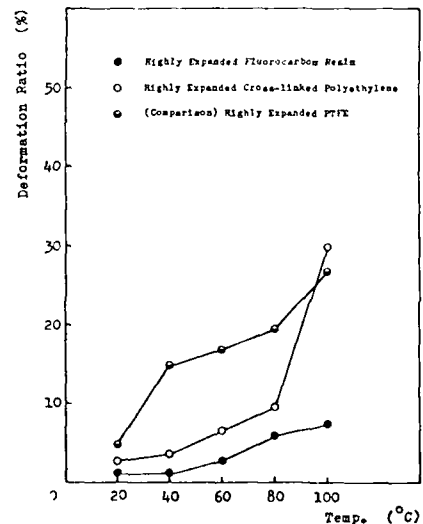
Fig.9 Heat Deformation Properties
