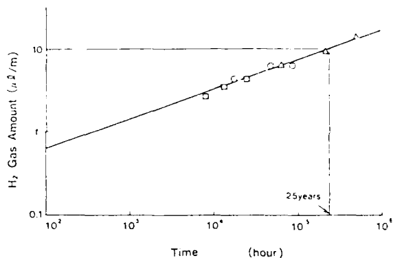
Fig.8 Estimated H 2 gas Amount at 3°C
