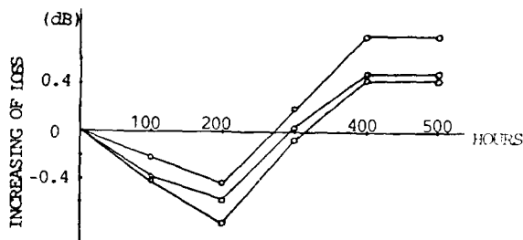
Fig 12 Optical loss at 150 degrees c
