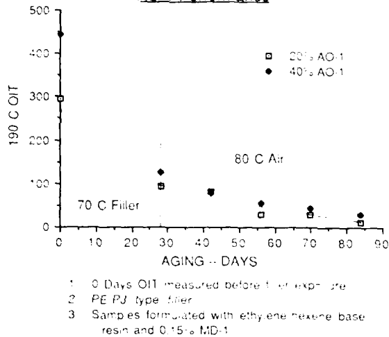
Figure 2 AO-1 Performance
