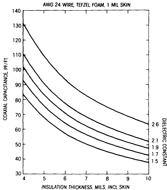
Figure 14 COAXIAL CAPACITANCE
