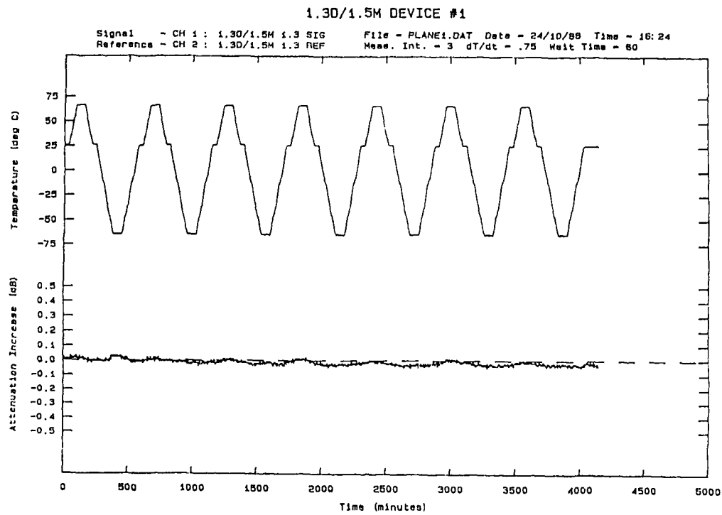
Figure 5 - WDM Temperature Test Results
