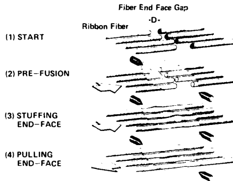
Fig.5 Fusion splicing process for the present method.
