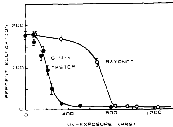
Fig.4 320-380nm DEGRADATION OF SPOOL SAMPLE.
