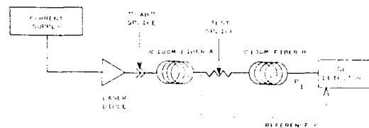
FIGURE 2. MEASUREMENT OF LOSS CUTBACK METHOD SOURCE STE LOSS = P_0 - P_1
