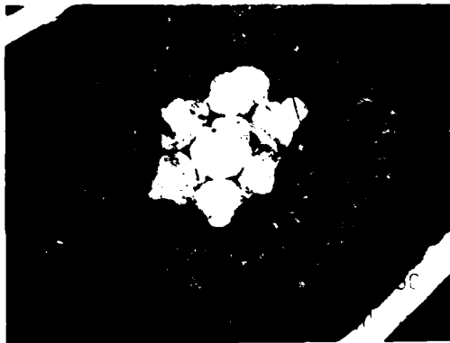
Figure 6a. 6 Nickel plated conductor Thermally Aged at 650 C. Magnification 75X (11.44 micron Nickel plate thickness)
