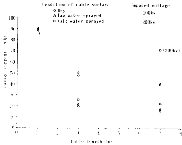
Fig. 6 Relationship between cable length and leakage current
