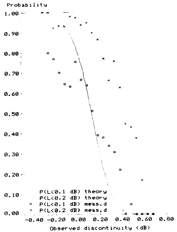
Figure 3. Probability of obtaining splice losses <math>< 0.1 \text{ dB}</math> and <math>< 0.2 \text{ dB}</math> vs. measured OTDR reading (theory and experimental data)
