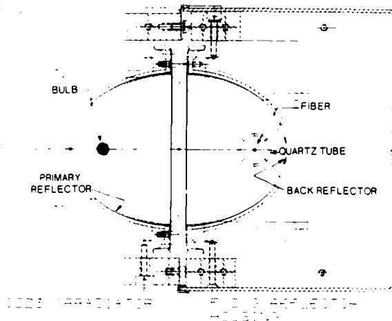
FIGURE 6 REFLECTOR SYSTEM
