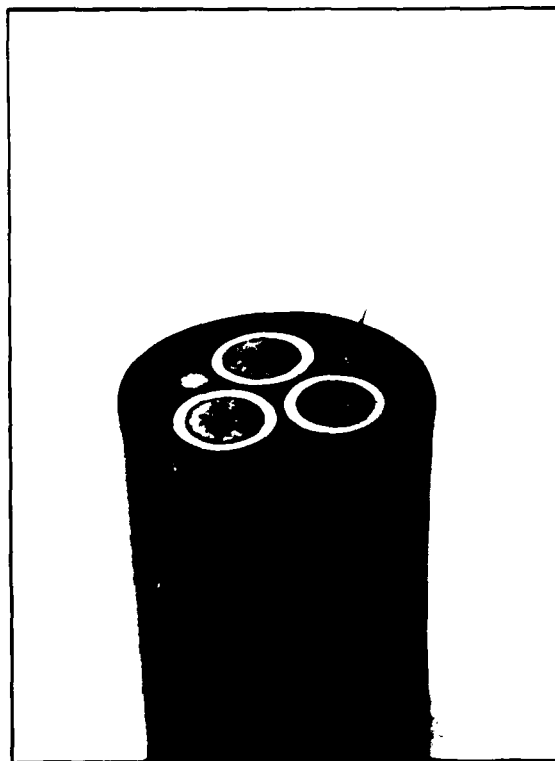
Fig. 3: Drag Cable 3 \times 120 + 2 \times 35 with 6 optical fibres
