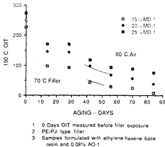
Figure 3 MD-1 Performance
