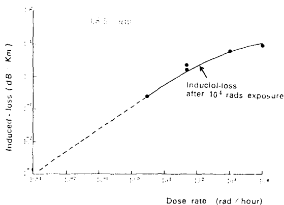
Fig.5 Dependence of the induced-losses after 10^4 rads exposure on the dose rate. The dashed curve represents the induced-loss extrapolated.
