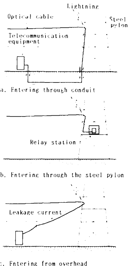
Fig. 12 Configuration of optical cable entering an installation housing
