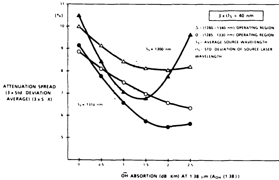
Figure 6 - Influence of hydroxyl (OH) impurity in the attenuation spread of GeO 2 -doped single-mode fibres operating in the 1285-1330 nm and in the 1280-1340 nm windows. The standard deviation in the source lasing wavelength is assumed to be 13.33 nm.
