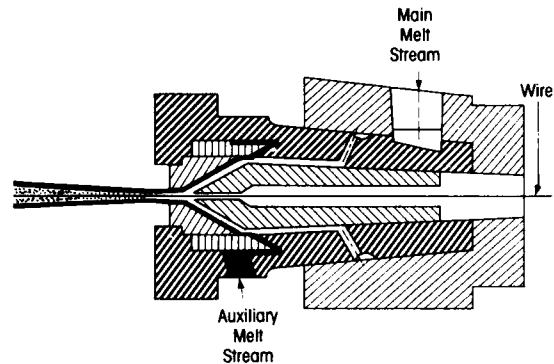
Figure 9 DUAL EXTRUSION FOR FOAM-SKIN PRODUCTION
