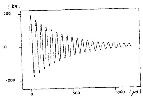
Fig. 6 Oscillating Wave Form for Lightning Simulation Test.
