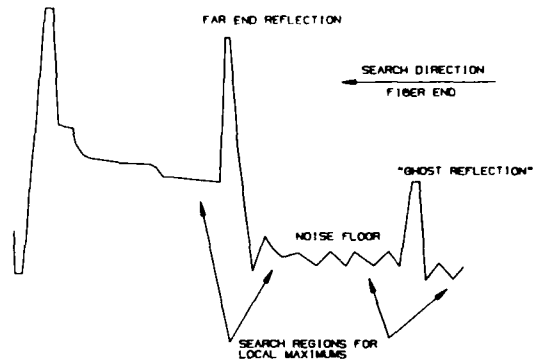
FIGURE 3. LOCATION OF FIBER END
