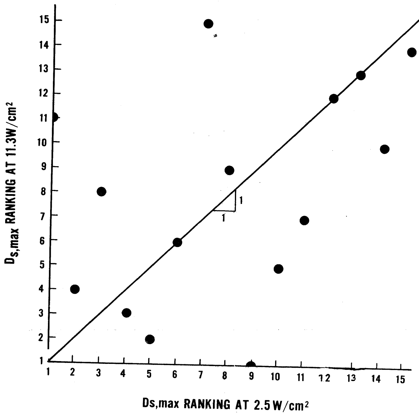
Figure 4. D_{s,max} Rankings at two Flux Levels from Brown [23] for Piloted Ignition.
