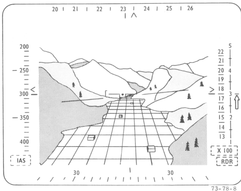
FIGURE 8. ELECTRONIC ATTITUDE DIRECTOR INDICATOR WITH TERRAIN CLEARANCE PRESENTATION
