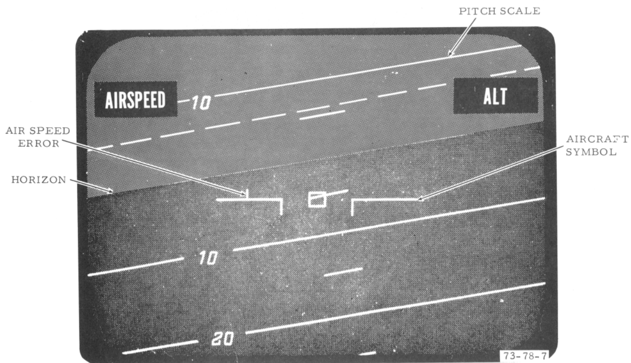
FIGURE 7. ELECTRONIC ATTITUDE DIRECTOR INDICATOR WITH FLIGHT DIRECTOR PRESENTATION
