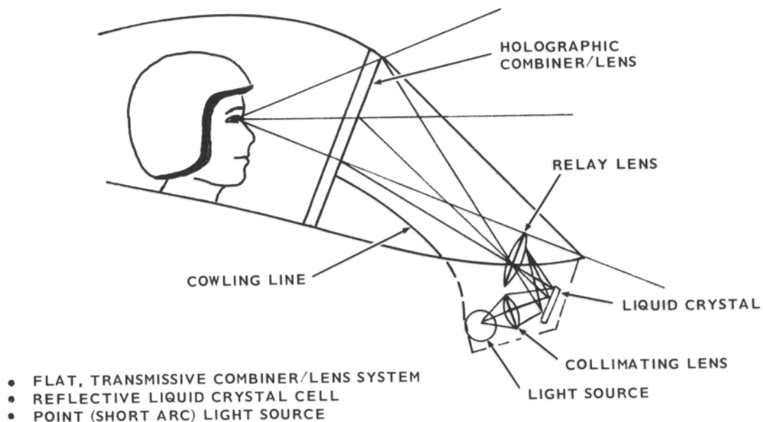
FIGURE 2. HEAD-UP DISPLAY BASELINE SYSTEM DESIGN (INDEX NO. 146)
