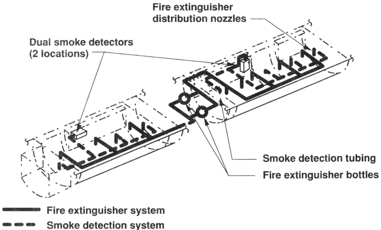
Figure 3-5. 757-200 Cargo Compartment Fire Protection.
