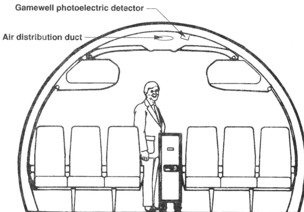
Figure 5-8. Attic Detectors.
