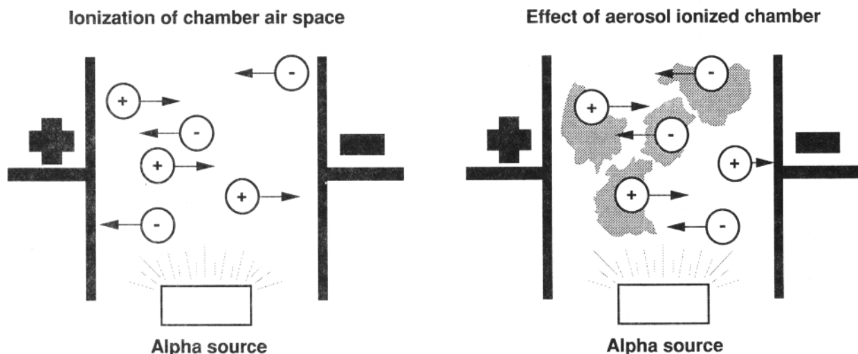
Figure 4-8. Ionization Detector.
