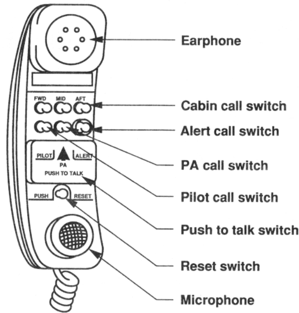
Figure 3-11. Communications Handset.
