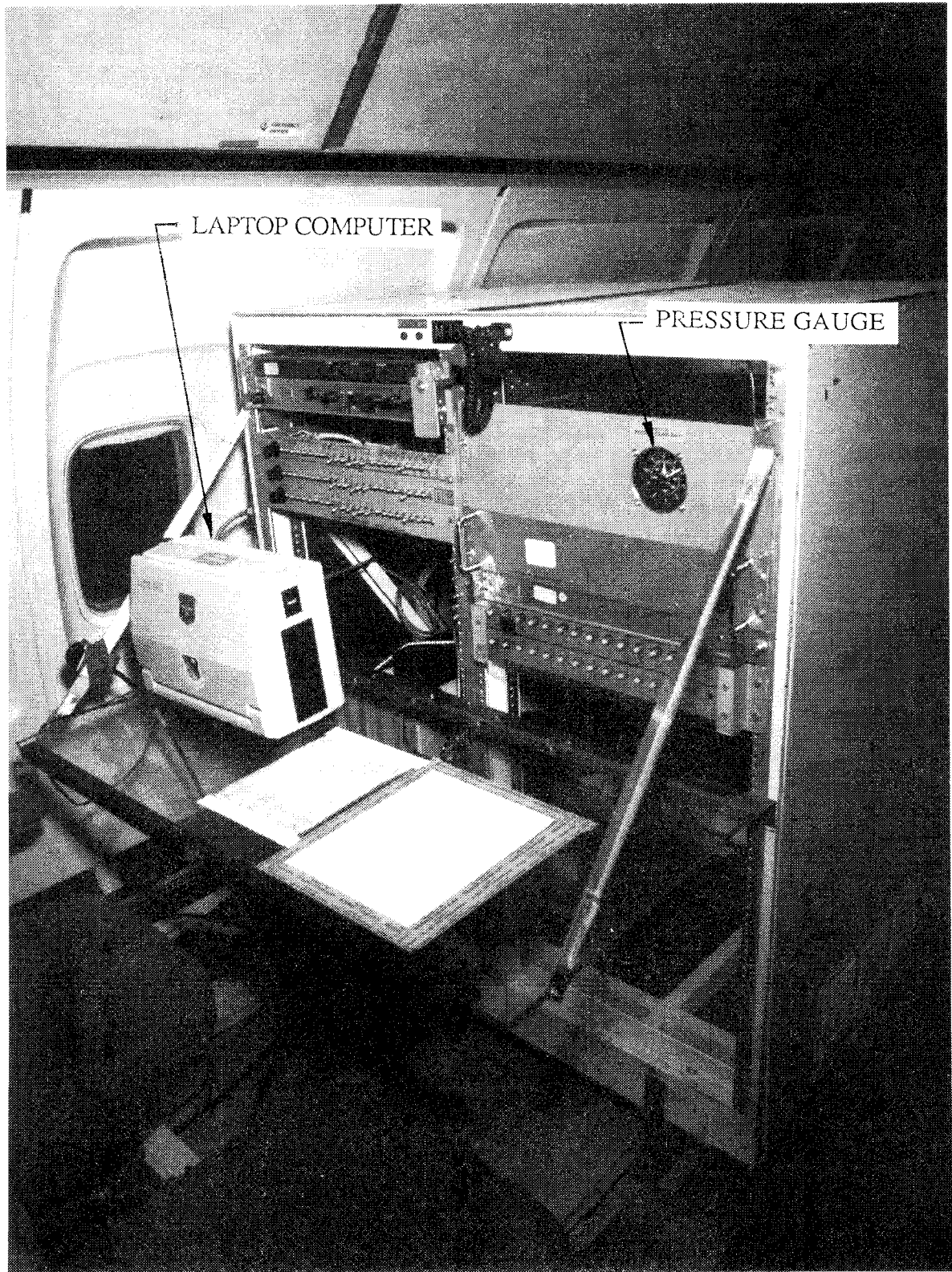
FIGURE 2.1.1-3 INSTRUMENT RACK, STATION 1080, AFT FACE
