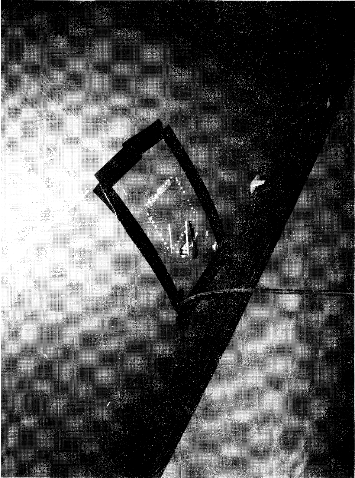
FIGURE 2.2.2-1 HELIUM HOSE AT ACCESS HATCH
