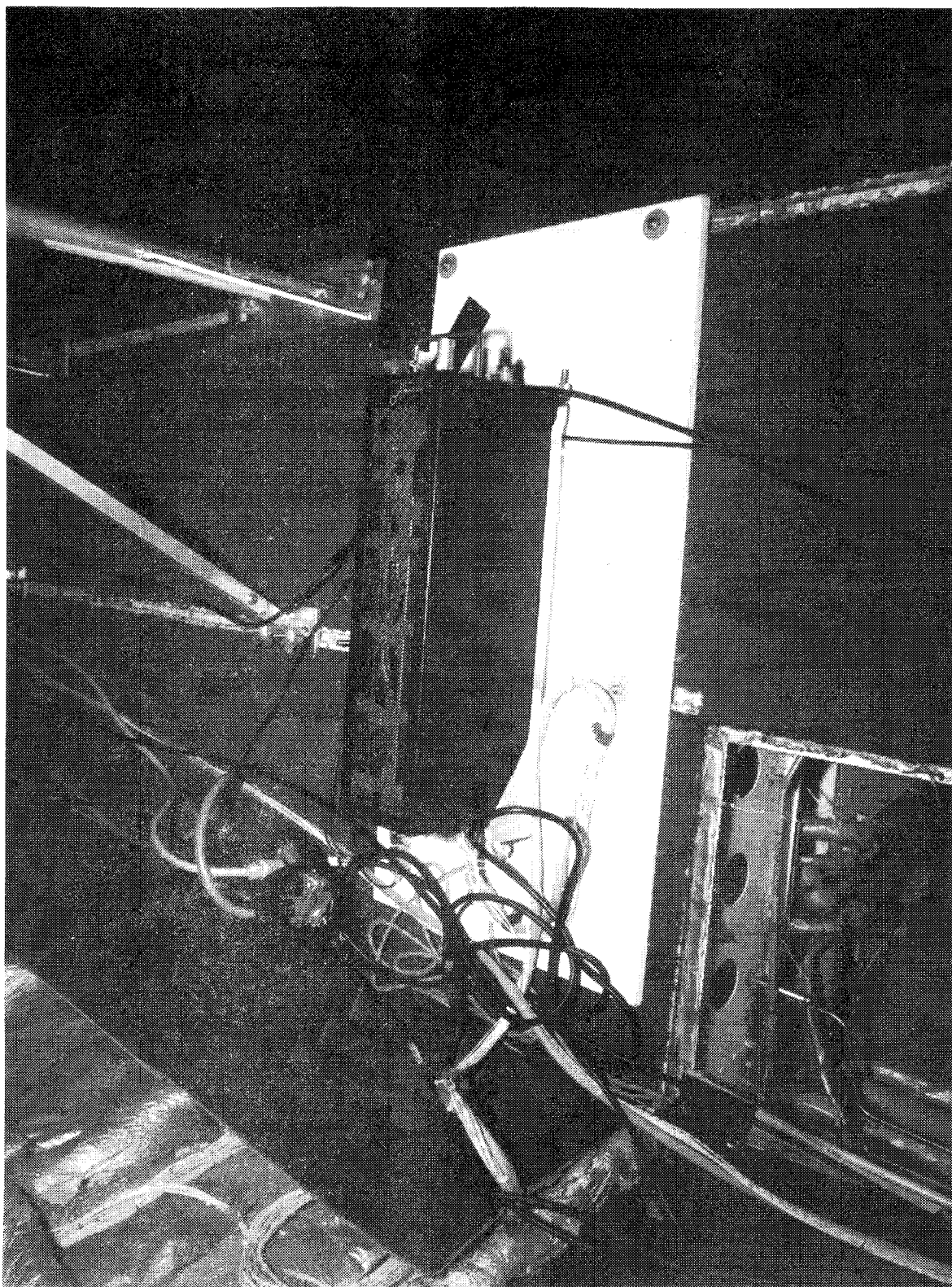
FIGURE 2.1.2-3. CABIN PRESSURE CONTROLLER (ON CABIN FLOOR)
