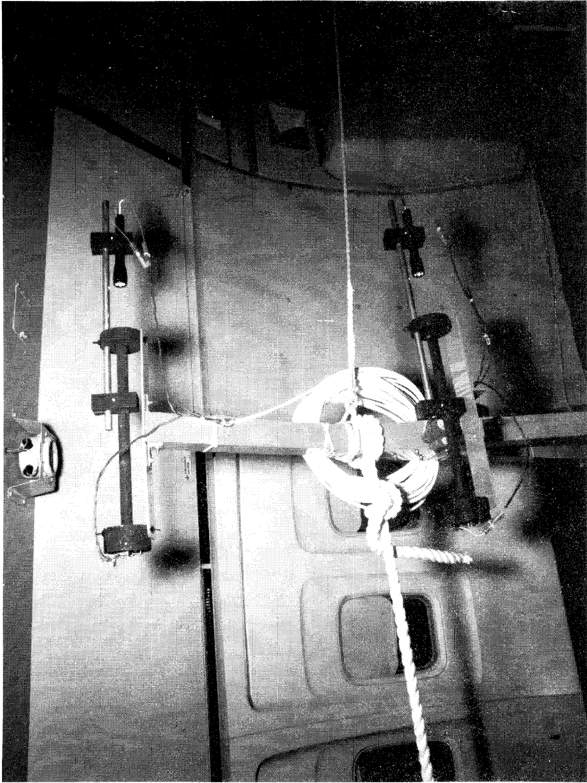
FIGURE 2.3.2-1. SMOKE METERS, TYPICAL FOR STATIONS 560, 800, 1030 AND 1270
