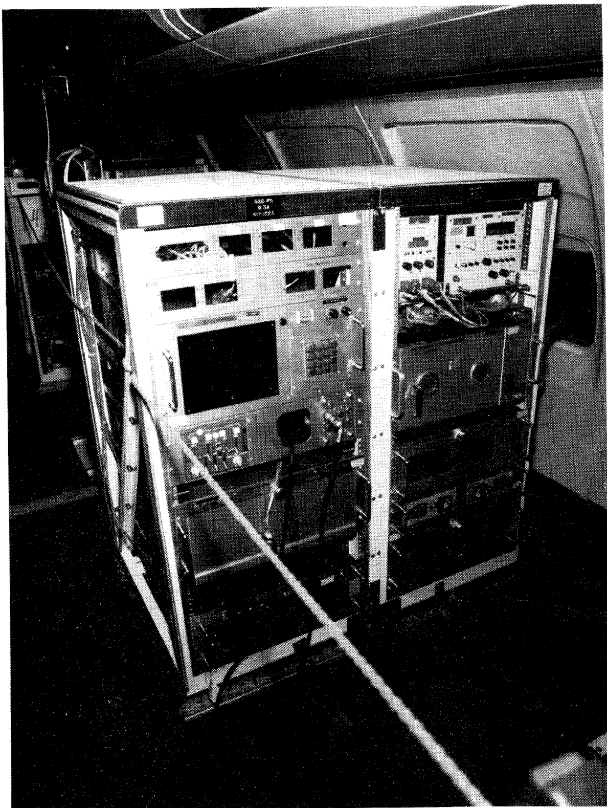
FIGURE 2.1.1-9 INSTRUMENT RACK, STATION 1548, RIGHT SIDE
