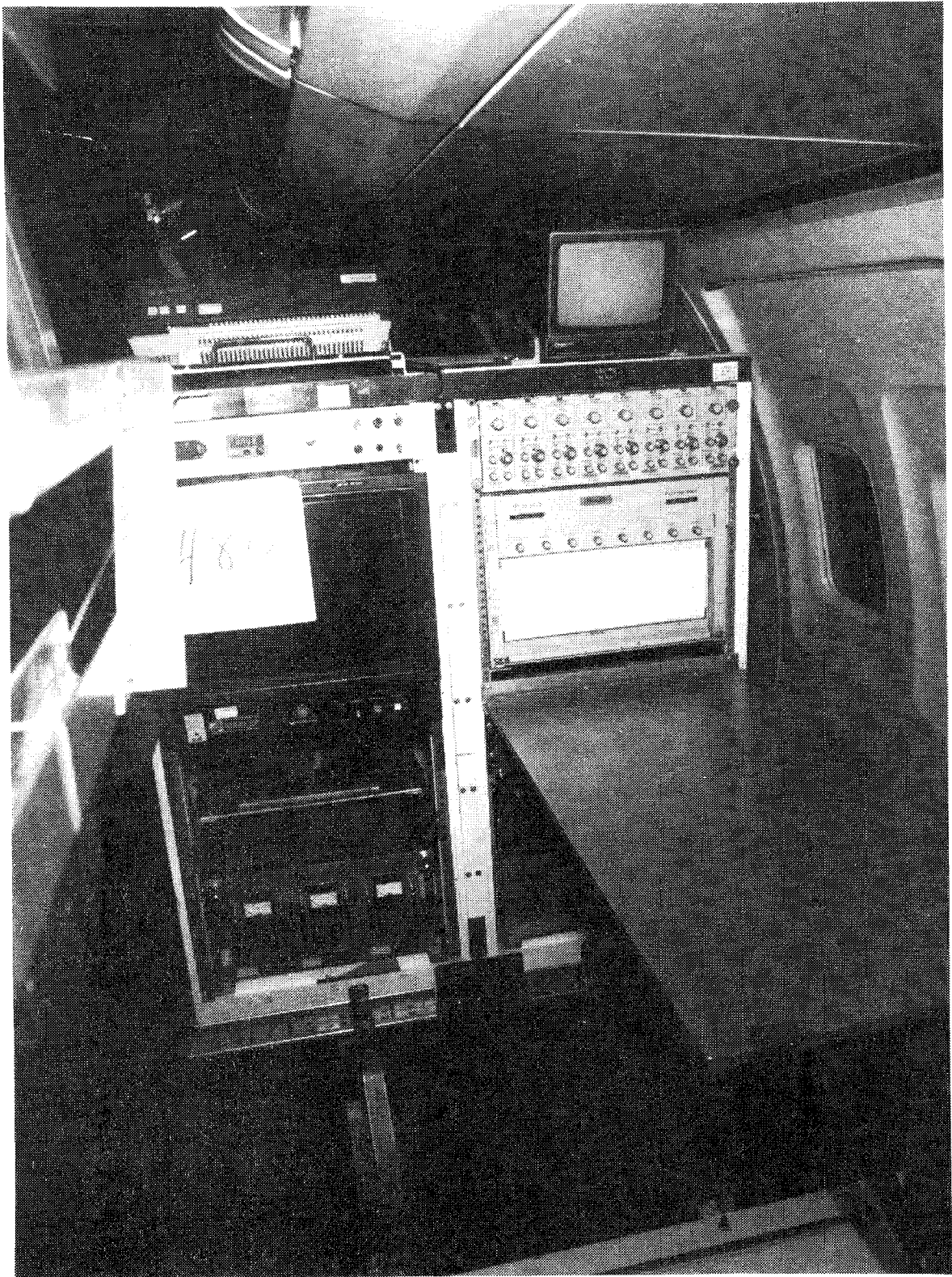
FIGURE 2.1.1-7 INSTRUMENT RACK, STATION 1448, RIGHT SIDE
