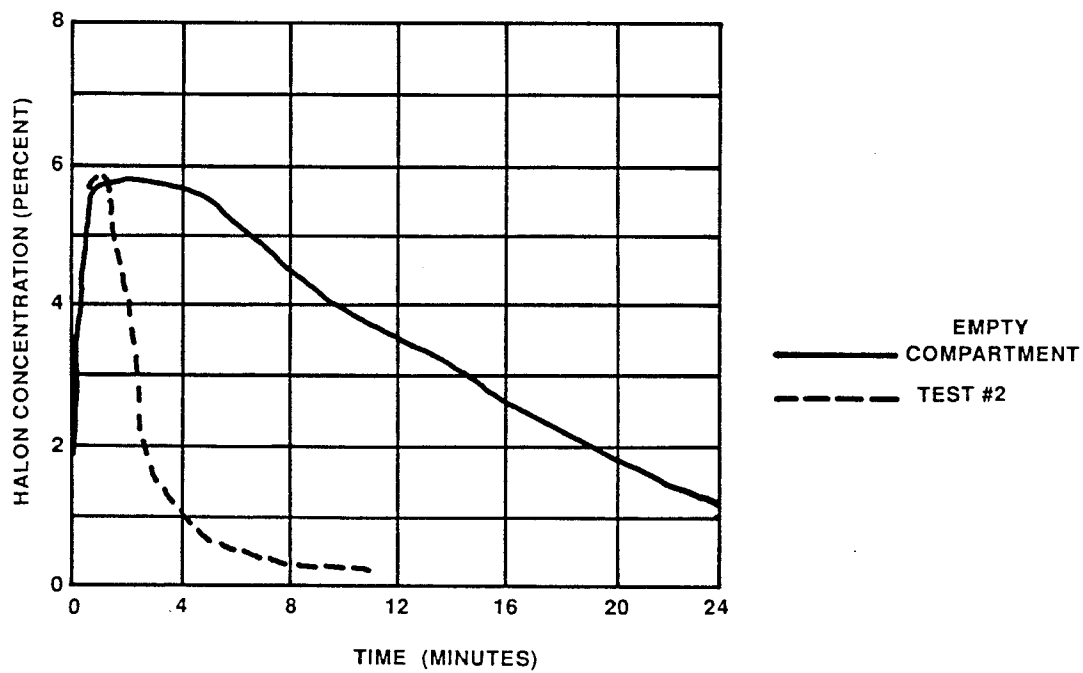
FIGURE 7. HALON CONCENTRATION
