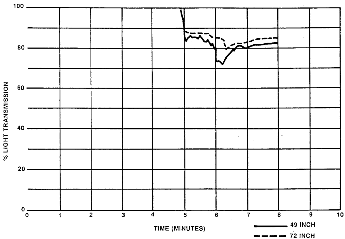
FIGURE 6. MID-CABIN SMOKE - TEST 3
