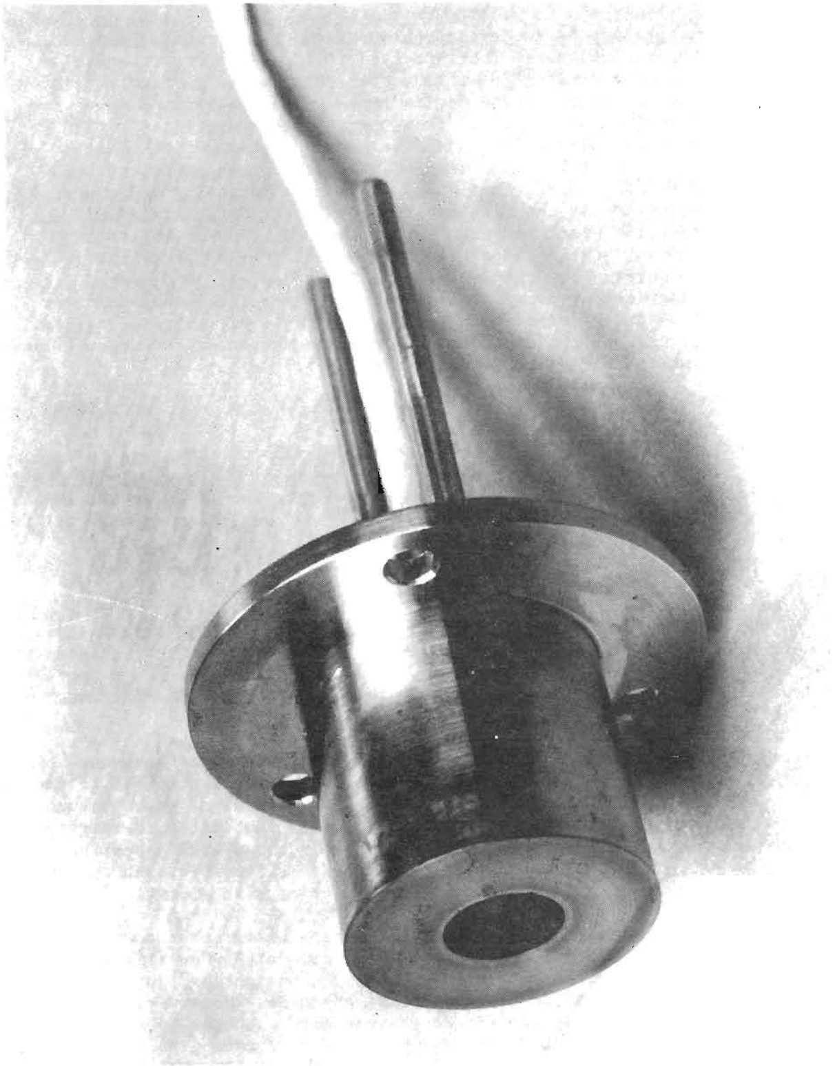
FIGURE 1. GARDON HEAT FLUX GAUGE
