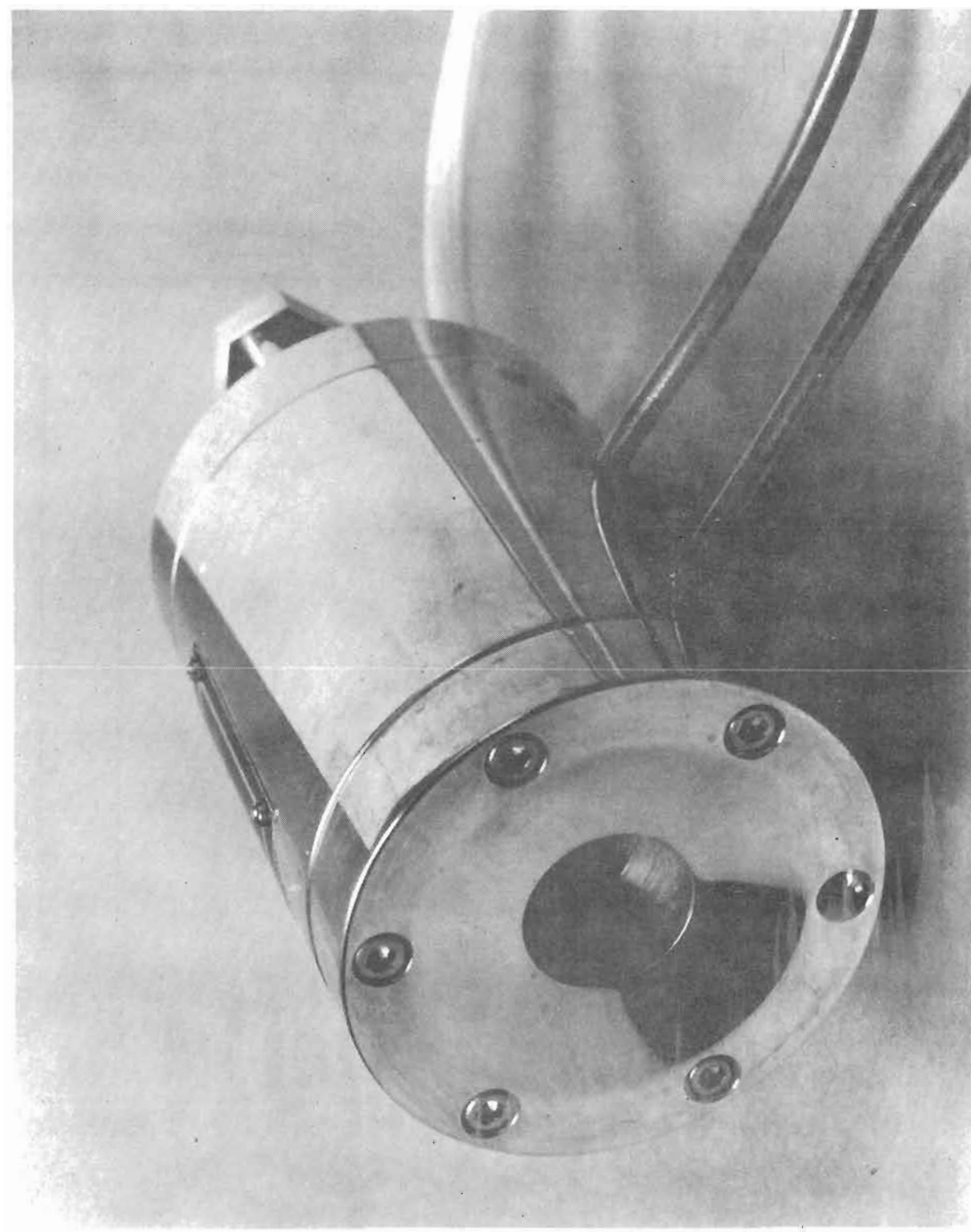
FIGURE 5. REFERENCE RADIOMETER (CFR ECR)
