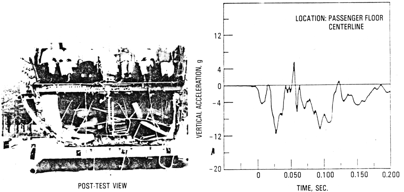
Figure 3-13. Results of Narrow-Body Airplane Forward Fuselage Section (With Cargo) Test (Reference 16)
