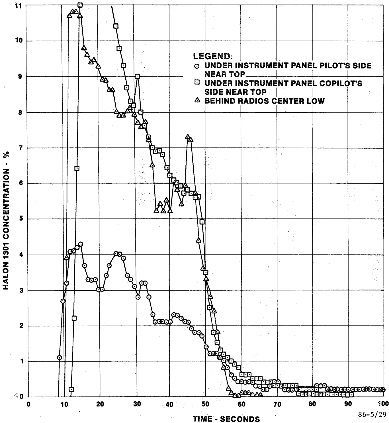
FIGURE 29. HALON 1301 CONCENTRATIONS - 3-POUND EXTINGUISHER DIRECTED UNDER THE INSTRUMENT PANEL - COPILOT'S SIDE - ALL SAMPLE LINES UNDER INSTRUMENT PANEL
