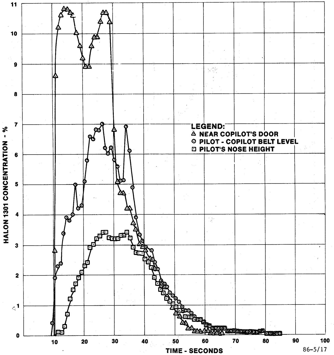
FIGURE 17. HALON 1301 CONCENTRATIONS - 3-POUND EXTINGUISHER DIRECTED TO THE COPILOT'S DOOR - OVERHEAD VENTS OPEN
