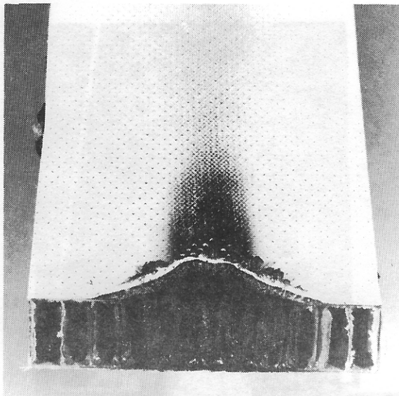
GEOMETRIC CENTER FLAME PLACEMENT
