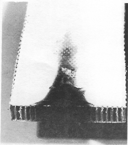
GEOMETRIC CENTER FLAME PLACEMENT
