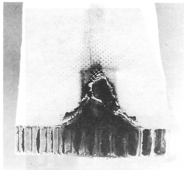
MIDPOINT-LOWER EDGE-FRONT FACE FLAME PLACEMENT
