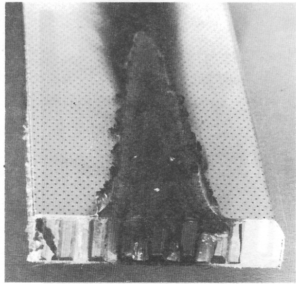
MIDPOINT-LOWER EDGE-FRONT FACE FLAME PLACEMENT
