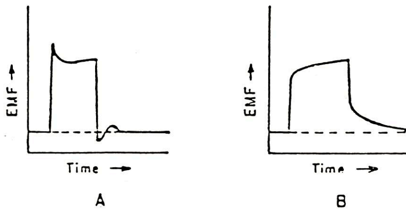
Figure 5. Square Wave Response
