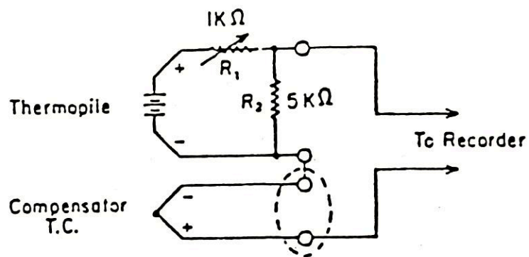
Figure 4. Wiring Diagram
