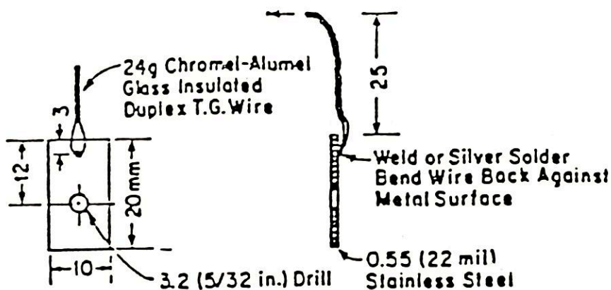
Figure 2. Compensator Tab
