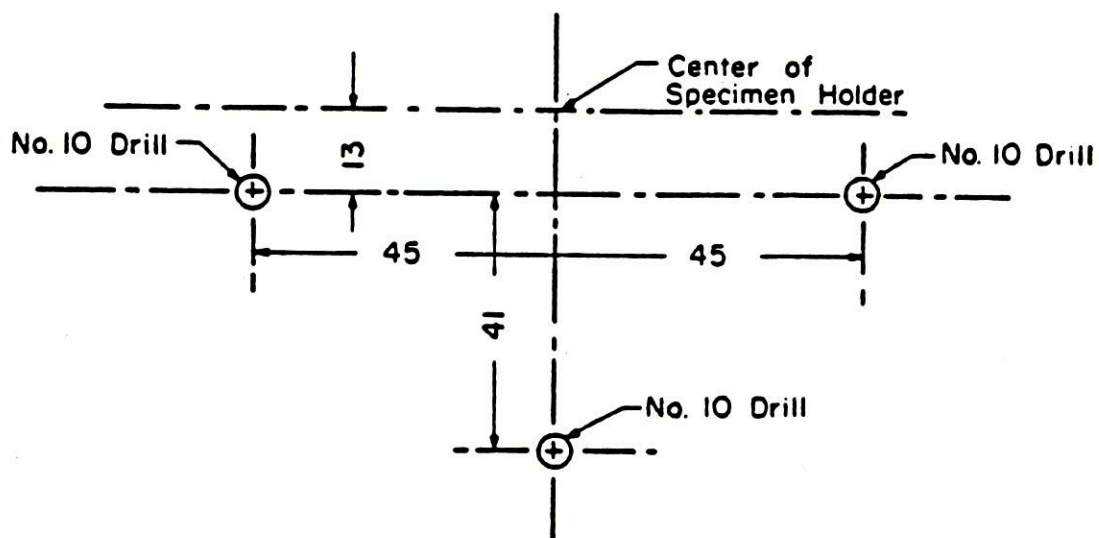
TEMPLATE FOR MOUNTING BOLTS VERTICAL MOUNT
