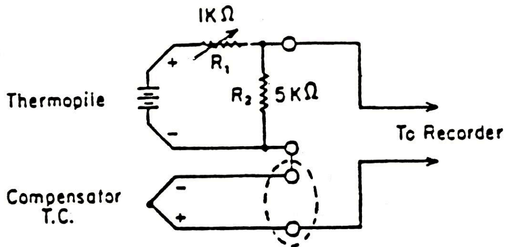
Figure 4. Wiring Diagram
