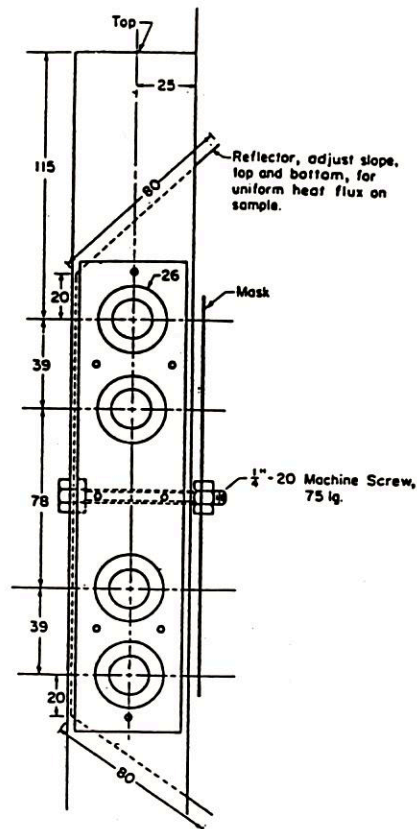
Figure 6B. "Globar" Radiant Panel
