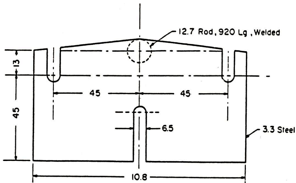
VERTICAL SUPPORT
