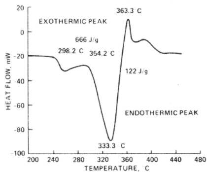
Figure 5: Differential Scanning Calorimetry of Vonar R 2
