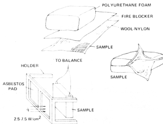
Figure 3: Sample Configuration
