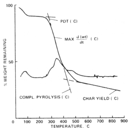
Figure 4: Typical Thermogram
