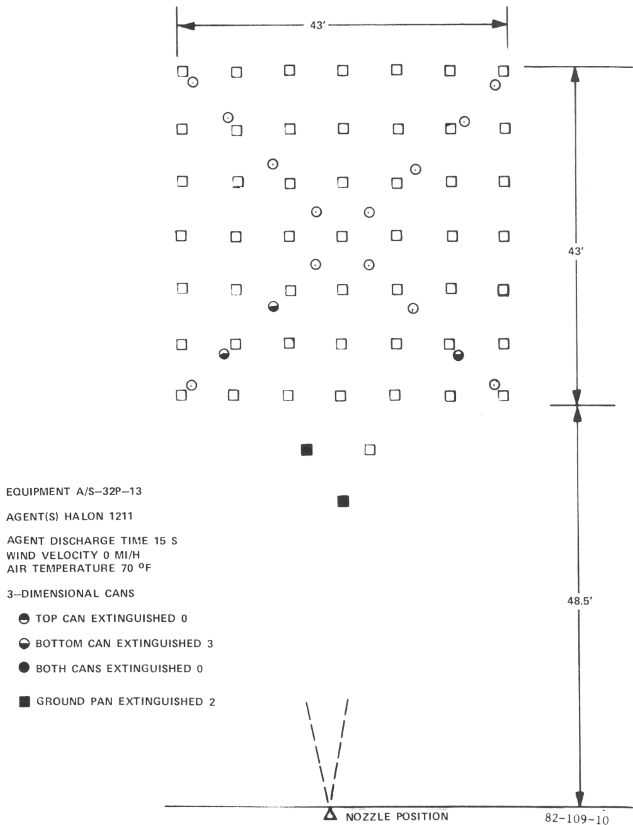
FIGURE 10. EFFECTIVE THROW RANGE OF HALON 1211
