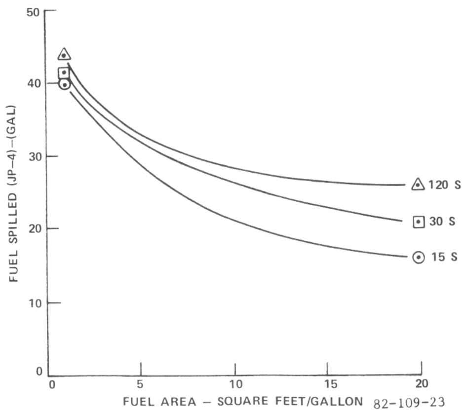
FIGURE 23. AREA OF FUEL SPREAD ON A RUNWAY SURFACE BEFORE AND AFTER IGNITION
