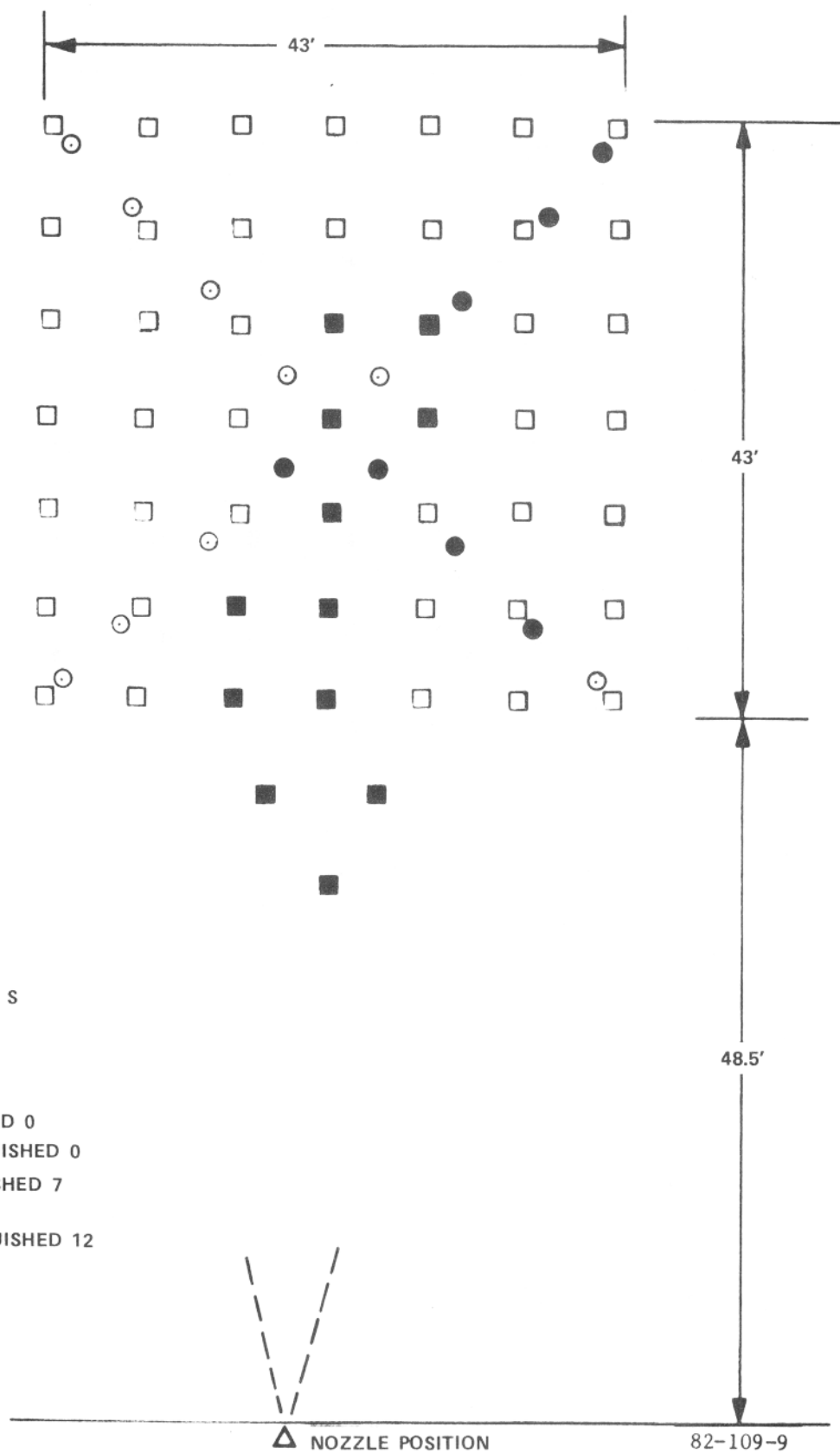
FIGURE 9. EFFECTIVE THROW RANGE OF MONNEX DRY POWDER
