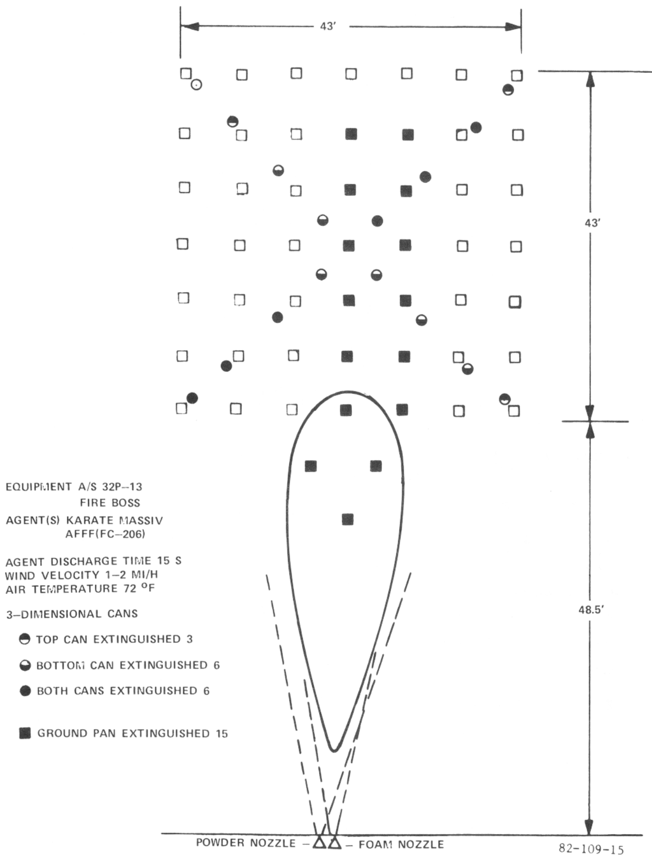
FIGURE 15. EFFECTIVE THROW RANGE OF KARATE MASSIV AND AFFF (FC-206) SIMULTANEOUSLY
