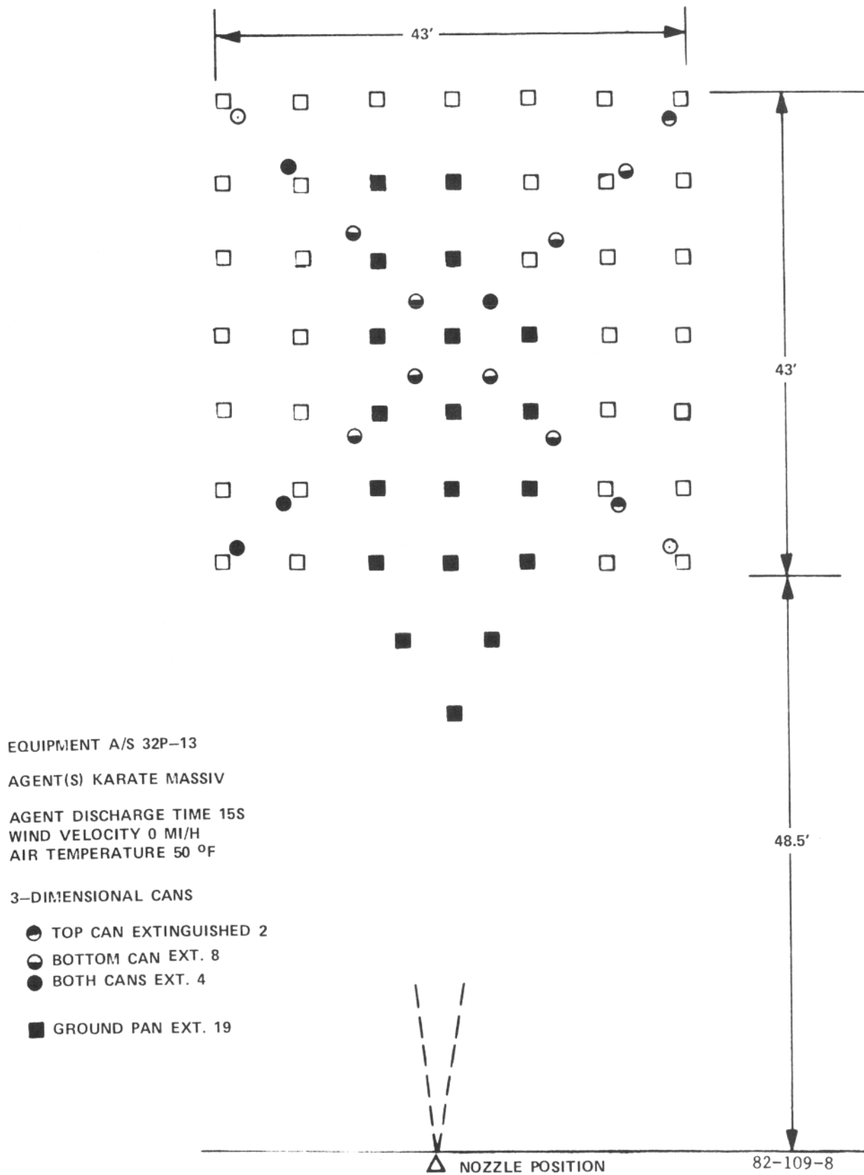
FIGURE 8. EFFECTIVE THROW RANGE OF KARATE MASSIV DRY POWDER
