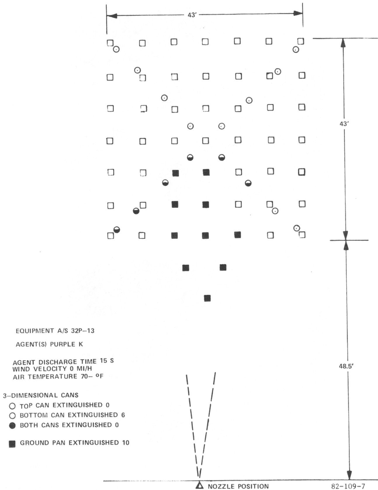
FIGURE 7. EFFECTIVE THROW RANGE OF PURPLE K POWDER
