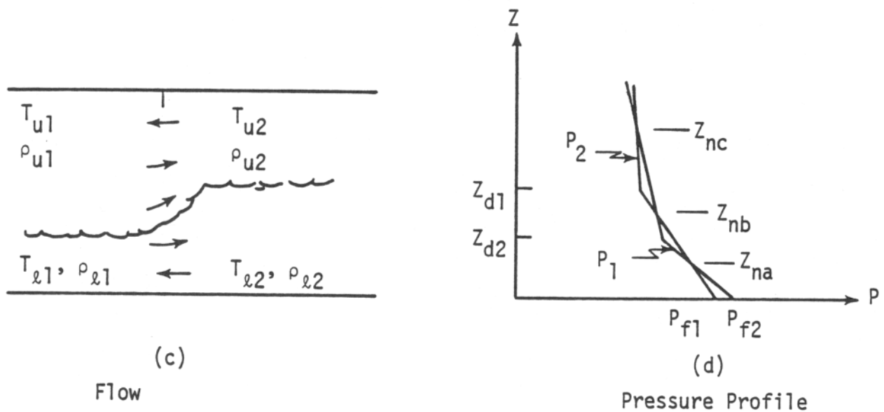
(a) & (b) Single Compartment Flow to Exterior (c) & (d) Flow Between Two Compartments
