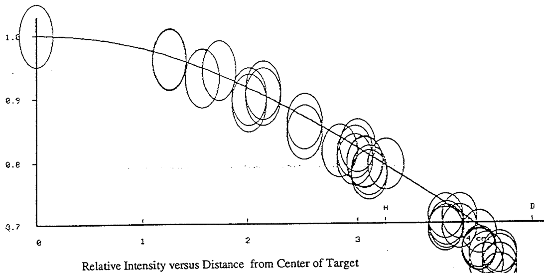
Figure 13. Radial Scan of Tubular Heater Fields with Errors Compared to Ideal
