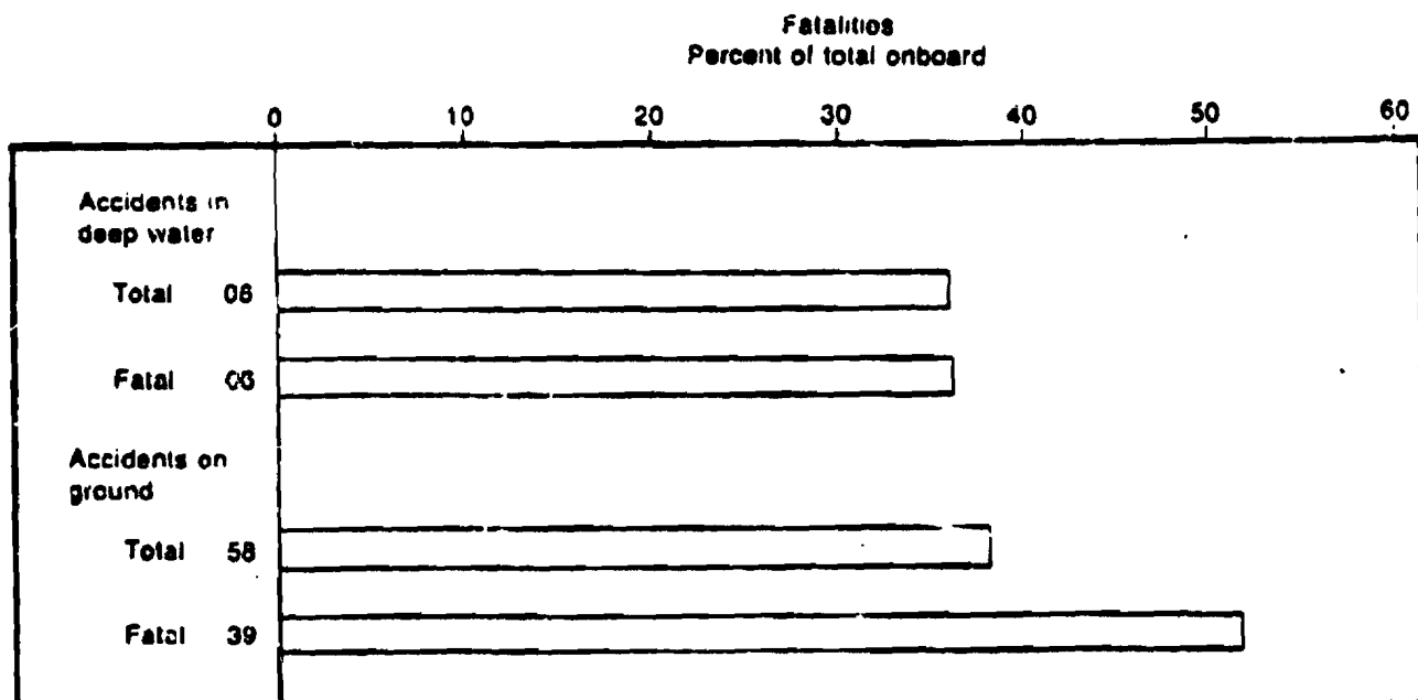
FIGURE 5. FATALITIES VERSUS ACCIDENT TYPE
