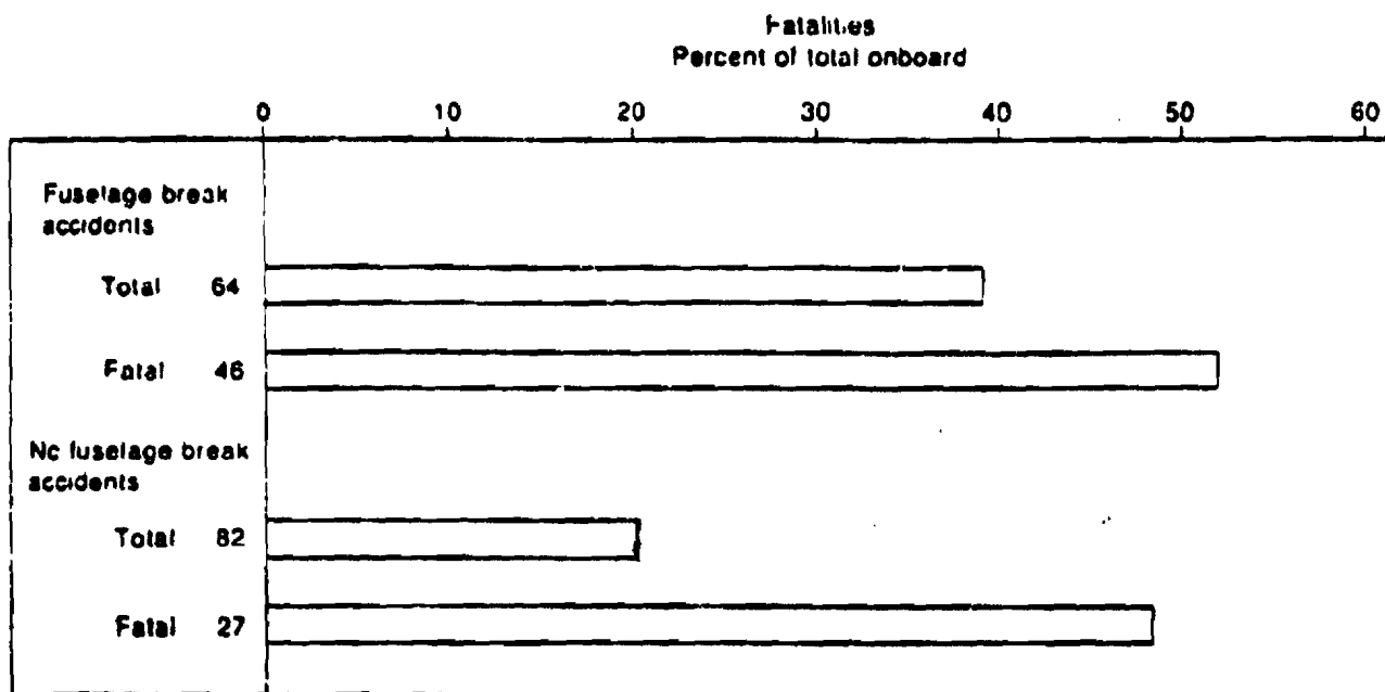
FIGURE 4. FATALITIES VERSUS FUSELAGE BREAK
