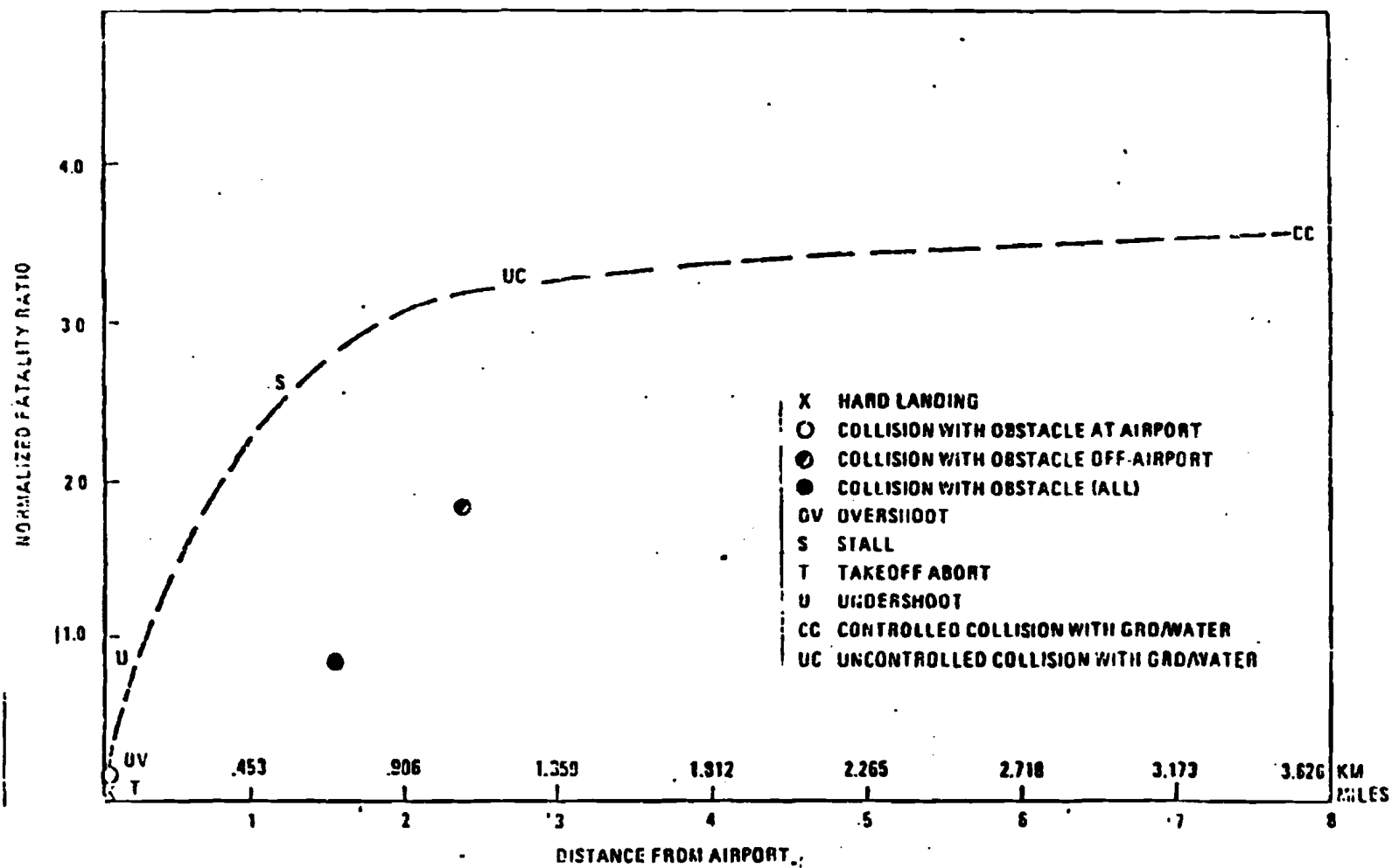
FIGURE 10. NORMALIZED FATALITY RATIO AS A FUNCTION OF DISTANCE FROM AIRPORT FOR CRASH SCENARIOS
