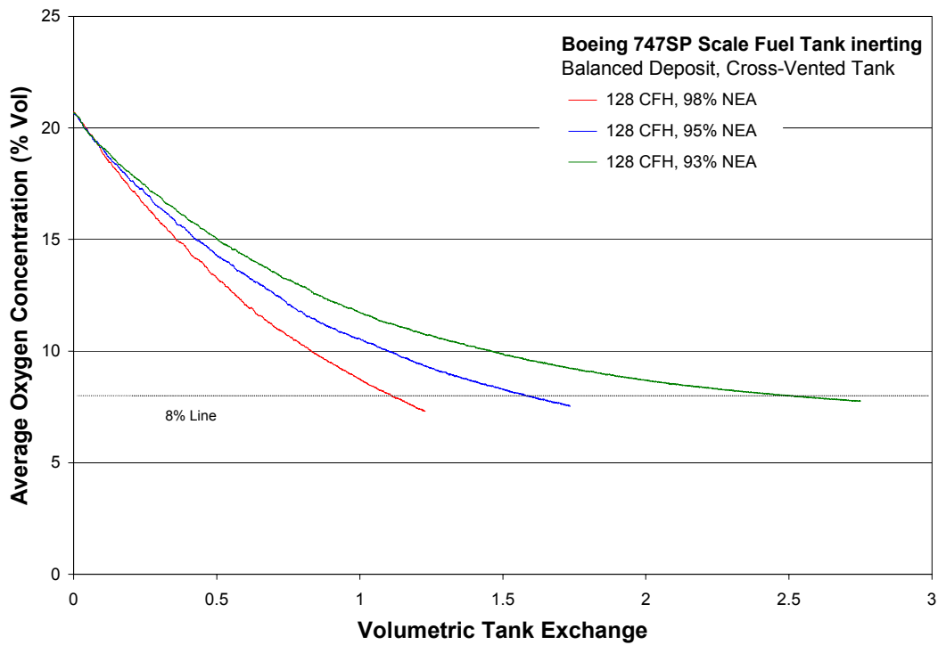
FIGURE 9. WEIGHTED AVERAGE TANK OXYGEN CONCENTRATION DATA FOR THE BALANCED DEPOSIT METHOD FOR 93%, 95%, AND 98% NEA
