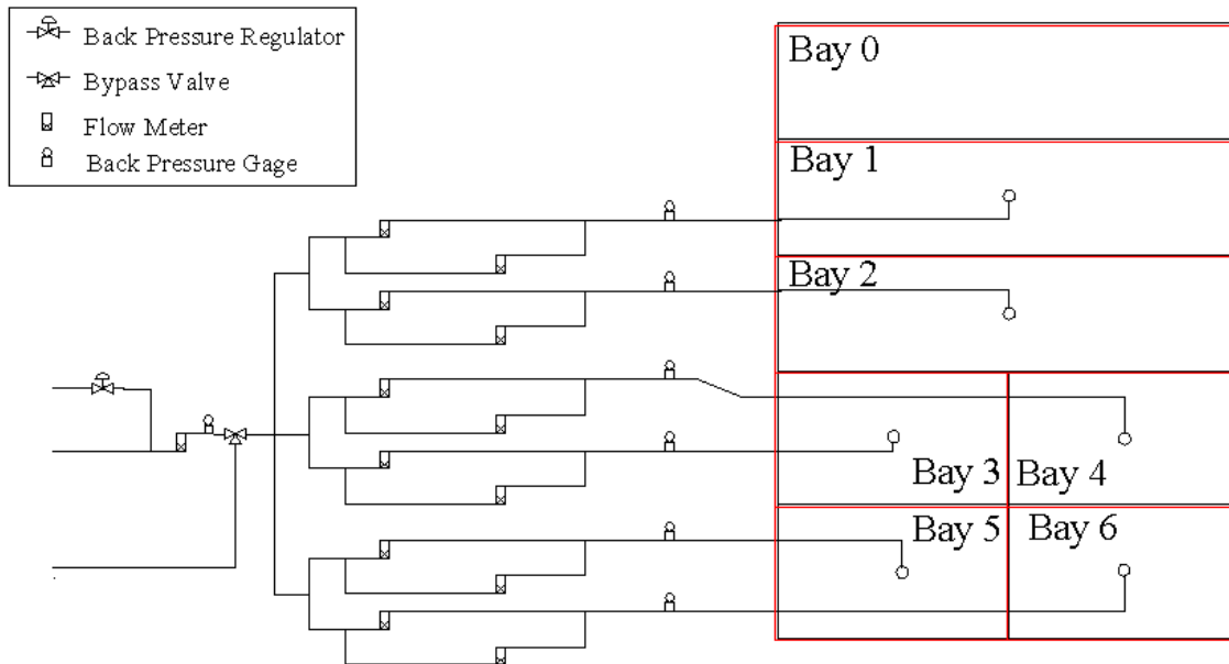
FIGURE 6. BLOCK DIAGRAM OF NEA DEPOSIT MANIFOLD
