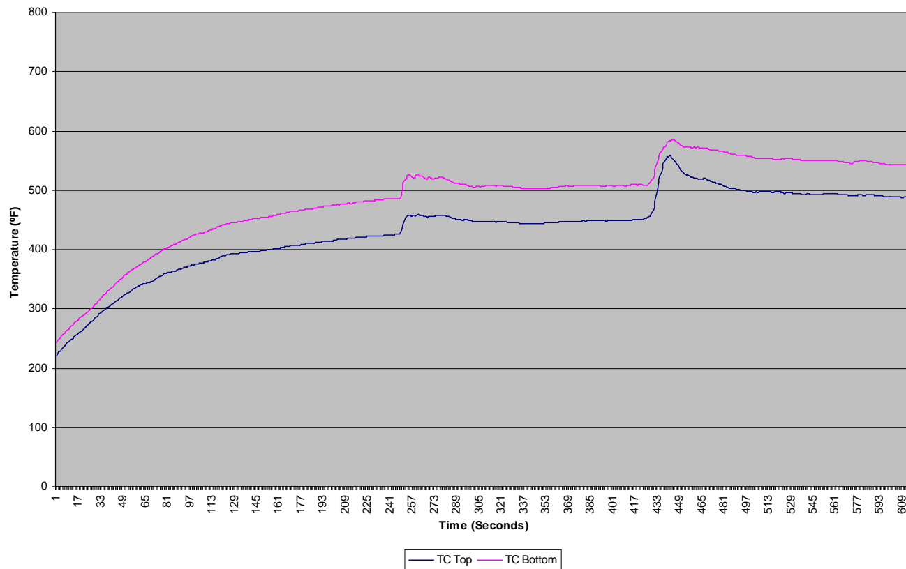
Test 86: Sanyo High Capacity, 50% Charge, Oven/Box Test
