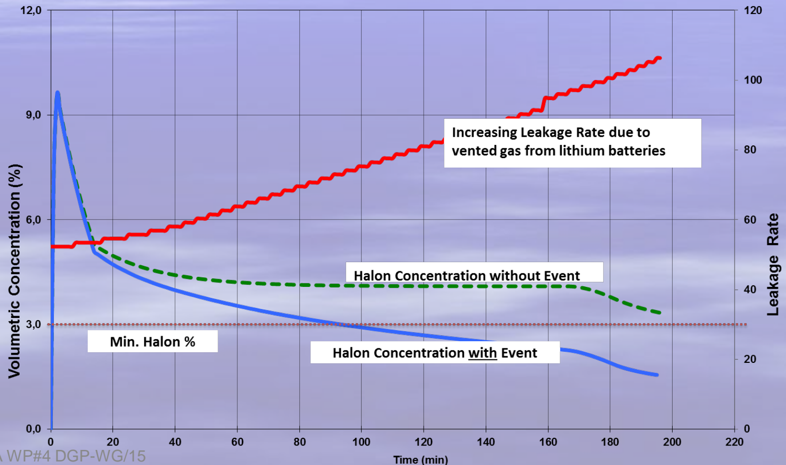
Simulation of Increasing Leakage/Decreasing Halon% due to LiBa Fire Propagation
