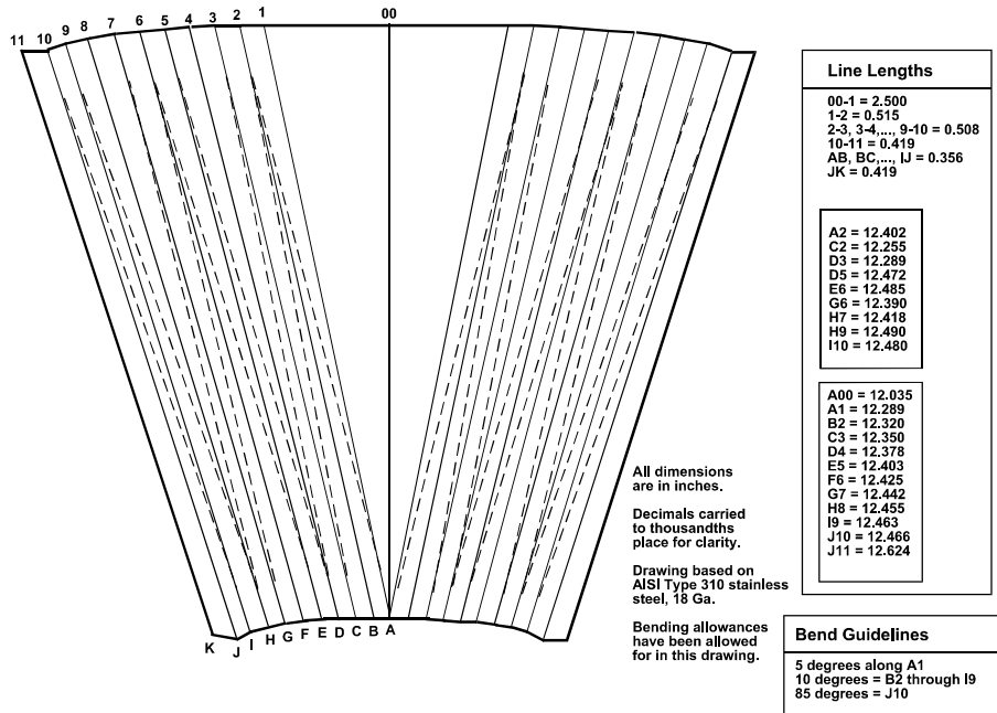
Figure 7-3a. Burner Cone Layout and Bending Pattern
