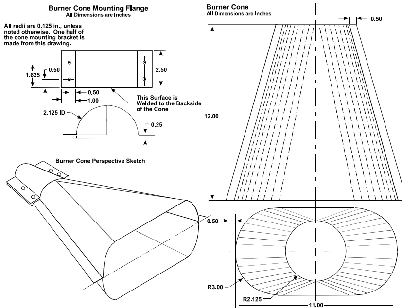
Figure 7-3b. Burner and Cone Details
