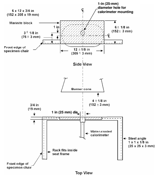
Figure 7-5. Top and Side Views of Calorimeter Bracket
