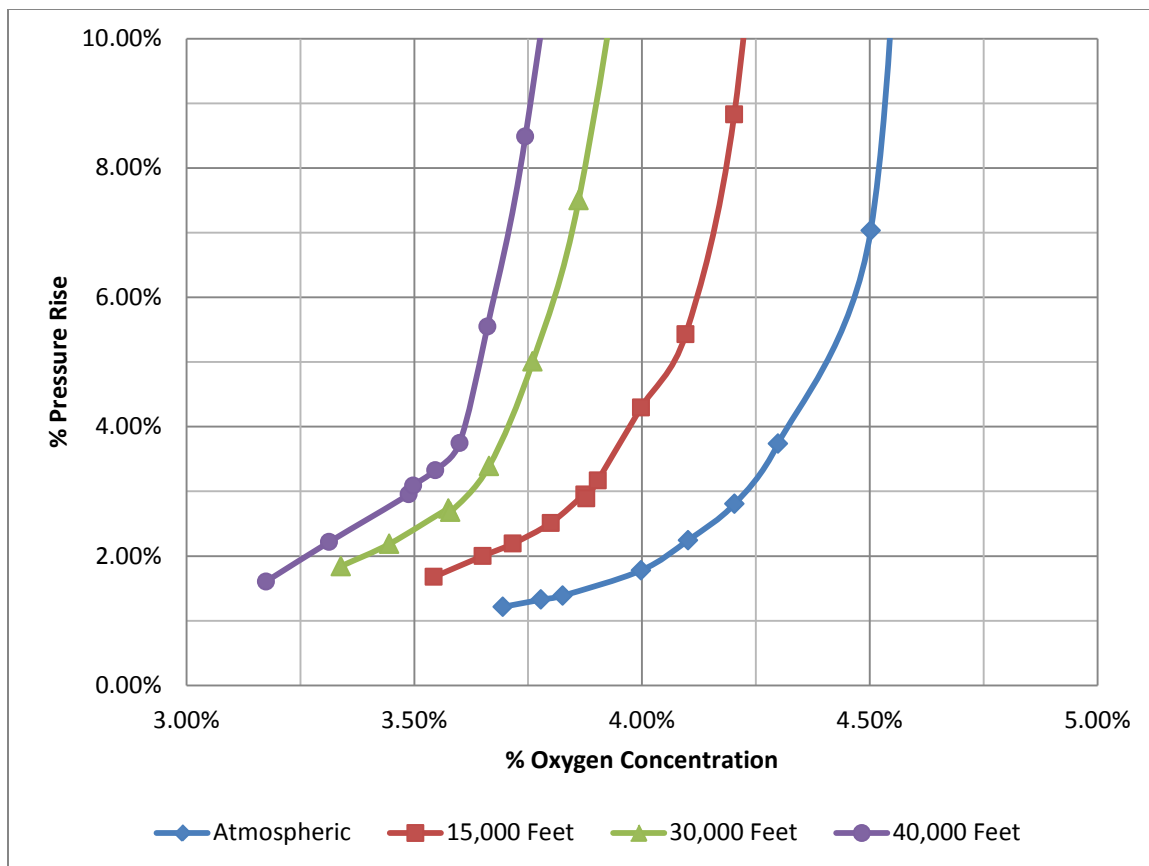
Figure 3.13: Explosion pressure data near the limiting oxygen concentration of hydrogen. Each point shows the peak pressure rise of a single test as a percentage of the initial pressure. A 3% pressure rise or more is considered flammable.
