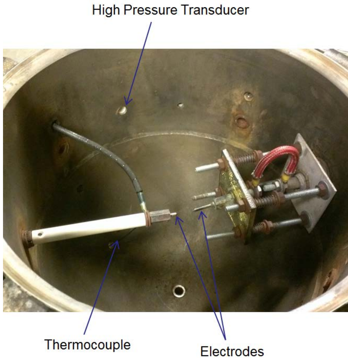
Figure 2.3: Picture of inside of combustion chamber. Shown in this picture are the fixed and movable electrodes, thermocouple, and the position of the high pressure transducer.
